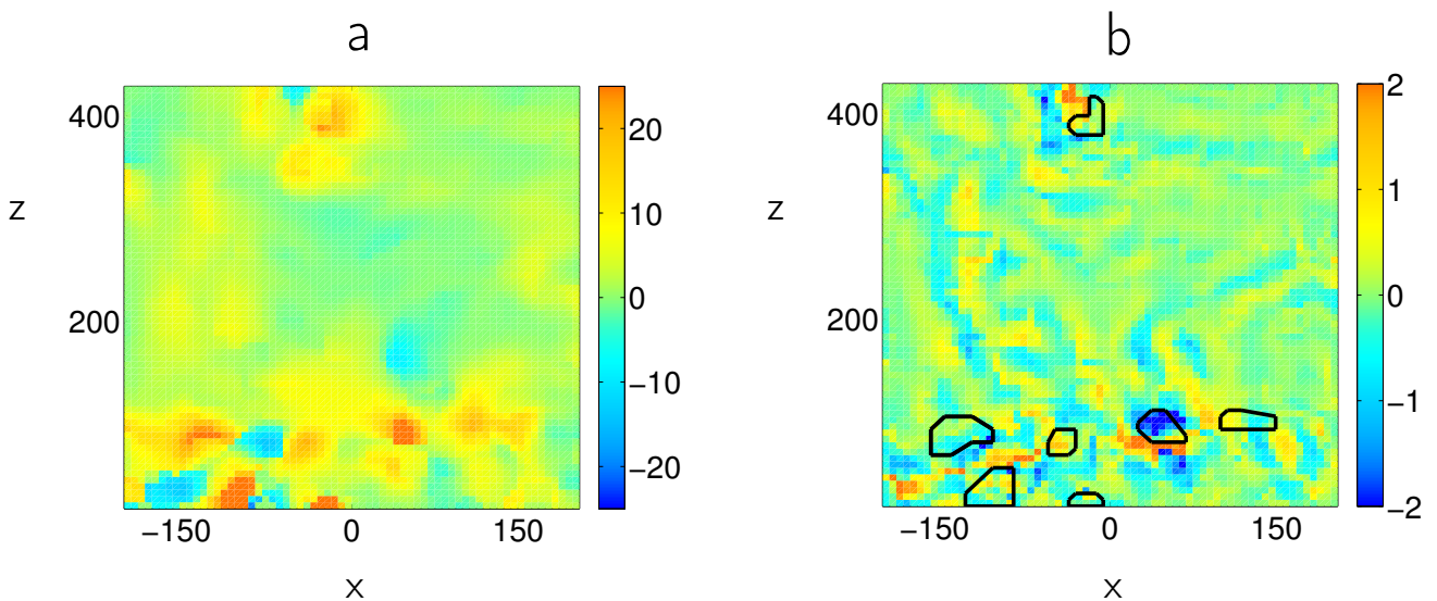
FIG. 7: Comparison between the Duchon-Robert (DR) and Eyink criteria using SPIV data. (a) map of the DR energy transfers \mathcal{D}_\ell and (b) map of the velocity circulation production \frac{d}{dt}\Gamma_\ell(\mathbf{u}) (normalized by their space-time averages) at the smallest resolution scale accessible. The results are displayed in the plane y = 0 orthogonal to the streamwise direction, and for the same data as in Fig. 2. For easier comparison, we have reported on the circulation map the contours of the areas where the DR dissipation is larger than 15 times its space-time average. We observe intense events in both maps.
