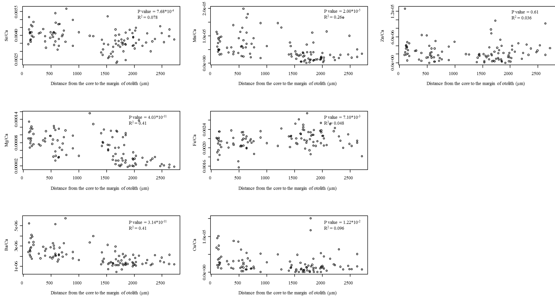
Figure 2c: relationship between element ratio and the distance along the posterior otolith axis of H. lanceolatus , P value (p) of the linear model and the Spearman correlation (R 2 ) are indicated.
