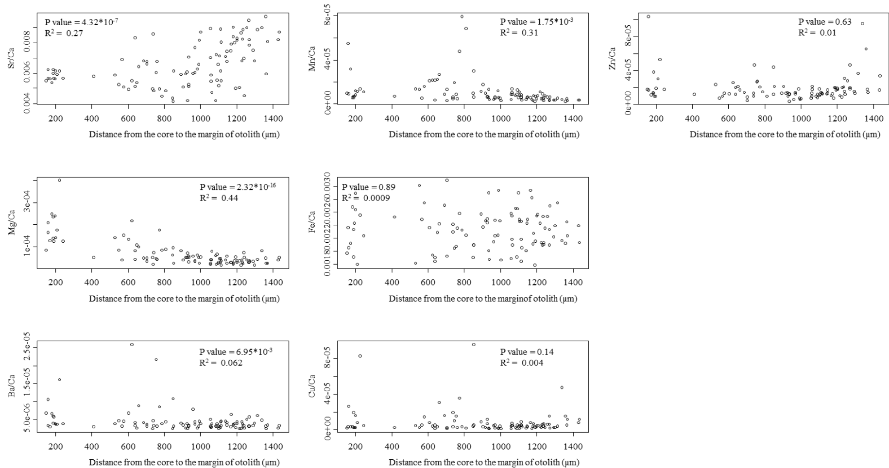
Figure 2b: relationship between element ratio and the distance along the posterior otolith axis of G. semisquamatus , P value (p) of the linear model and the Spearman correlation ( R^2 ) are indicated.
