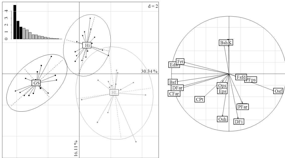
Figure 7: Functional differences linked to locomotion and food acquisition functions between the three sandeel species captured at the same date (May) at Lannion Bay, in a principal component analysis (PCA) (n = 44).
