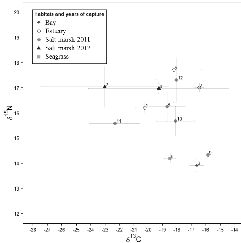
Figure 2: \delta^{13}\text{C} and \delta^{15}\text{N} (mean \pm sd) signatures of Dicentrarchus labrax muscles distinguished according to locations, habitat types and years: 1 - Loire Estuary; 2 - Lessay 2012; 3 - Bay MSMB; 4 - Rance 2012; 5 - Rance estuary; 6 - Dinan Anse; 7 - Trieux estuary; 8 - Arguenon; 9 - MSMB, 10 - St Briec; 11 - Lessay 2011; 12 - Rance 2011.
