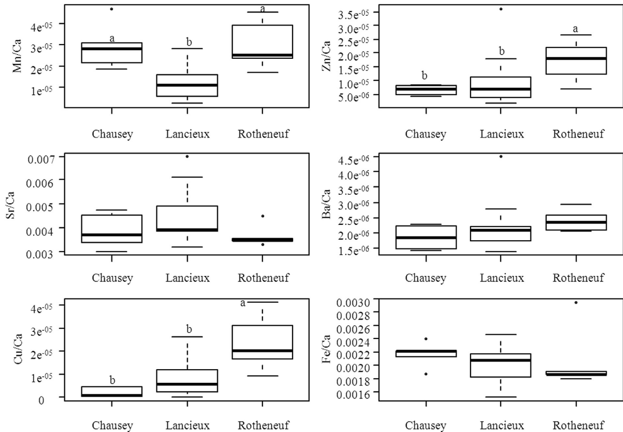
Fig. 7. Boxplots comparing different element ratios from Small Sandeels otoliths from the three sites of capture. Element ratios are inferred from the external zone of the otoliths (capture fingerprint) of Lancieux ( n = 24 ), Chausey ( n = 5 ), and Rotheneuf ( n = 5 ). Letters in superscript indicate significant differences (MANOVA, p < 0.05 ) between sites, when present.
