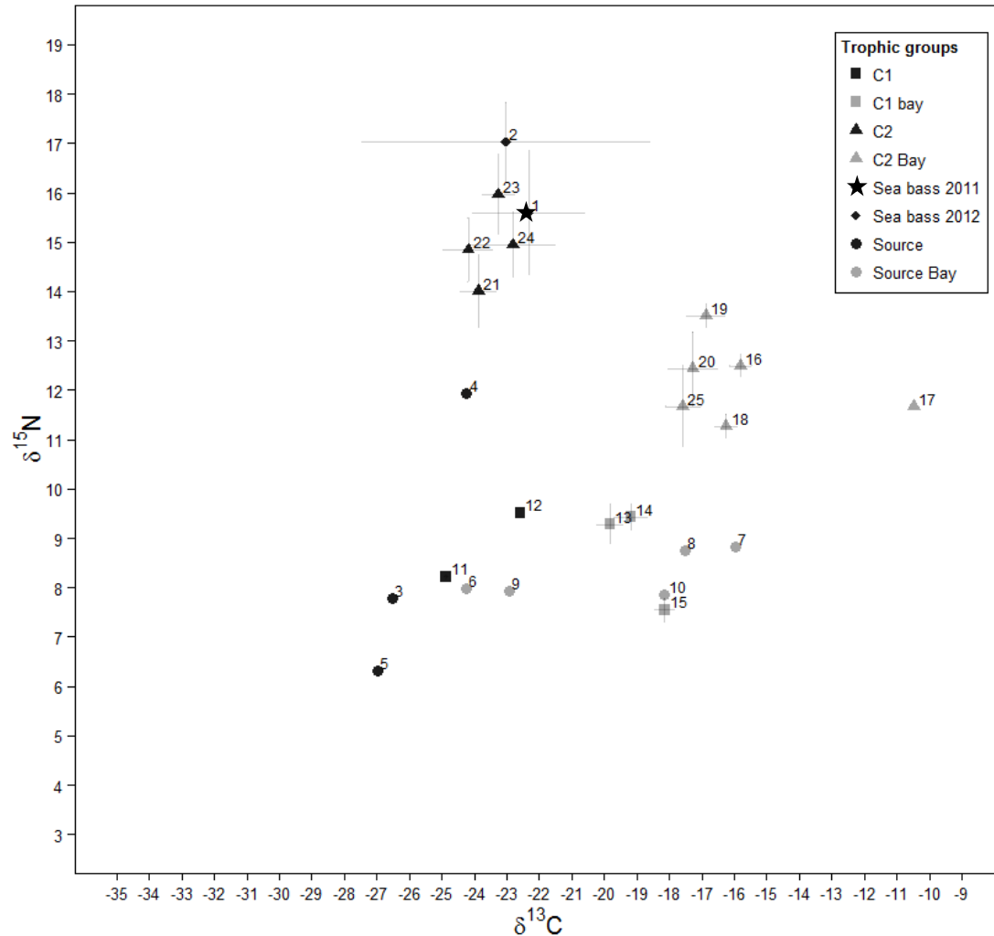
Figure 3: Isotope signatures of the food web of Lessay (mean and standard deviation). Black symbols corresponded to salt marshes organisms and grey symbols to organisms collected in the bay (i.e. outside of the salt marshes). The trophic groups represent sources, primer consumers (C1) and secondary consumers (C2). 1 - D. labrax 2011; 2 - D. labrax 2012; 3 - S. maritima , 4 - A. portulacoides , 5 - E. maritima ; 6 - Calliblepharis ciliata ; 7 - Fucus serratus ; 8 - Ascophyllum nodosum ; 9 - Chondrus crispus ; 10 - Halopitys incurva ; 11 - Gammaridae ; 12 - Sphaeromatidae ; 13 - Crassostrea gigas ; 14 - M. edulis ; 15 - Cerastoderma edule ; 16 - Nephtys sp ; 17 - Leptosynapta inhaerans ; 18 - Paraonidae ; 19 - Lumbrineridae ; 20 - Nemerthe sp ; 21 - C. maenas (salt marsh); 22 - Palaemons elegans ; 23 - Pomatoschistus microps ; 24 - C. crangon ; 25 - C. maenas (bay).
