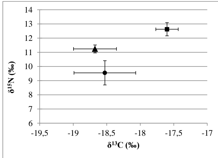
Figure 6: δ 13 C (‰) and δ 15 N (‰) muscle stable isotopic values for the three sandeels in May at Lannion (n = 15, for each species). Square: H. lanceolatus , triangle: G. semisquamatus , circle: H. immaculatus .
