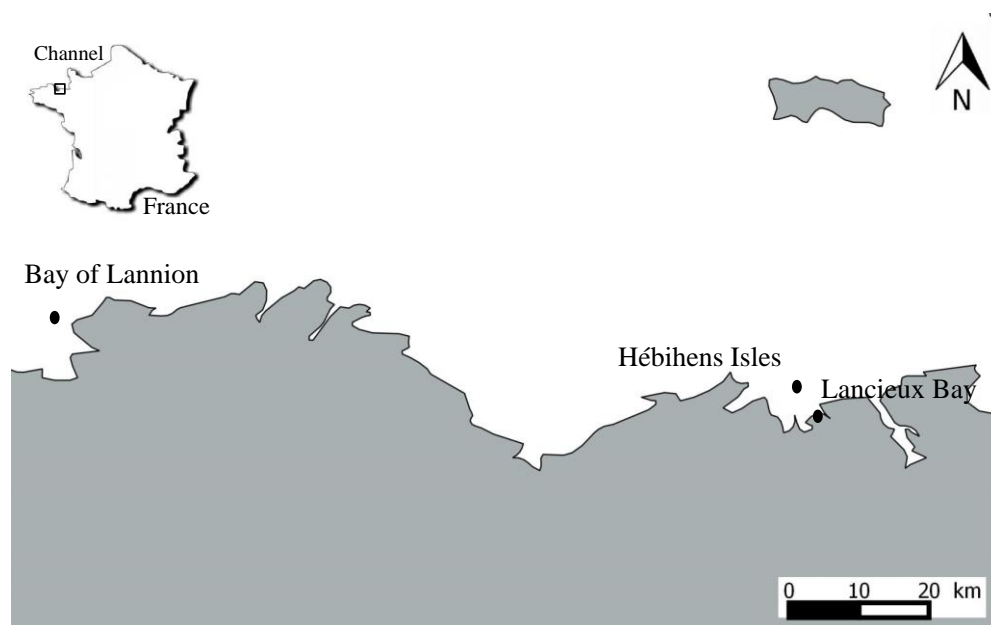
Figure 1: Location of the three sampling sites of sandeels in the Norman-Breton Gulf (south-western English Channel). The three species were captured in subtidal sandbanks in the Bay of Lannion. For the spatial analysis, H. lanceolatus was also captured in Hébihens Isles (subtidal sandbanks) and in intertidal sandbanks at Lancieux Bay.
