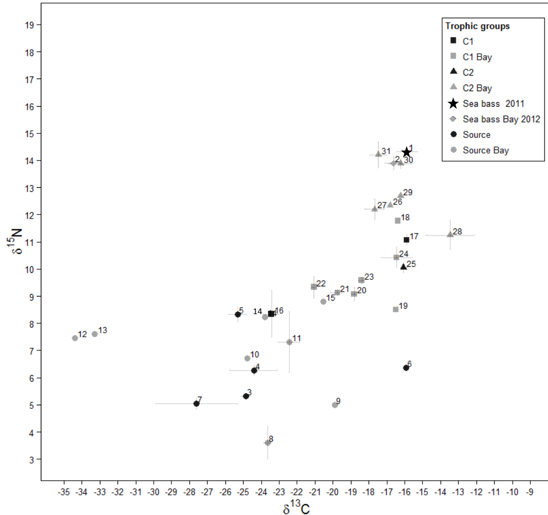
Figure 4: Isotope signatures of the food web of MSMB (mean and standard deviation). Black symbols corresponded to salt marsh organisms and grey symbols to organisms collected in the bay (i.e. outside of the salt marshes). The trophic groups represent sources, primer consumers (C1) and secondary consumers (C2). 1 - D. labrax 2011; 2 - D. labrax 2012 Bay; 3 - E. maritima ; 4 - P. maritima ; 5 - A. portulacoides ; 6 - microphytobenthos; 7 - river POM; 8 - marine POM; 9 - phytoplankton Bay; 10 - Taonia sp. ; 11 - Ceramium sp. ; 12 - Plocamium sp. ; 13 - S. coronopifolius ; 14 - Calliblepharis ciliata ; 15 - Solieria chordalis ; 16 - Amphipoda ( Orchestia gammarellus ); 17 - Mysidaceae (salt marsh); 18 - Mysidaceae (bay); 19 - Albra albra ; 20 - Crepidula fornicata ; 21 - M. edulis ; 22 - Crassostrea gigas ; 23 - Cerastoderma edule ; 24 - Arenicola arenicola ; 25 - H. diversicolor ; 26 - Nephtys sp. ; 27 - Palaemon serratus ; 28 - C. crangon ; 29 - C. maenas ; 30 - Pomatoschistus sp. , 31 - Loligo sp.
