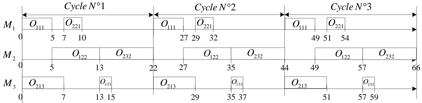
Figure III. 18: Allocation des machines sans contraintes de maintenance
