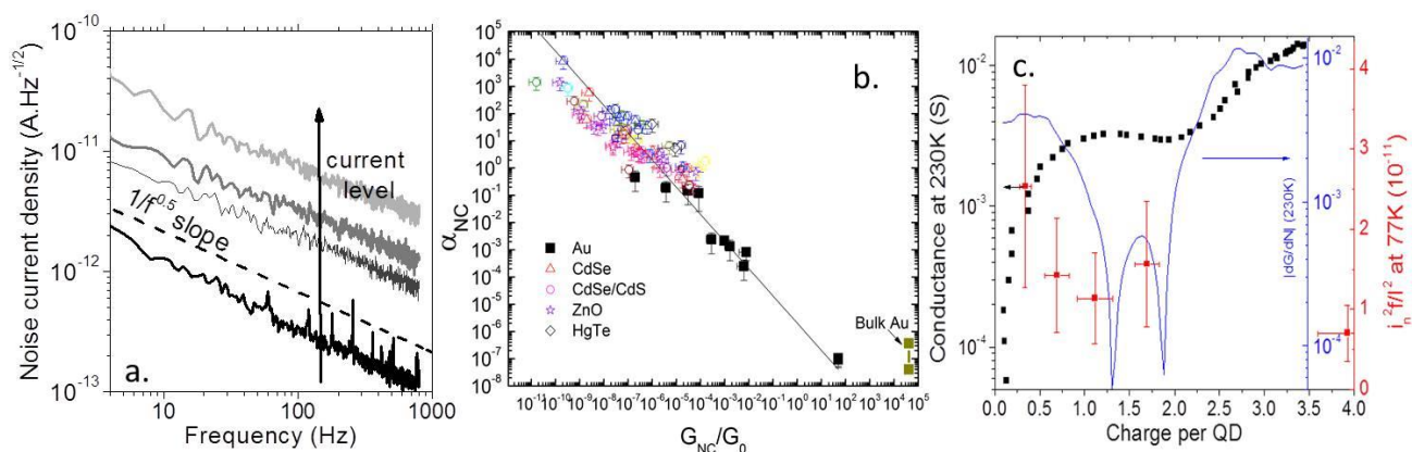
Figure 16 a. Noise current density as a function of signal frequency for CdSe NPL film under different biases. b. Hoope constant normalized by the number of nanocrystals as a function of the interparticle conductance for a broad range of material and nanoparticle sizes. Conductance, transconductance and noise intensity as a function of the CQD carrier density, from ref 18.
