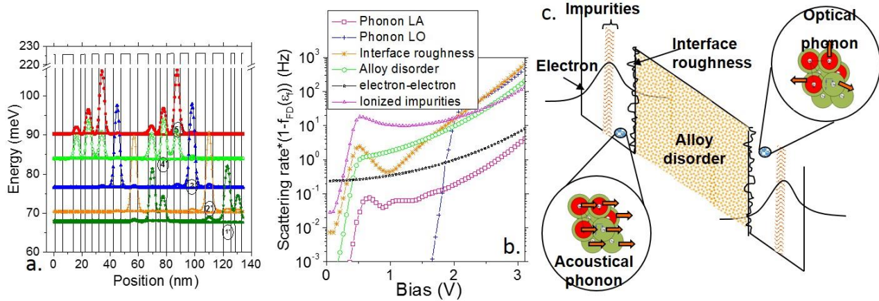
Figure 2 a. Band structure and wavefunction of a THz quantum cascade detector, as proposed in ref 3. b. Scattering rates resulting from different scattering processes as a function of the applied bias for the 15 \mu m QWIP structure, as investigated in ref 4. c. Different scattering mechanisms considered in the modelling tools developed in ref 3-5, 7.
