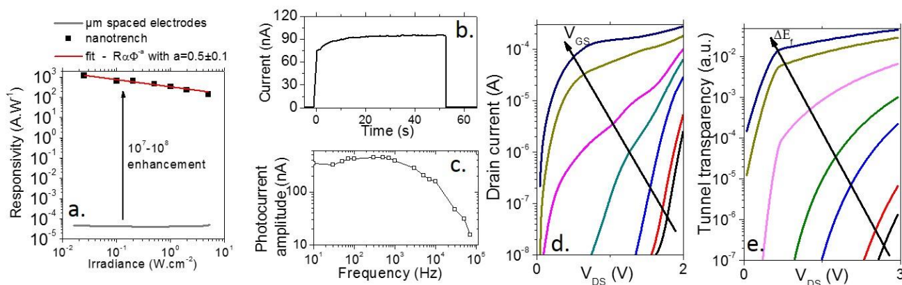
Figure 24 a. Photoresponse as a function of the photon irradiance ( \lambda=405\text{nm} ) for a film of CdSe/CdS NPL deposited on 10\mu\text{m} spaced electrodes or on a nanotrench. b current in a CdSe/CdS NPL film deposited on a nanotrench under a pulse of light. c. Frequency dependence of the photocurrent for a CdSe/CdS NPL film deposited on a nanotrench. The cut-off frequency is around 3 kHz. d IV curves under different gate biases for a CdSe/CdS NPL film deposited on a nanotrench. e. Tunnel transparency relative to the injected contact as a function of the drain bias for different gate biases for a CdSe/CdS NPL film deposited on a nanotrench.
