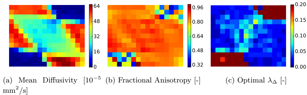
Figure 5.3: The estimated Mean Diffusivity (MD), Fractional Anisotropy (FA) and optimal regularization weight for the physical phantom. It can be seen that white MD differs for different fiber configurations, the FA is consistent in fibrous areas. The optimal regularization weight using GCV also shows similar values in fibrous areas, but much higher in the empty areas.
