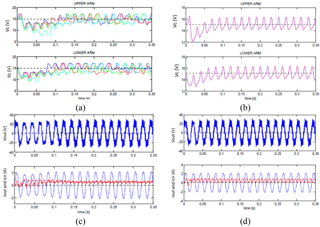
Fig. 2.25.: Simulation results of (provided by a trainee of master degree who was supervised by the author of this manuscript [Yaf]):
