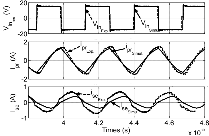
Fig. 3.19.: Validation results for a power transmission function ( ep_1 = 1mm ): the comparison of V_{in,power} , i_{pr} and i_{se} between the simulation and the experimental results
