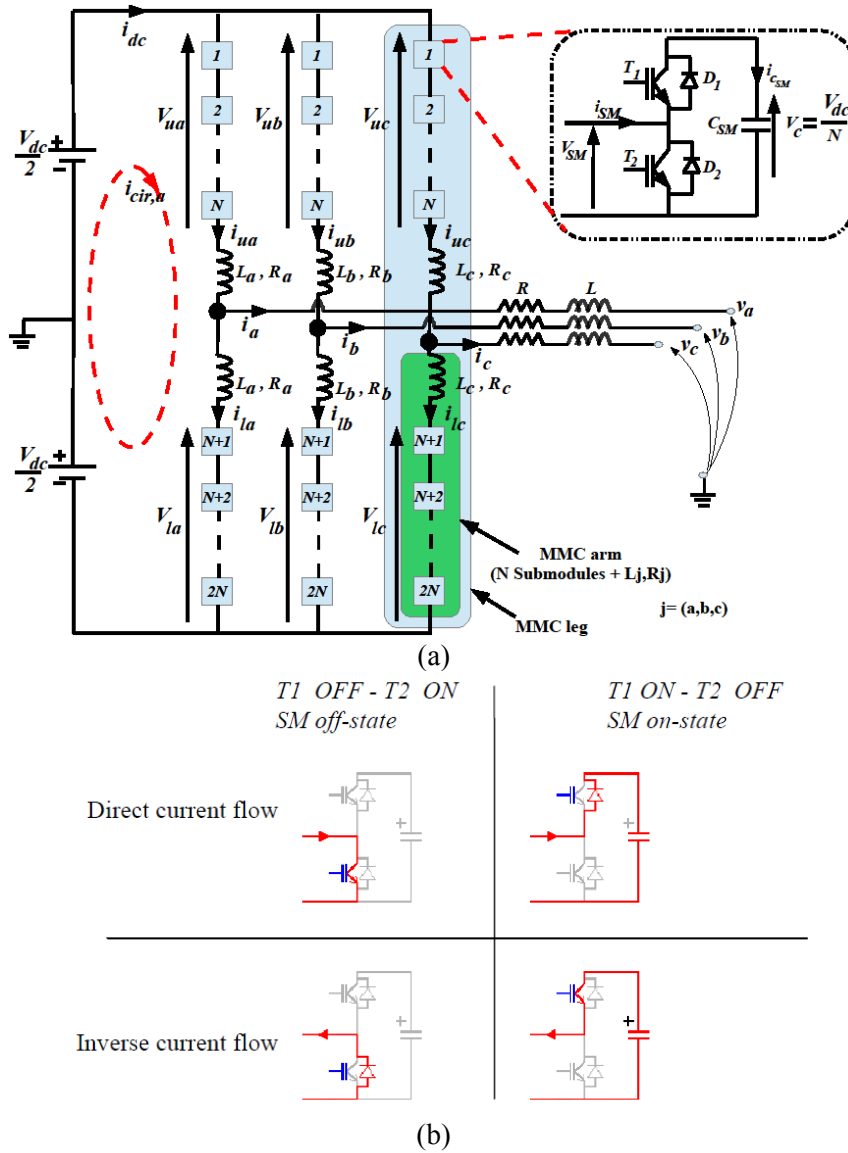
Fig. 1.15: MMC topology descriptions:
