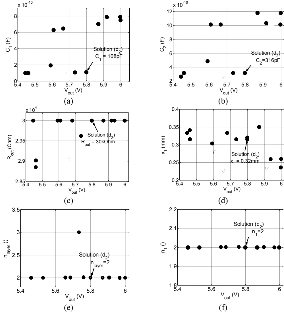
Fig. 2.13.: Evolution of the variables as a function of the output voltage V_{\text{out}}
