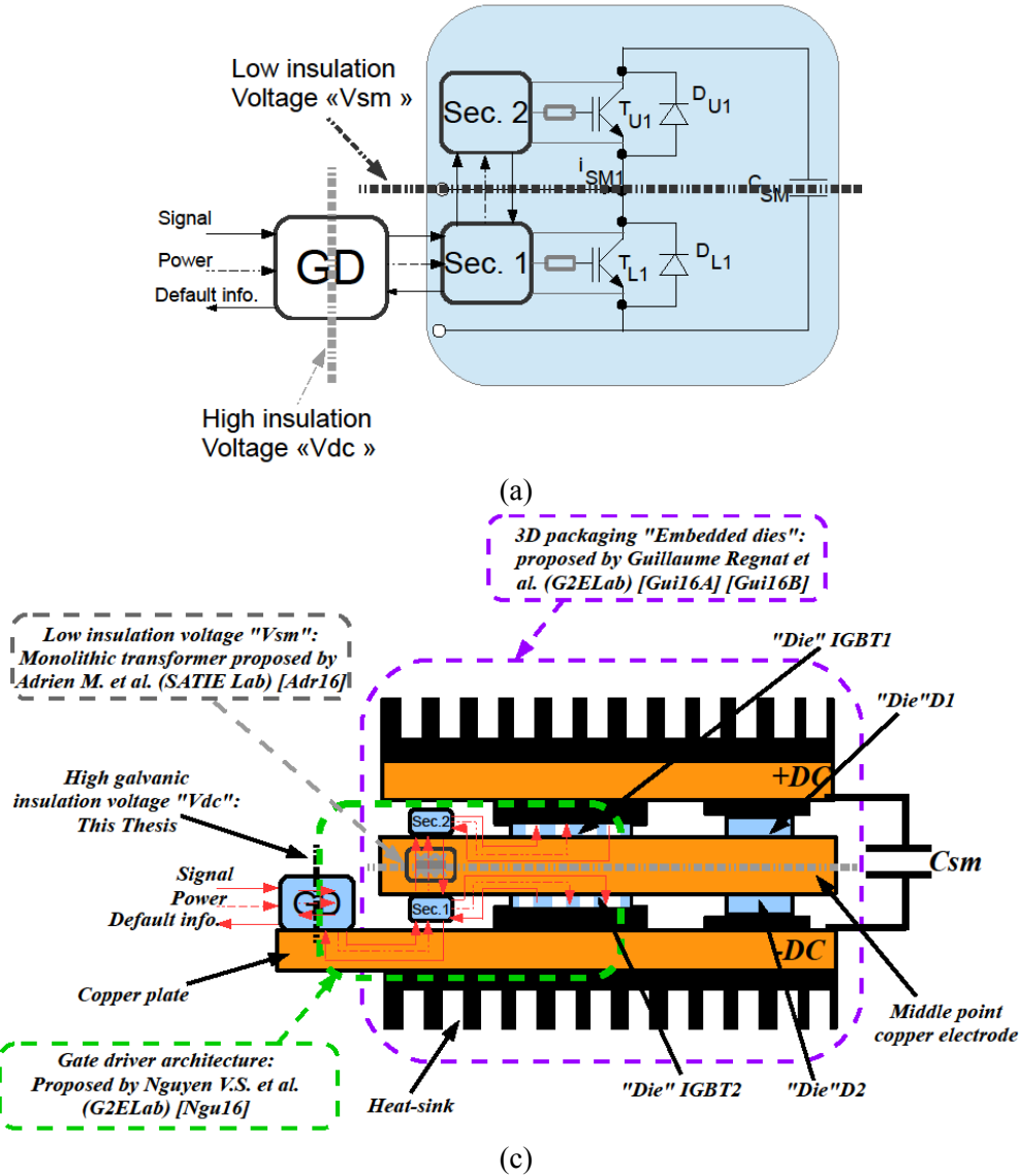
Fig. 3.23: 3D packaging of active power modules for SM:
