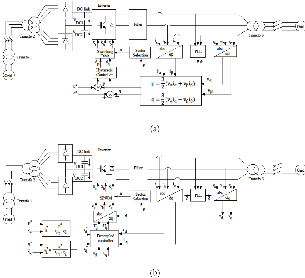
Fig. 1.5: Example of the proposed control design for 3L-NPC converter:
