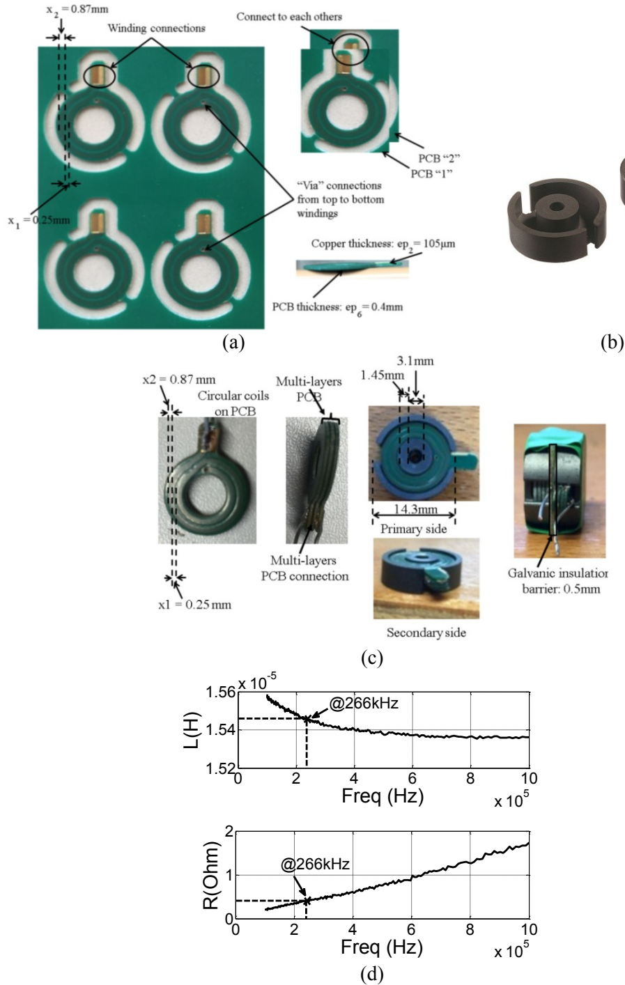
Fig. 3.2.: Optimal pot core planar transformer set up:
