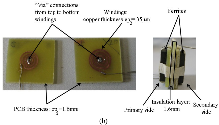
Fig. 3.9.: Procedure of optimal transformer fabrications for two different ferrite cores: (a) Pot core multi-layer planar transformer, (b) Double-layer planar transformer.
