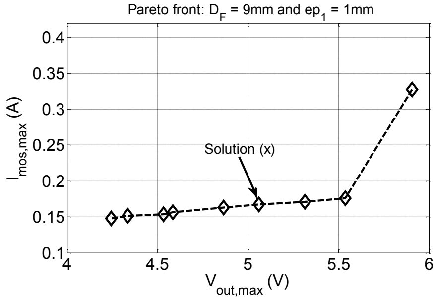
Fig. 3.20.: Pareto front for a signal transmission function with ep_1 = 1\text{mm} .
