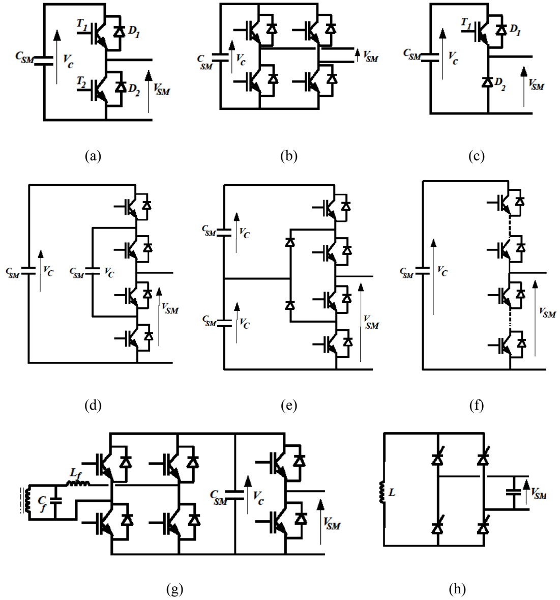
Fig. 1.13: Various sub-module topologies for MMC converter:
