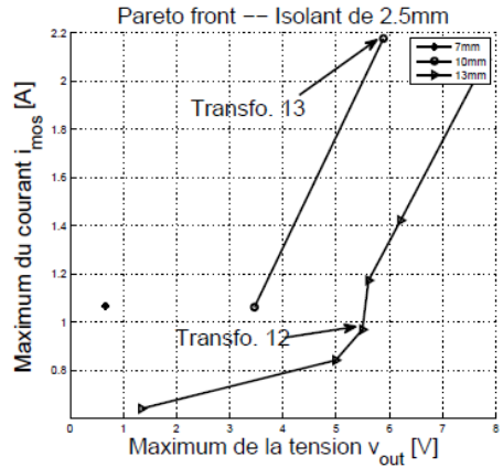
c. PCB Insulation layer 2.5 mm
