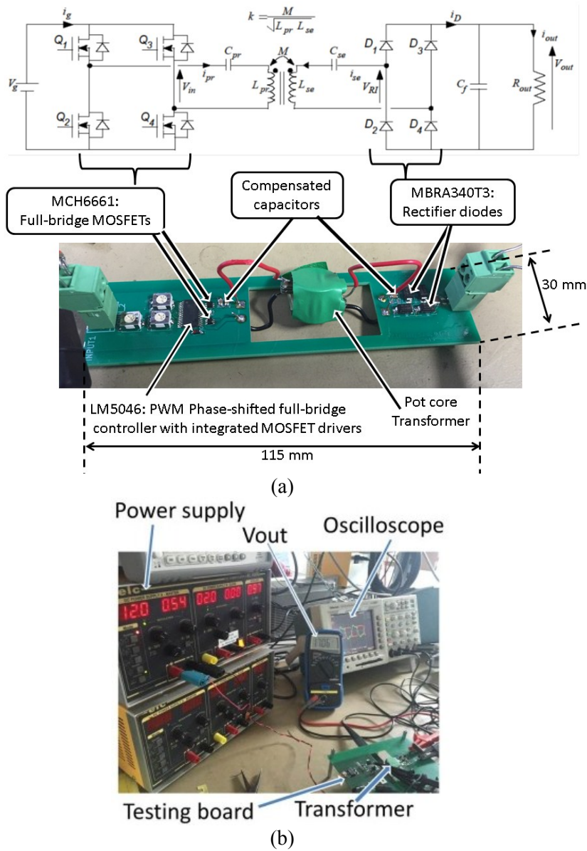
Fig. 3.3: A testing board: (a) An optimal prototyped board, (b) Physical prototype instruments.
