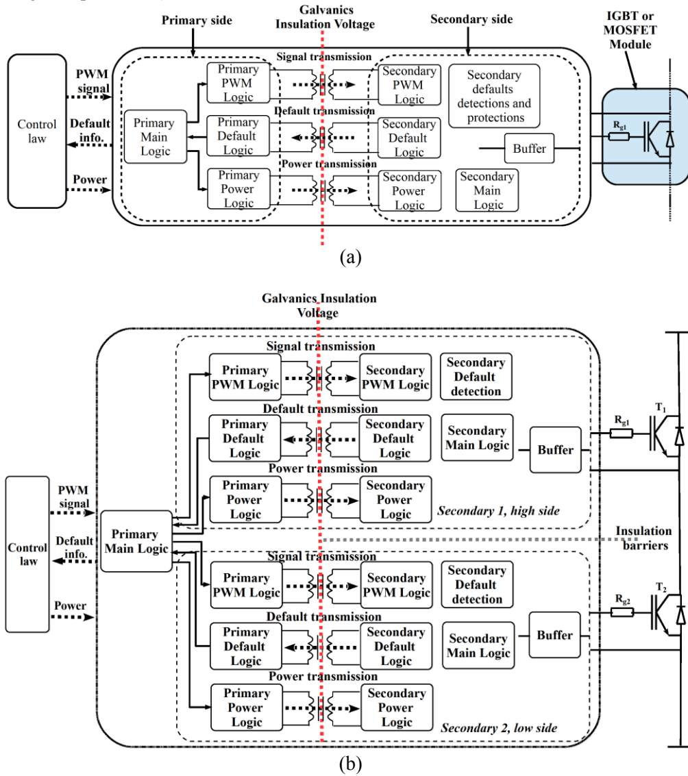
Fig. 2.1.: Synopsis of: (a) a single channel IGBT gate driver, (b) a dual channel IGBT gate driver.
