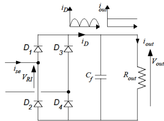
Fig. 2.16.: Description of insulated DC-DC resonant converter topologies:
