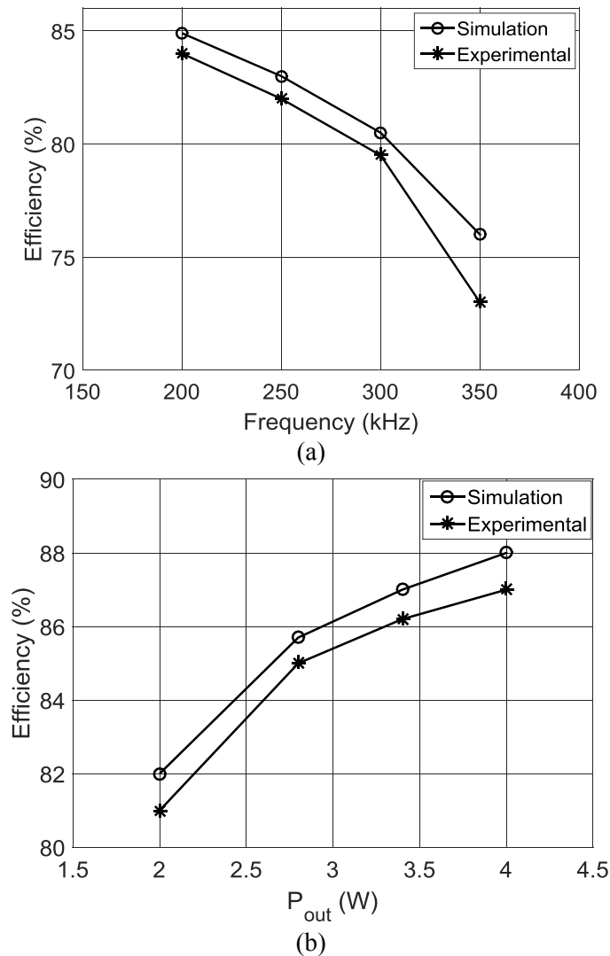
Fig. 3.5.: More validation results for a power transmission function:
