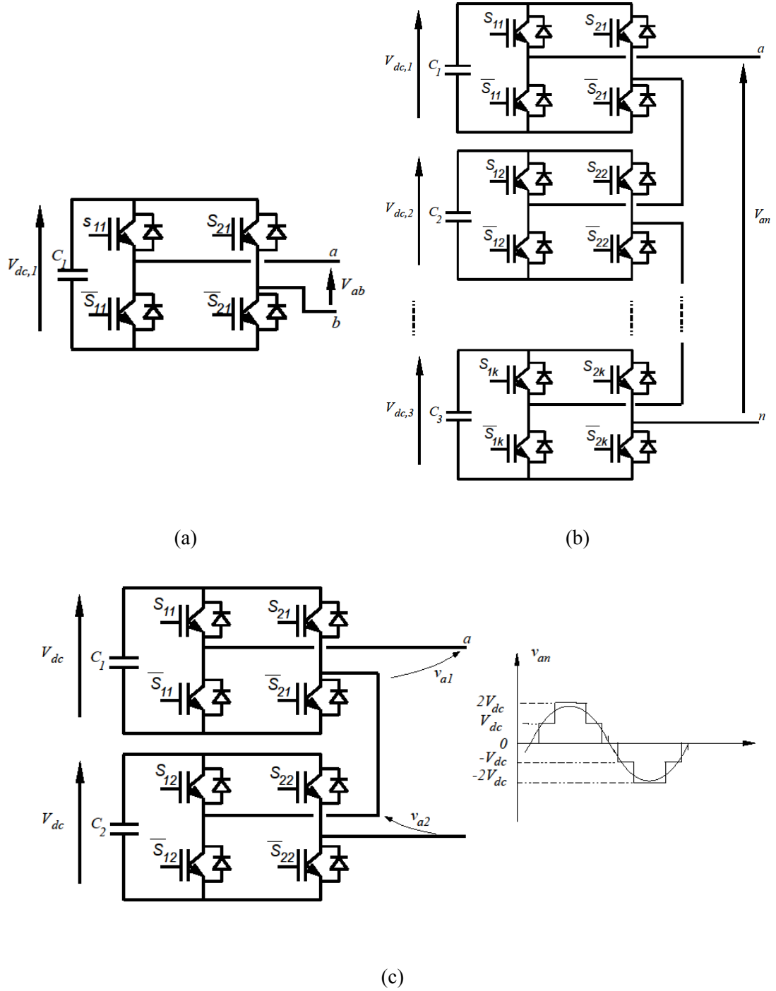
Fig. 1.9: Cascaded H-bridge (CHB) multilevel converter description:
