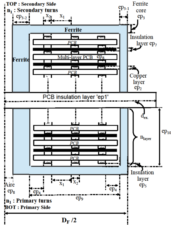
Fig. 2.19.: Multi-layer pot core transformer 2D description (re-call of Fig. 2.9).
