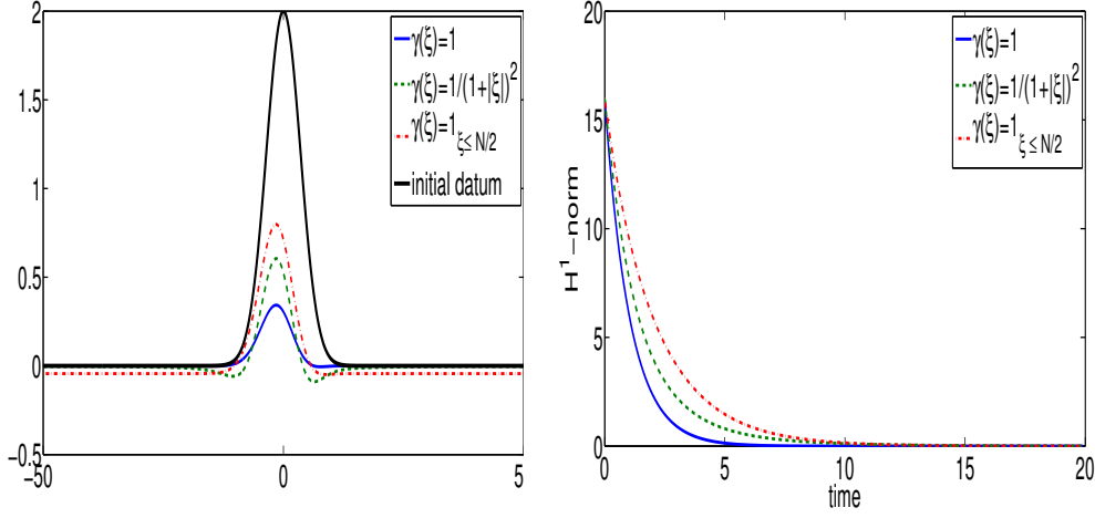
Figure 2.1: On the left, solution of the damped equation with \gamma(\xi) = 1 (—), \gamma(\xi) = 1/(1 + |\xi|)^2 (- -) and \gamma(\xi) = \mathbb{I}_{\xi \leq N/2} (· · ·) starting from the same initial datum (—) at time t = 20 . On the right, decay of the H^1 -norm with respect to time.
