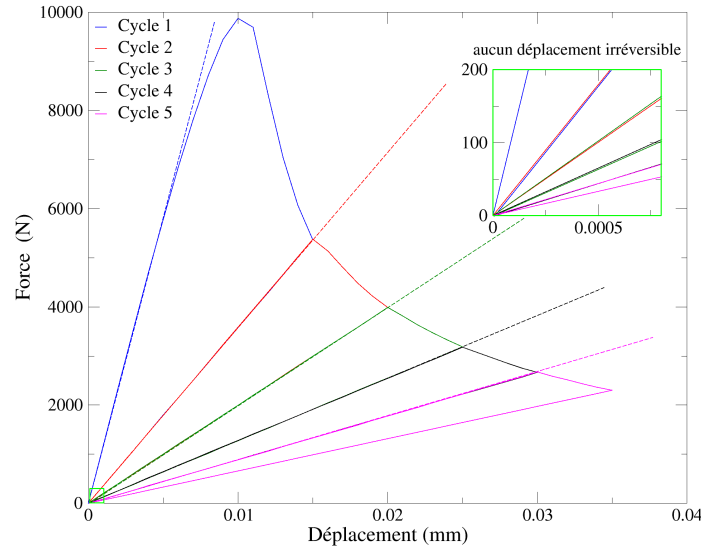
FIGURE 2.24 – Cycles charge-endommagement-propagation-décharge
