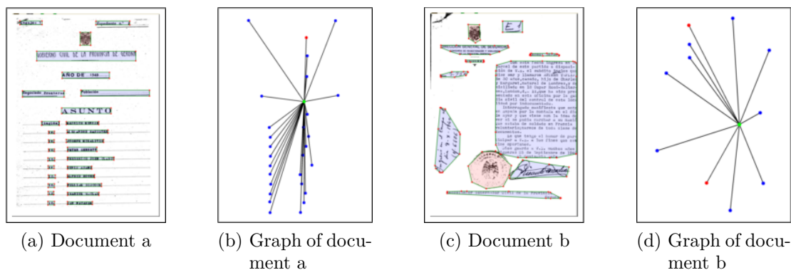
Figure 3.2.2: The graphs produced by the descriptor of Gordo and Valveny. Image reproduced from [GV09].
