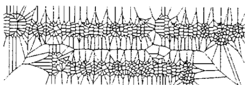
(c) Full Voronoi diagram
