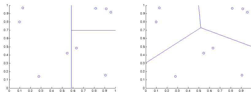
(a) Non optimal/unbalanced clustering result.
