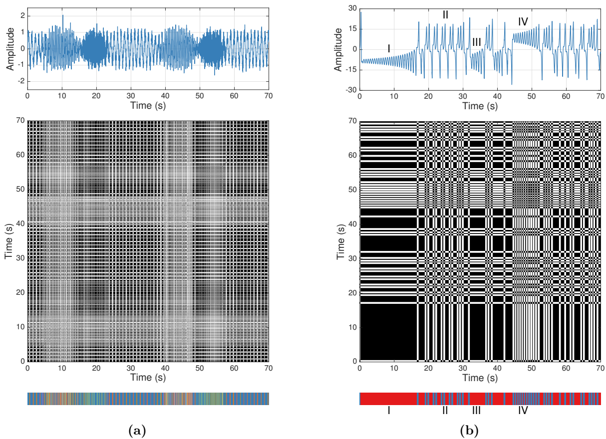
Fig. 2.15: The SRSA results for the synthetic data obtained with delay embeddings. (a) Transient oscillations, reconstruction parameters: m = 5 , \tau = 0.1 s; (b) Solutions of the Lorenz system, reconstruction parameters: m = 3 , \tau = 0.18 s.
