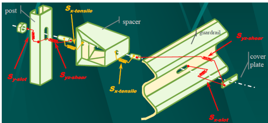
Figure 1- 15 Multi-body Models of Bolted Connections of safety barrier [14]
