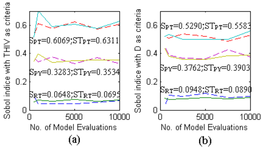
Figure 3- 33 Evolution of Sobol' indices against sample data size: (a) THIV as criteria (b) D as criteria (Solid line: total effects of PT ( ST_{PT} ), PY ( ST_{PY} ) and RT ( ST_{RT} ); Dotted line: main effects of PT ( S_{PT} ), PY ( S_{PY} ), RT ( S_{RT} ))
