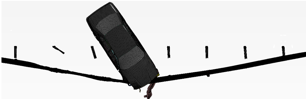
Figure 4- 3 Failure of vehicle redirection when H and E decrease greatly
