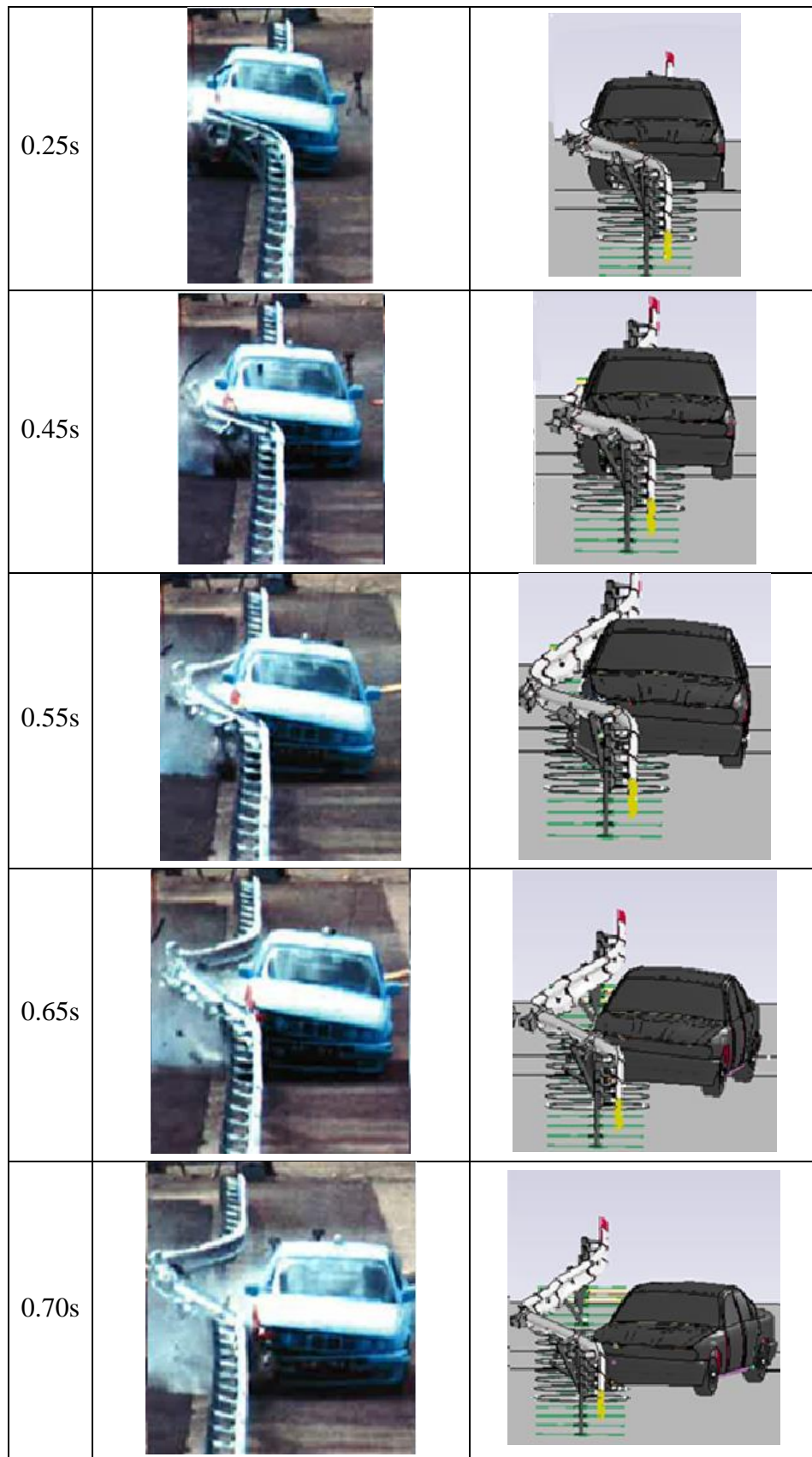
Figure 3- 25 VRS crash test &amp; simulation visual comparison
