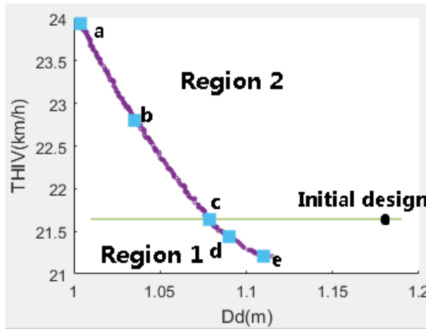
Figure 4- 5 Pareto efficient solution of VRS MONO
