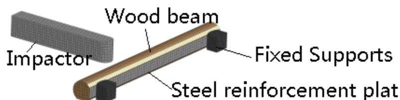
Figure 2- 8 Numerical model of the bending test [49]
