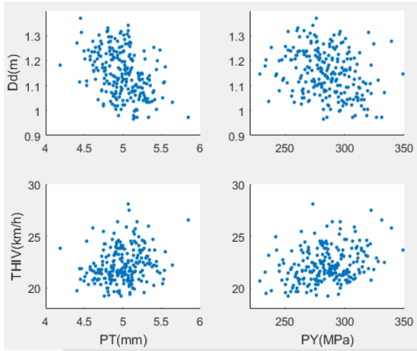
Figure 4- 4 Scatter plot of uncertain factors PT , PY and outputs THIV , D
