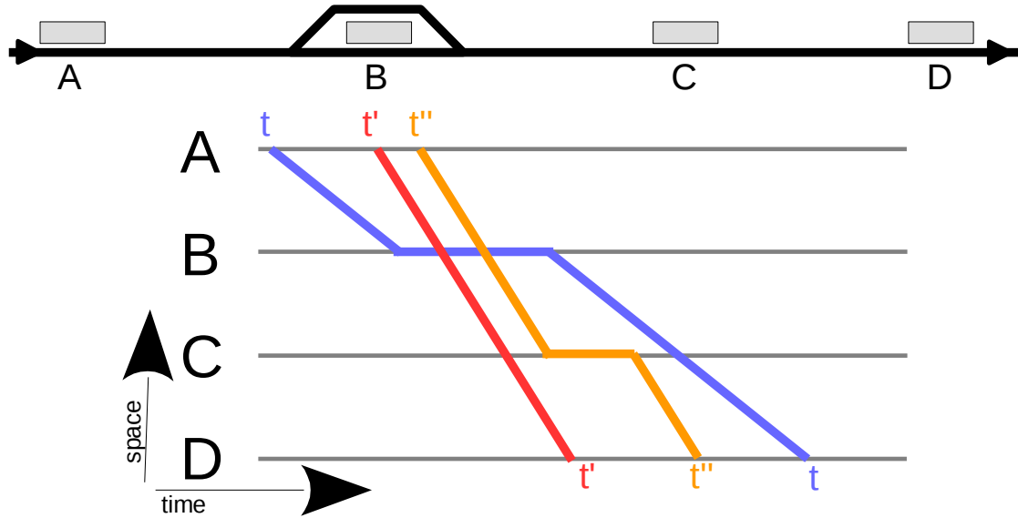
Figure 4.5: Example of circular dependency between trains. Three trains t , t' and t'' run between stations A and D. t is overtaken by t' and t'' in station B, the only available overtaking location. First, if the departure of t from A is delayed, it causes a delay on t' . Next, by delaying t' , t'' is delayed as well. Finally, because t must be overtaken by t'' in B, and t'' has a scheduled stop in C, whenever t'' is delayed it causes a delay on t .
