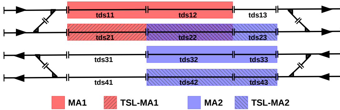
Figure 4.2: Example of two MA s affecting a set of TDS s. MA1 directly affects tds11 and tds12 , while imposing a TSL in tds21 and tds22 . MA2 directly affects tds32 and tds33 , and it imposes a TSL in two set of TDS s: First, tds22 and tds23 , and second, tds42 and tds43 .
