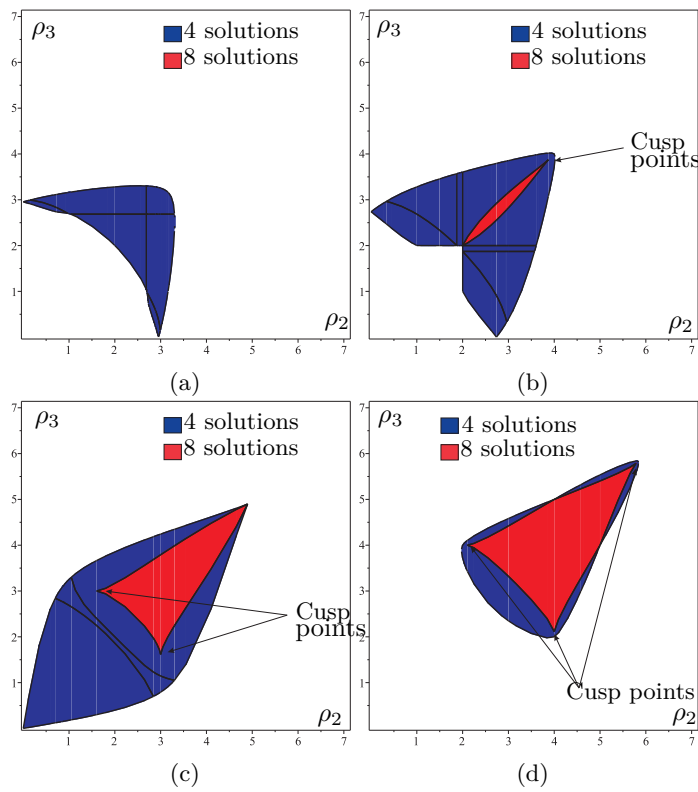
Figure II.14 – Slice of the joint space for OM^1 for \rho_1 = 1 (a), \rho_1 = 2 (b), \rho_1 = 3 (c) and \rho_1 = 4 (d) and the number of solution for DKP for k = 1
