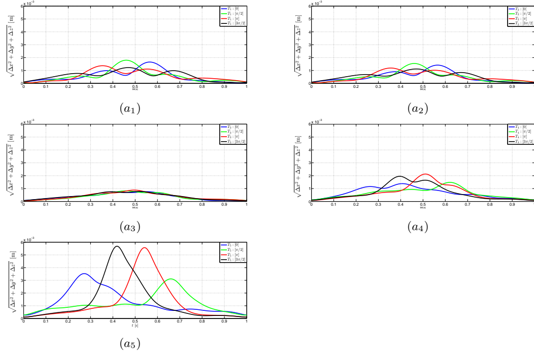
Figure V.14 – Cartesian errors, norm, along trajectories \phi_1(t) ( a_1 ), \phi_2(t) ( a_2 ), \phi_3(t) ( a_3 ), \phi_4(t) ( a_4 ) and \phi_5(t) ( a_5 ) for different starting positions [T_1 : [0] (in blue), T_2 : [\pi/2] (in green), T_3 : [\pi] (in red), T_4 : [3\pi/2] (in black)], Image of the joints errors in the workspace of the manipulator.
