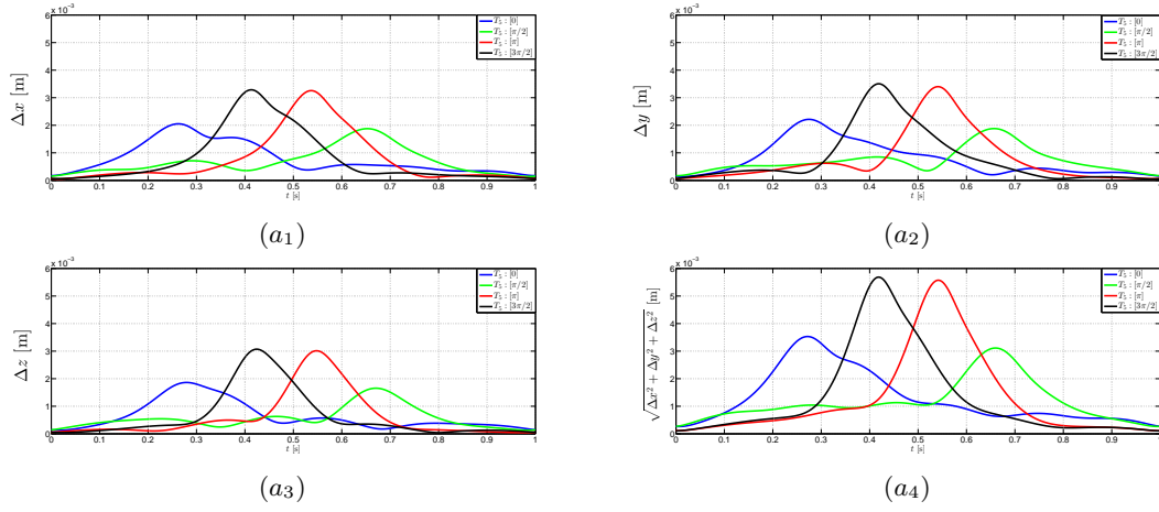
Figure V.13 – Cartesian errors in x ( a_1 ), y ( a_2 ), z ( a_3 ) and norm ( a_4 ) along the trajectories \phi_5(t) for different starting positions [T_1 : [0] (in blue), T_2 : [\pi/2] (in green), T_3 : [\pi] (in red), T_4 : [3\pi/2] (in black)], Image of the joints errors in the workspace of the manipulator.
