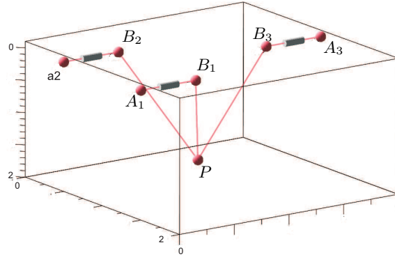
Figure II.3 – Configuration plot for Triaglide robot
