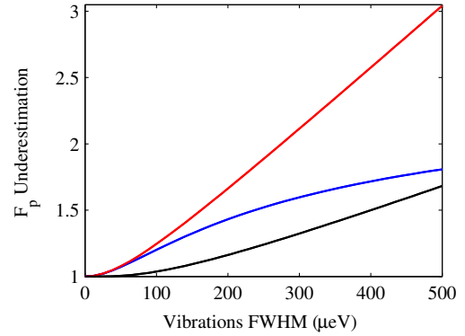
Figure C.2 – Underestimation of the Purcell factor as a function of the FWHM of the vibrations of the cavity. In red the photon count method factor V , in blue the transient method factor V_2 and in black the ratio V/V_2 .
