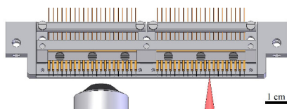
Figure 3.8 – Shooting setup : on the left a Mirau objective enables a measurement of the surface, on the right, a \text{CO}_2 laser is focused by an aspherical lens. The fibers are rowed in a metallic holder, to be shot in series. Reprinted from [149], with the author’s permission.
