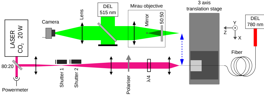
Figure 3.7 – Schema of the shooting setup : the fiber is on a translation stage, which can switch between two positions. The shooting position is in the lower part of the schema. In the upper part, a Mirau objective is present to analyze the surface of the fiber before and after the shoot. Adapted from [149], with the author’s permission.
