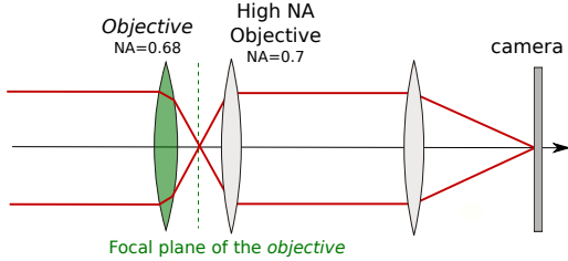
Figure B.1 – Schema of the setup with which the objective properties are evaluated : a plane wave is focused with the objective and the image plan is observed with a high numerical aperture objective.
