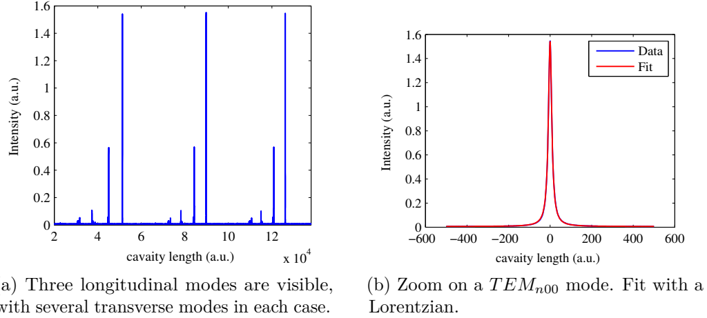
Figure 3.25 – The wavelength is fixed and the cavity length is swept fast while its output is recorded with a photodiode. The ratio of the distance between two longitudinal peaks and the width of a peak gives the finesse of the cavity.
