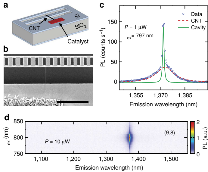
Figure 1.20 – An individual carbon nanotube coupled to a nanobeam cavity. (a) A schematic of a device. (b) Scanning electron microscope image of a device with a suspended nanotube. Scale bar is 2 μm. (c) Typical PL spectrum of an air-mode device coupled to a nanotube. The dots are data and the lines are Lorentzian fits. (d) PL excitation map of the device shown in c taken with the laser polarization perpendicular to the nanobeam. Reprinted from [32], published under the Creative Commons CC-BY licence.
