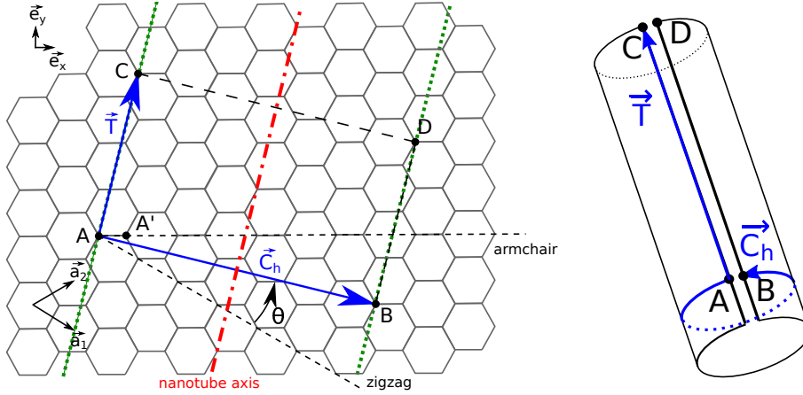
Figure 2.1 – Graphene is composed of carbon atoms organized as a 2-dimensional honeycomb lattice. Its basis vectors \vec{a}_1 and \vec{a}_2 are depicted in black. A carbon nanotube can be considered as a graphene sheet wrapped around its chiral vectors \vec{C}_h . The basis vectors of the primitive cell of a CNT are \vec{C}_h and \vec{T} , where \vec{T} is along the axis of the tube. The dashed green line depicts the full zone along which the nanotube is wrapped. All the figures in this chapter are, unless otherwise mentioned, inspired to some extent from [91, 92, 93], with the authors permission.
