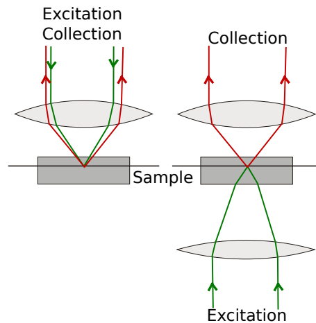
Figure 4.9 – On the left, a standard confocal setup, on the right the excitation is switch to the back.
