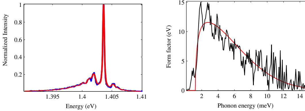
(a) Photoluminescence spectrum of a single carbon nanotube taken at 10K, in blue as already shown in figure 4.10 and fit in red.
