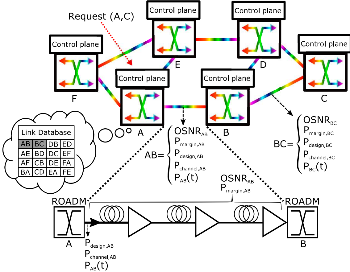
Figure 3.7: Network example.
