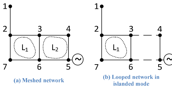
Figure IV-6 – Illustration of the limit of the constraint (IV.49) if some DGs are producing enough to supply power to the close loads
