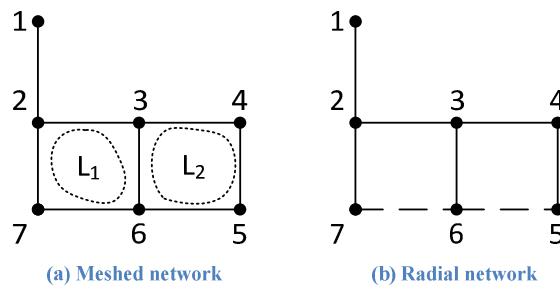
Figure IV-5 – Effect of the constraint (IV.49) on a meshed network without DG
