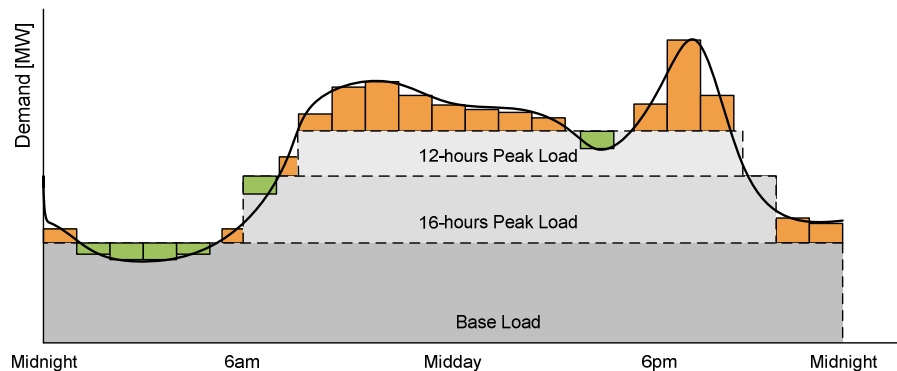
Figure I-13 – Procurement of energy blocks by a BRP in the different energy markets [KOK-13]
