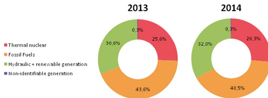
Figure I-2 - Generation mix repartition in ENTSO-E member TSO's countries in 2013 and 2014 [EUR1-15]
