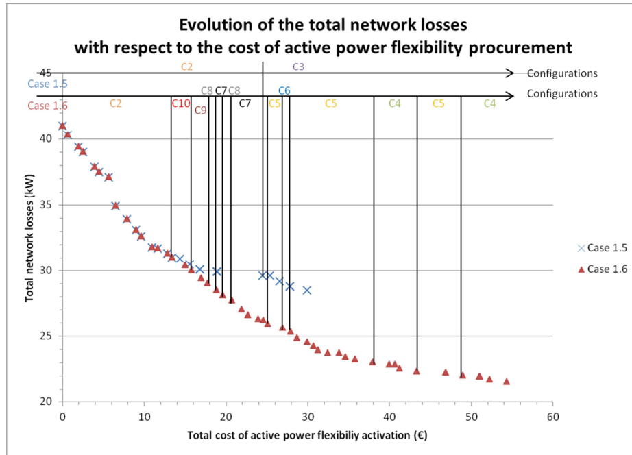
Figure IV-17 – Evolution of the 33-nodes network losses optimization solutions with respect to the maximum admissible cost of active power flexibility procurement in cases 1.5 and 1. 6
