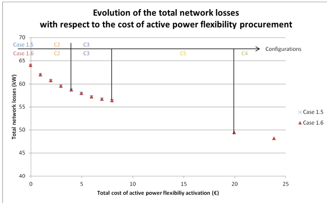
Figure IV-18– Evolution of the 72-nodes network losses optimization solutions with respect to the maximum admissible cost of active power flexibility procurement in cases 1.5 and 1. 6
