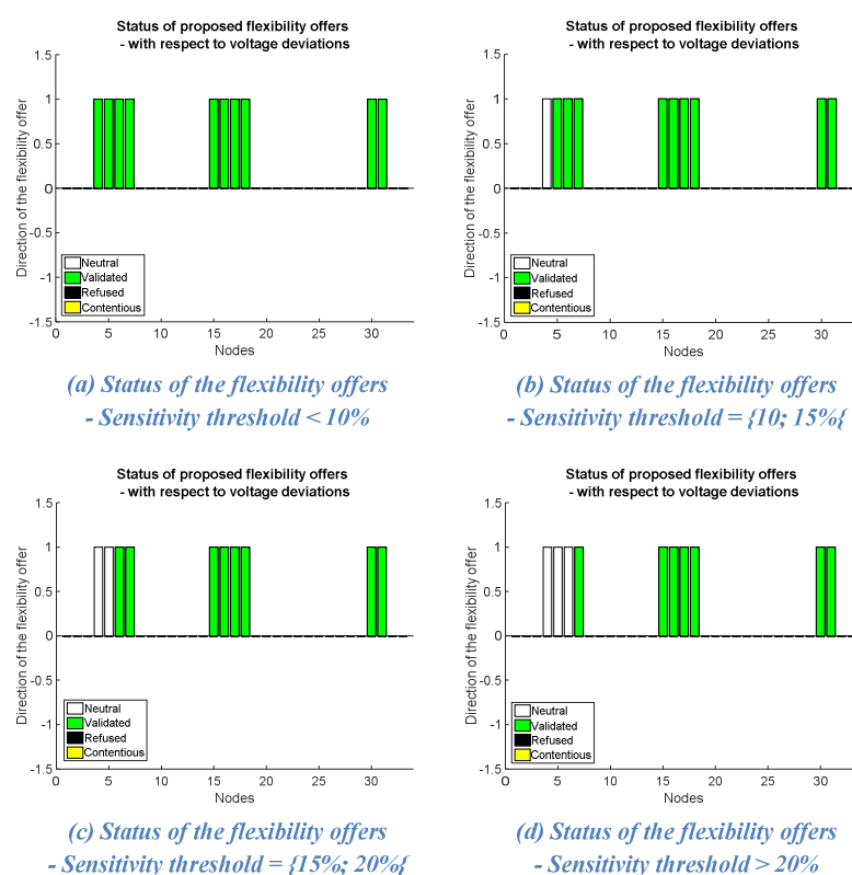
Figure AVIII-6 – Impact of the sensitivity threshold on the statuses of the flexibility offers (33-nodes network, test case 2)
