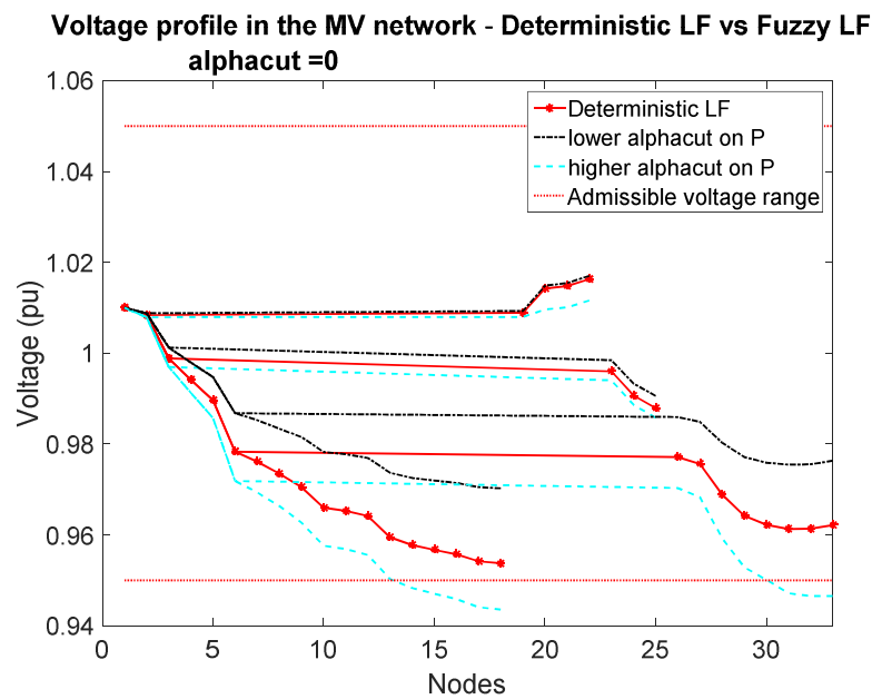
Figure III-13 - Fuzzy voltage profiles in the 33-nodes network ( \alpha=0 )/ second set of flexibility offers
