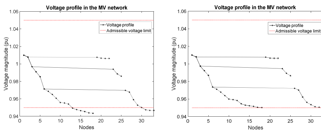
(a) Voltage profile in case of sudden changes in the weather conditions (no local production anymore) (4p.m)
