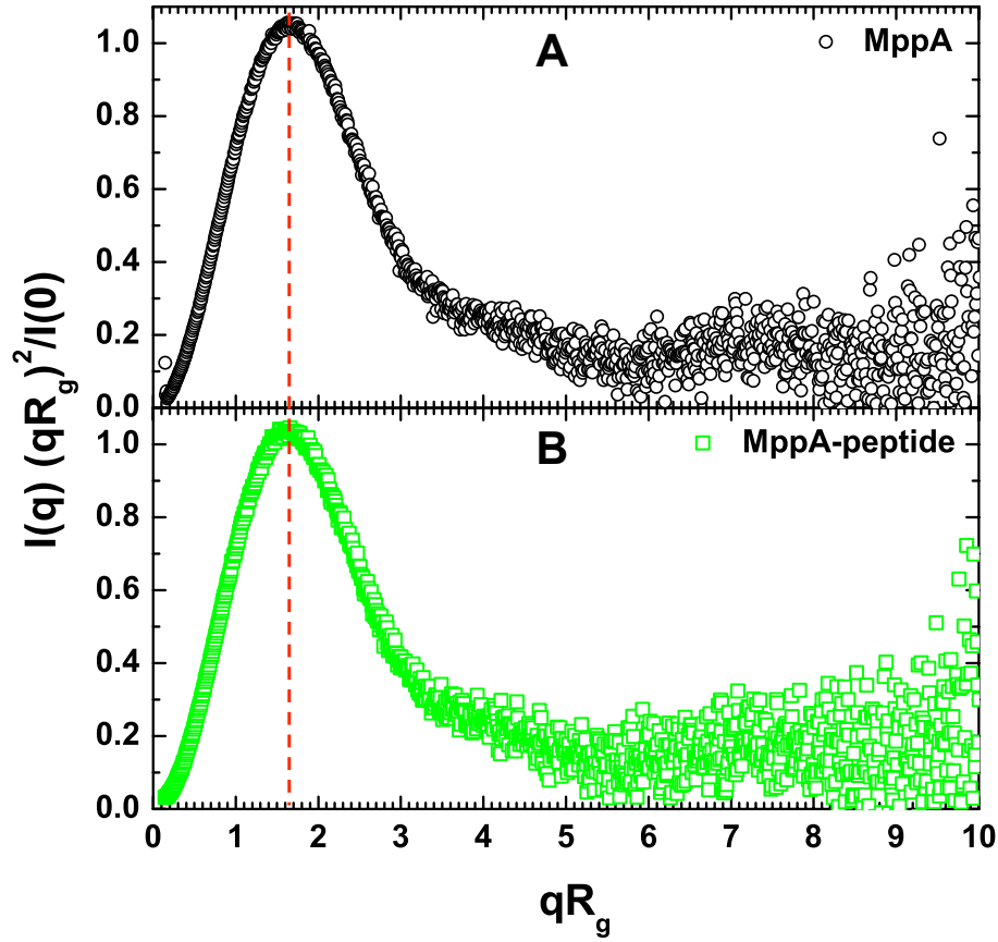
Figure 6.3: Kratky plots for (A) MppA and (B) MppA-peptide, which has the bell-shaped feature in the range 0 < qR_g < 3 with maximum at qR_g \sim 1.7 . These plots strongly confirms that the protein has compact folded structure in solution.
