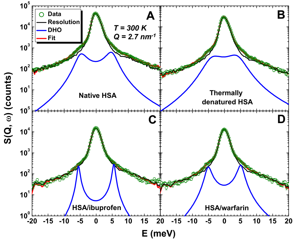
Figure 5.9: Dynamic coherent structure factor measured from (A) native HSA, (B) thermally denatured HSA, (C) HSA/ibuprofen and (D) HSA/warfarin, and corresponding fitting with Eq. 5.4 at Q = 2.7 \text{ nm}^{-1} and T = 300 \text{ K} . The green circles, black, blue and red curves indicate the experimental data, resolution, DHO function with two Brillouin-side peaks and the best fit to the data, respectively. The hydration levels ( h ) for all the samples were \sim 0.4 .
