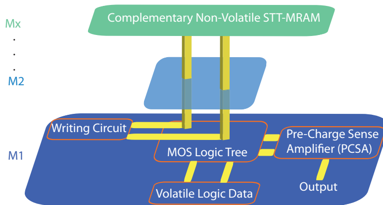
Figure 2.12: General architecture of logic in memory based on STT-MRAM: Mx represents the highest level of metal in CMOS technology.
