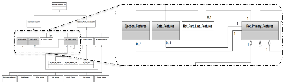
Figure 30 Relationships between rotational primary features and gate features and primary features and ejection features.
