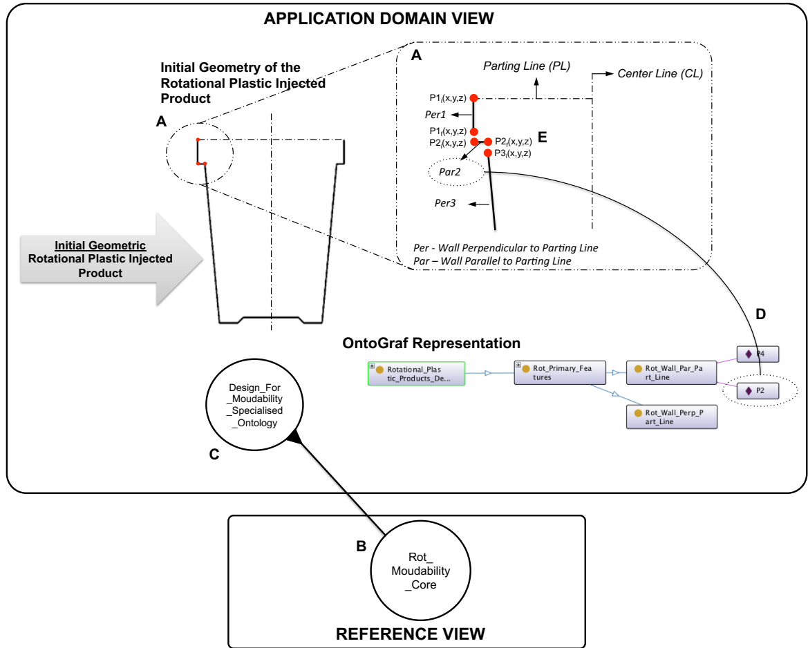
Figure 59 Controlled Specialisation Approach.
