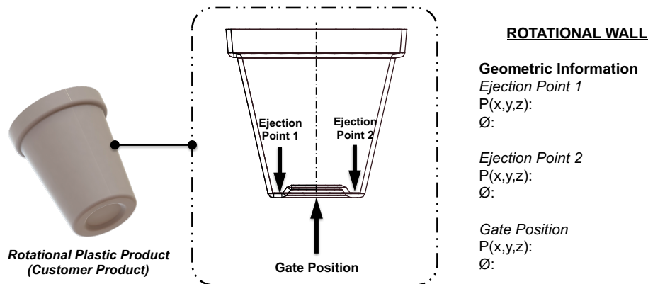
Figure 31 Gate and Ejection Features in Plastic Injected Products.
