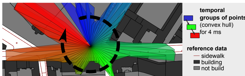
Figure 22: Rotating Lidar (Velodyne) with strong temporal dependency (200 ms acquisition).
