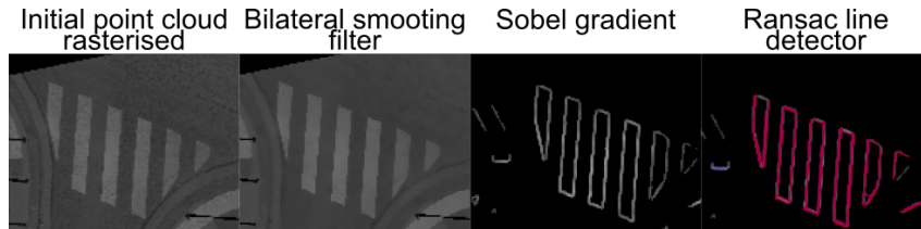
Figure 27: A part of a point cloud is converted to a raster. We use bilateral smoothing, gradient (Sobel), and line detection (RRANSAC by Chum and Matas, 2002) to reconstruct the pedestrian crossing. These operations are much faster and easier on rasters rather than points.
