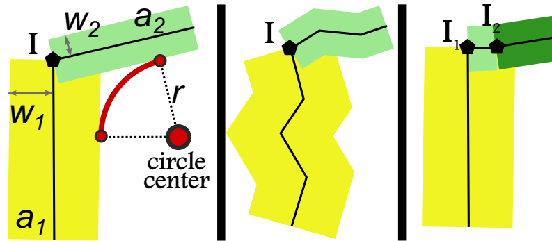
Figure 50: Finding the circle centre problem. Left classical problem, middle and right using real-world data.
