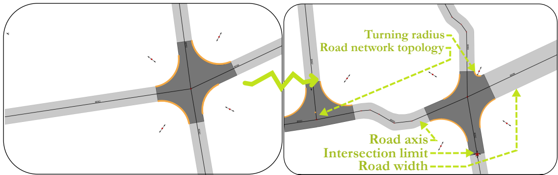
Figure 95: StreetGen road model parameters, each can be modified using in-base interaction.
