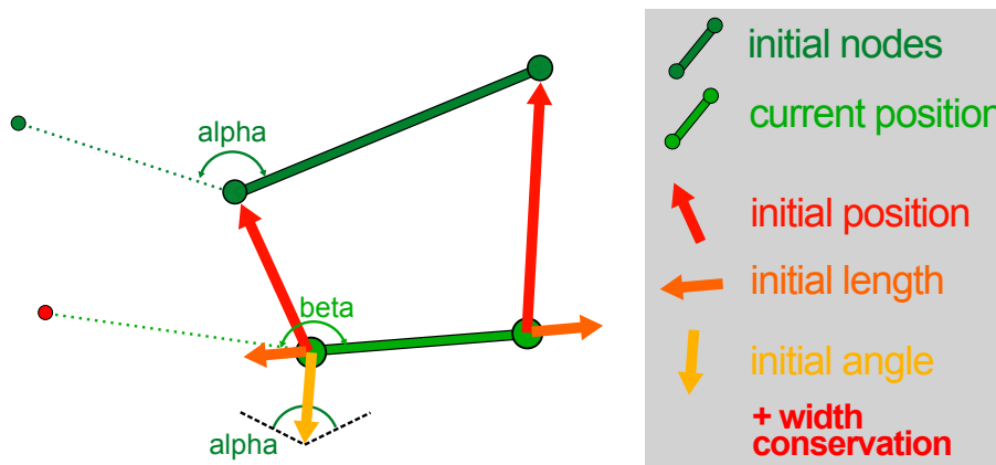
Figure 114: Regularisation forces that work to preserve initial values of parameters. The "initial position" force tends to preserve each node initial position. The "initial length" force tends to preserve each road segment length. The "initial angle" force tends to preserve initial angle between road segments. The "initial width" tends to preserve the initial width of each road segments.
