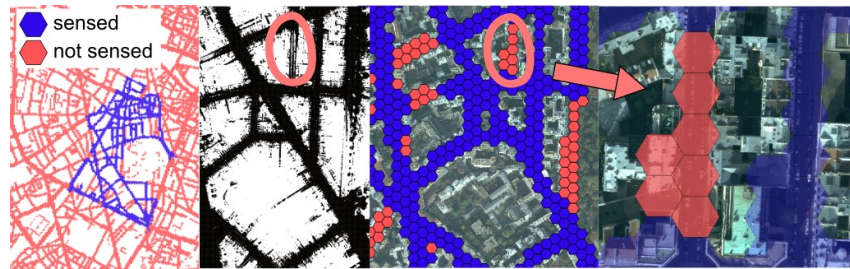
Figure 37: "To-Do" hexagonal map showing the places where the mapping vehicle has not sensed enough points (red hexagon), and where the sensing is sufficient (blue hexagon). Without this map, the zoomed missing part is challenging to notice on raw data.
