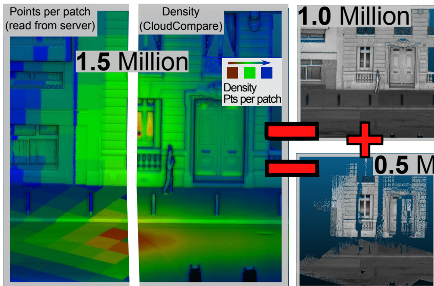
Figure 140: Abnormal density detection and correction. Top points per patch (left) or density (right), green-yellow-red. Bottom reflectance in grey.
