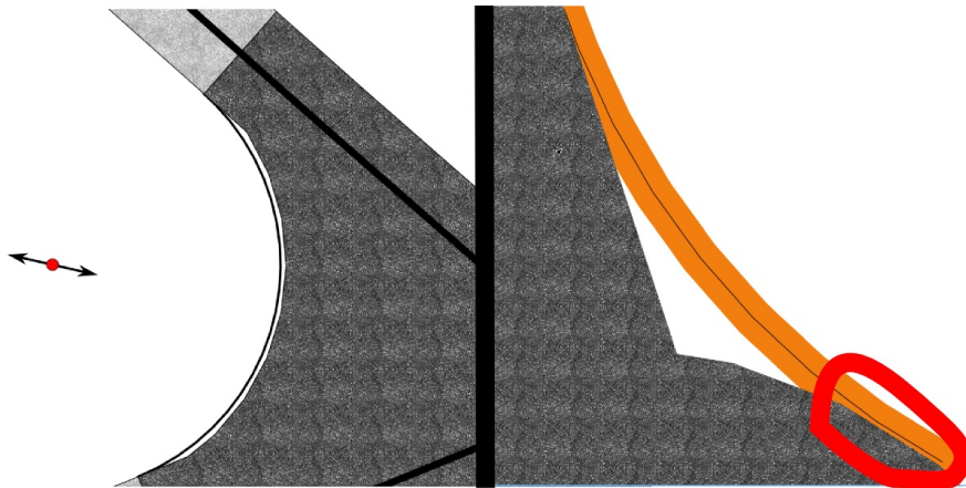
Figure 79: Example of a precision issue. Left, we approximate arcs with segments, which introduces errors. Right, the error was sufficient to incorrectly union the intersection surface.
