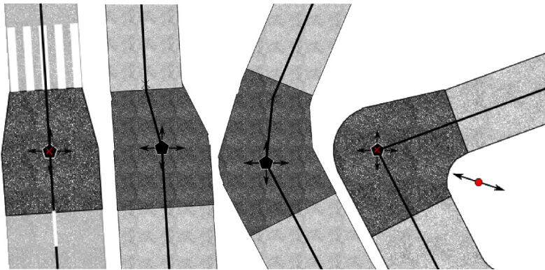
Figure 55: Variable buffer for robust roadway width transition.
