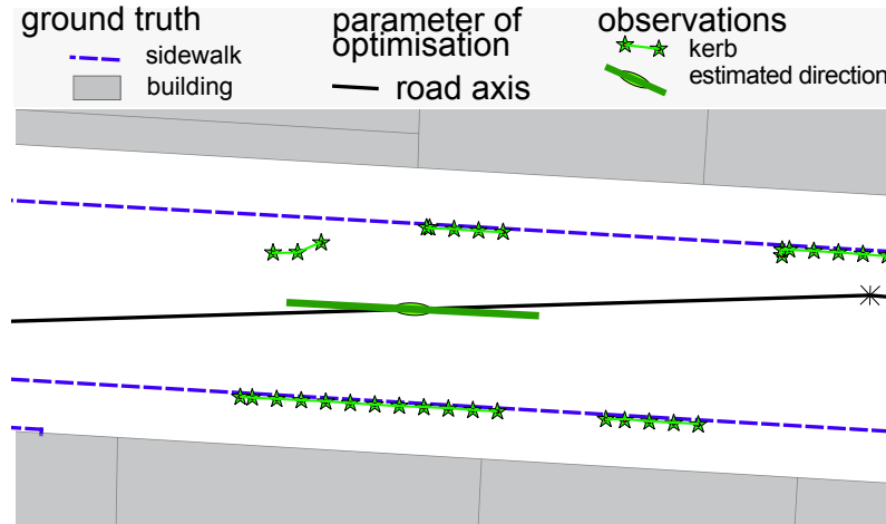
Figure 112: Estimated road axis segment slope based on weighted median of kerb observations. The estimated slope is coherent with the ground truth, and is very different from the road axis to be optimised.
