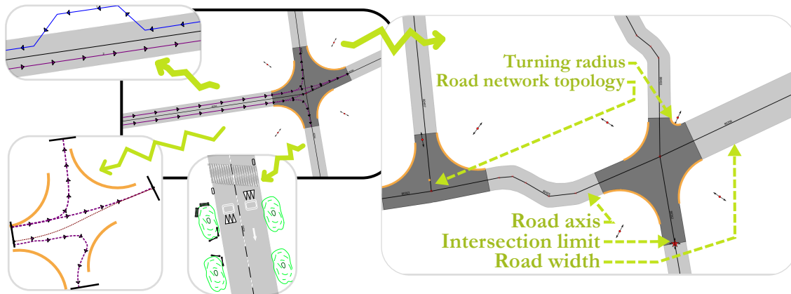
Figure 81: Interaction is handled in-base rather than in custom software. Street model is regenerated automatically (StreetGen) when user edit street model parameters using convenient and effective interactors. Road model, traffic information and street features can be edited.
