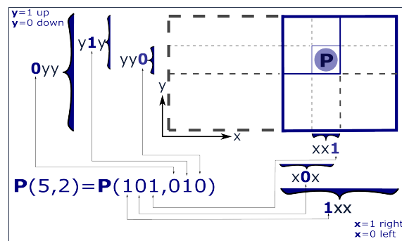
Figure 141: Principle of binary coordinates for a centered, scaled and quantized point cloud.
