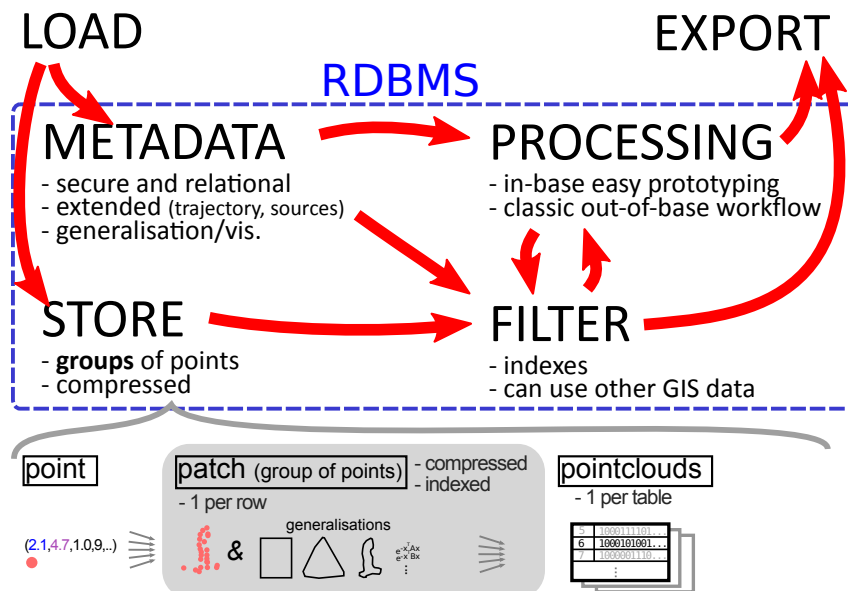
Figure 144: Overall and storage organisations of the Point Cloud Server.
