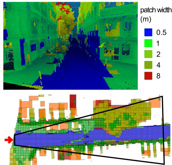
Figure 34: Illustration of variable patch size repartition in an urban point cloud.
