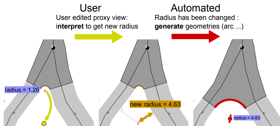
Figure 90: The curbstone arc centre is generated from the radius value and other geometries. We use it as an indirect geometric controller through a "Proxy view". The user edits the arc centre using this view, which is interpreted as a new radius. Then, another trigger re-generates arc centre and other geometries based on the new radius. No infinite cyclic trigger call occurs thanks to the proxy view which separates automated changes and user changes.
