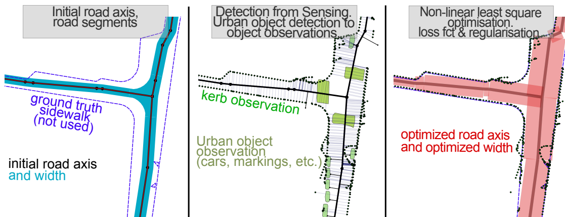
Figure 104: Approximate road axis network and road width are available, forming a basic road modelling. Various sensing methods produce urban feature detections which are processed into consolidated observations, and assigned to road axis segments. A robust non linear least square optimisation then fits the road modelling to observations. The result is much closer to ground truth, even when the road model is too simple for the actual road configuration (varying width, asymmetric changes, curves). The user can further input observations if necessary.
