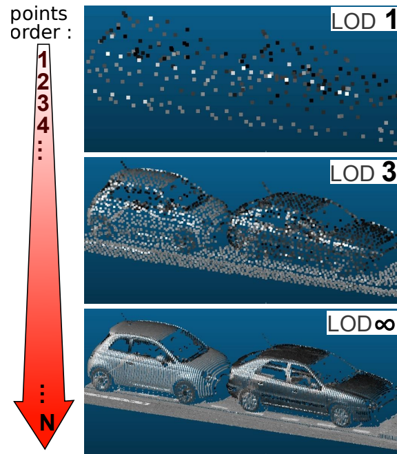
Figure 135: 3 Geometrical Level Of Detail (LOD) for the same point cloud. Reading points from 1 to N gradually increases the details, because of the specific order of points (MidOc).
