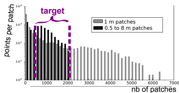
Figure 35: Histogram of points per patch for constant and variable size patch. Using variable size patch strongly reduces the number of very small or very large patches. Total number of patches is roughly conserved.
