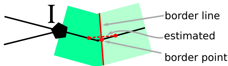
Figure 53: Creating the border line by cutting the section following a local estimation of the normal.
