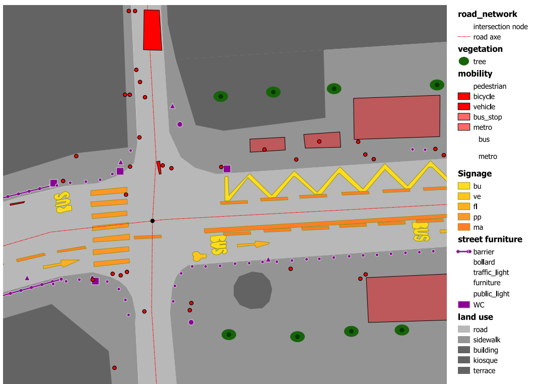
Figure 16: Vector data: various vector types forming a map.
