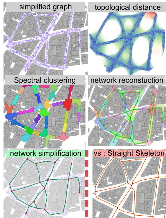
Figure 43: From simplified graph, all topological distance from a vertex to any vertices close enough are computed with PGRouting, the result is clustered using spectral clustering of Pedregosa et al., 2011. We then reconstruct the network with PostGIS Topology, and perform a final simplification step. For comparison an automated result using a straight skeleton based method.
