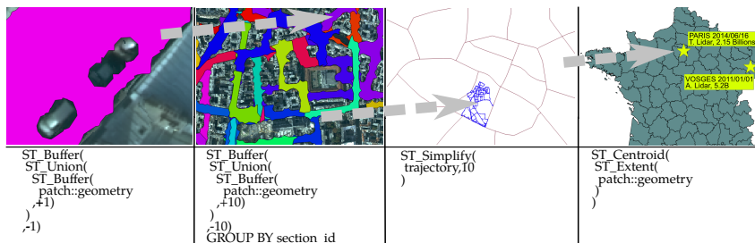
Figure 36: Successive visualisations (various scale) of point cloud coverage, see 2.3.3 for details.
