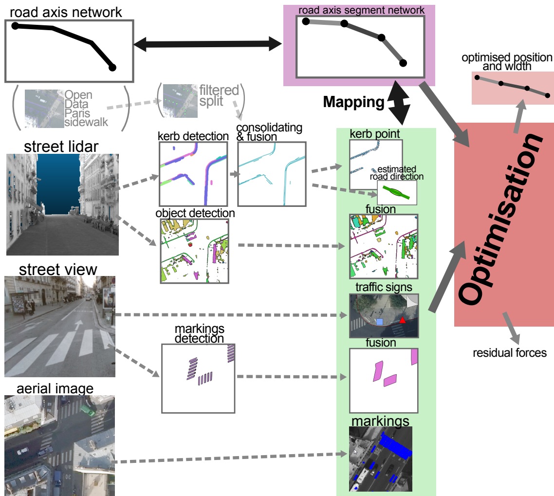
Figure 108: Data sources for optimisation. The input road axis network is refined into a road axis segment network. We use the detections from several methods. Those detections are processed to become useful observations, which are associated with road segments. The optimisation produces new road segment widths and positions.
