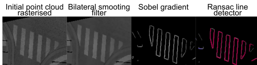
Figure 27: A part of a point cloud is converted to a raster. We use bilateral smoothing, gradient (Sobel), and line detection (RRANSAC by Chum and Matas, 2002) to reconstruct the pedestrian crossing. These operations are much faster and easier on rasters rather than points.
