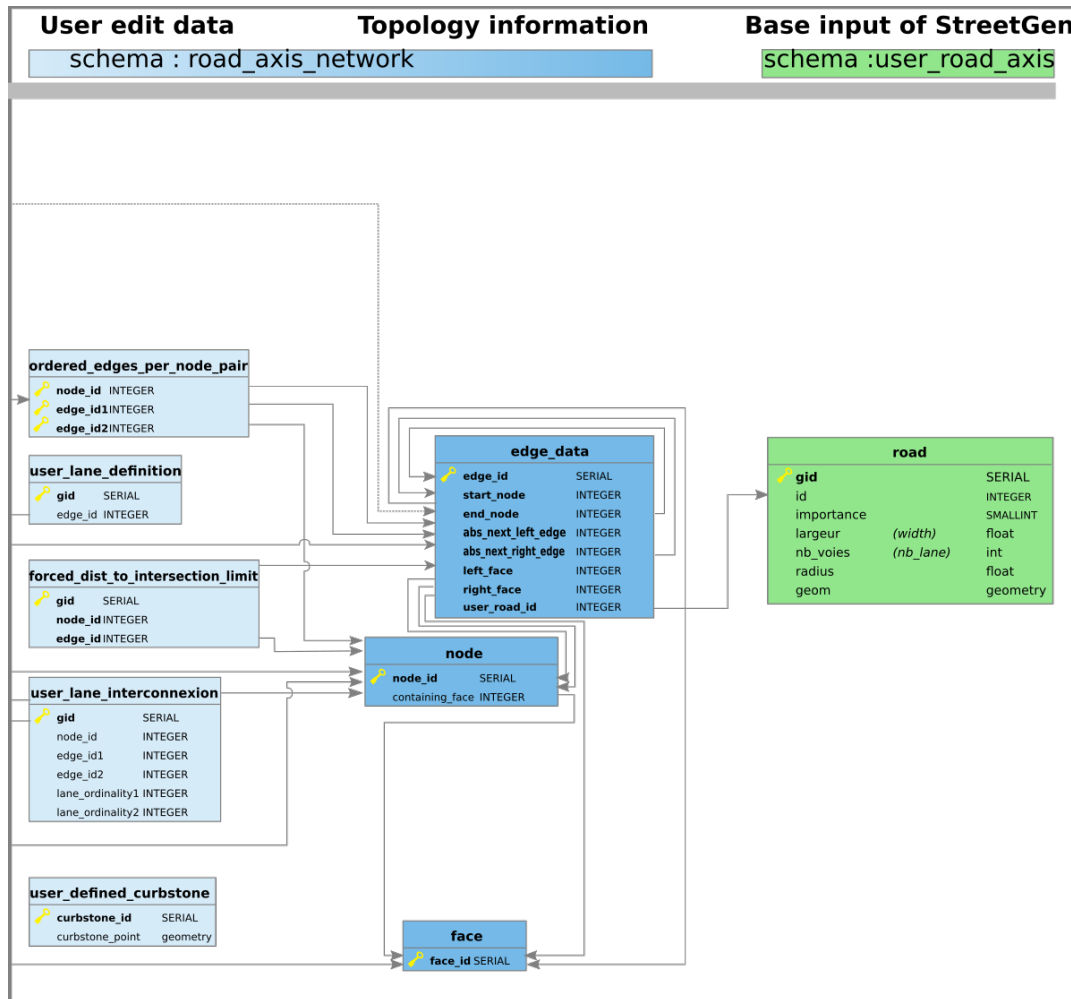
Figure 160: StreetGen base table schema in database (part 2/2)
