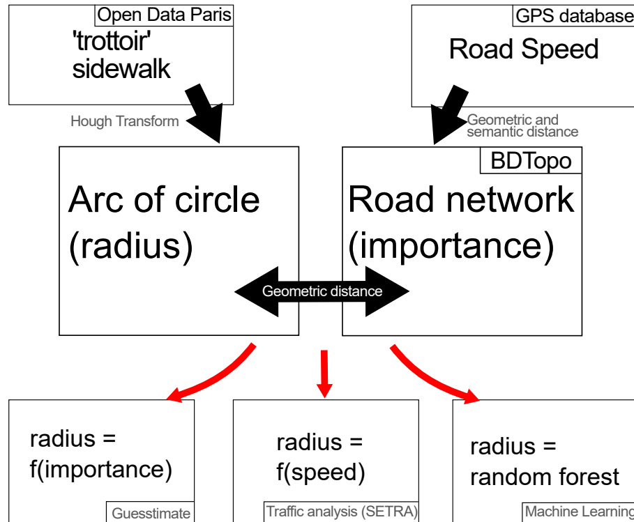
Figure 67: Workflow to test radius hypothesis.
