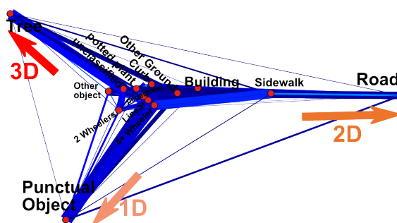
Figure 150: Spectral clustering of confusion matrix of Paris data set classification using only ppl descriptor. Edge width and colour are proportional to affinity. Node position is determined fully automatically. Red-ish arrows are manually placed as visual clues.
