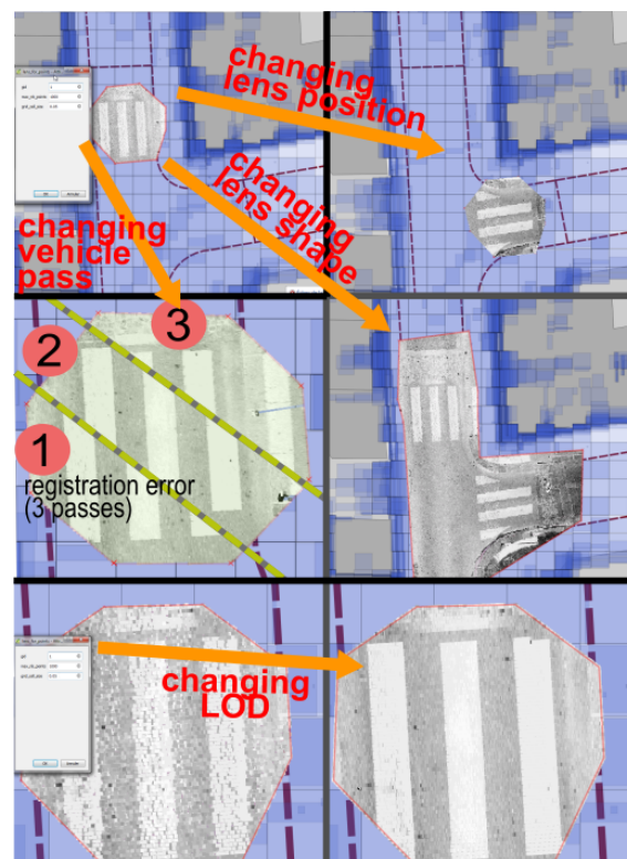
Figure 31: A polygon representing a lens that reveals points underneath it (among billions), with a given Level Of Detail and vehicle pass, at about 100 kpts /s. Points are automatically updated when the lens is modified by the user, using a pure in-base solution, which makes it compatible with any client.
