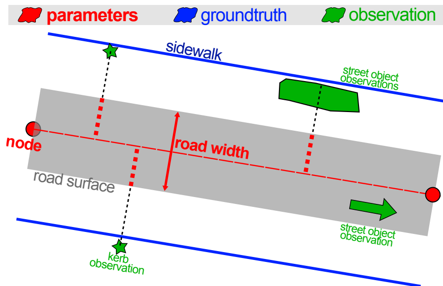
Figure 106: A roadway is modelled with connected nodes and width, which implicitly describes a crude road surface (a rectangles). Observations are defined regarding the implicit road surface.
