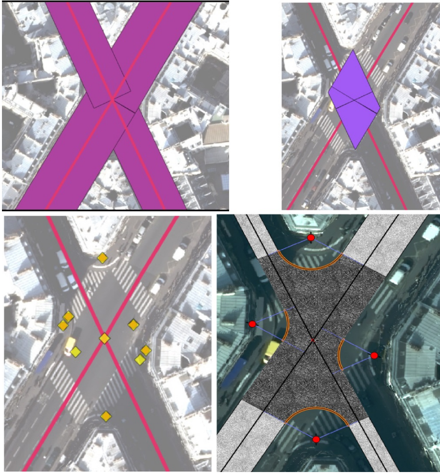
Figure 51: A method to robustly find circle centres using geometric operations. Buffer of axis is computed, then the intersection of outer ring of buffer returns a set of candidates points. Among the candidates, the one closest to the intersection centre are the final circle centre.
