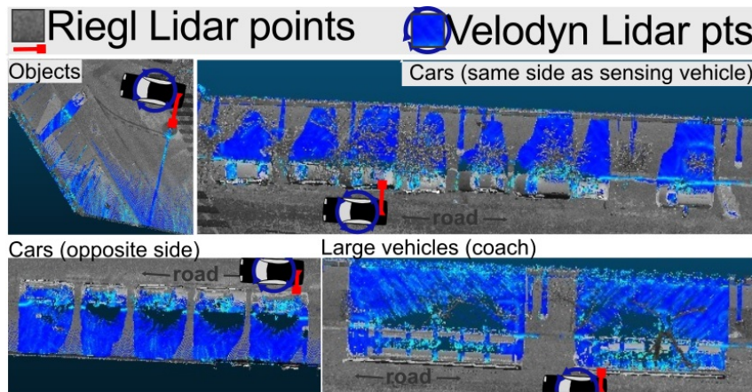
Figure 129: Point cloud sensing with static Lidar (Riegl) is occluded by cars and street objects, which hides side-walks. Adding a rotating Lidar (Velodyne) greatly reduces occlusion because the same spot can be sensed from different angles.
