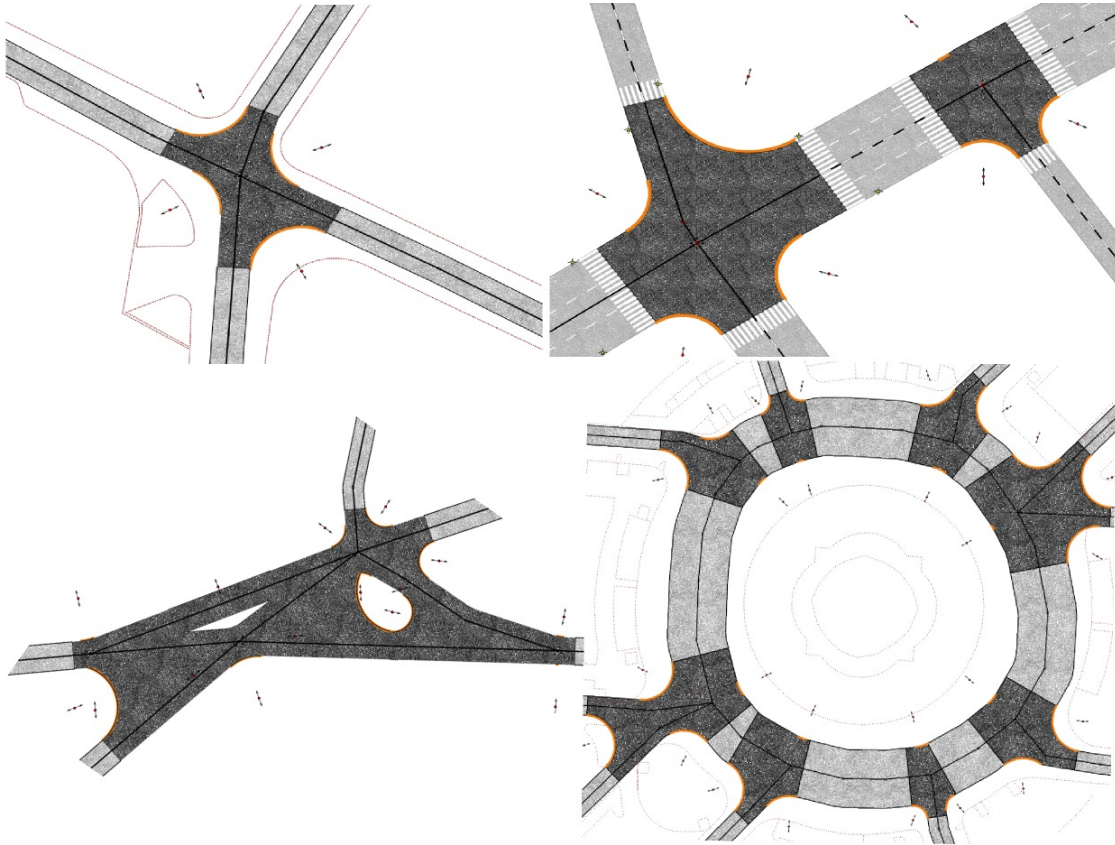
Figure 70: Example of results of increasingly complex intersection.
