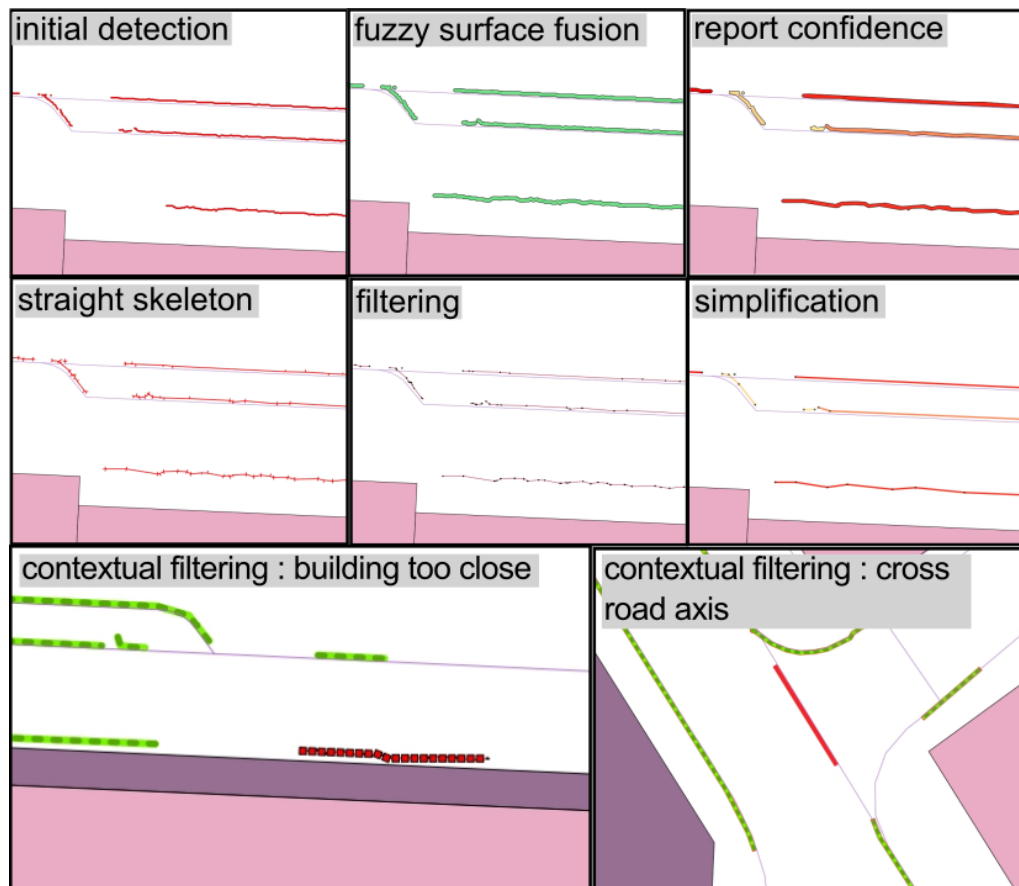
Figure 110: Input kerb detection is consolidated and filtered (both geometrically and with context) to produce suitable observations.
