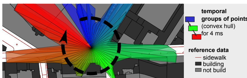
Figure 22: Rotating Lidar (Velodyn) with strong temporal dependency (200 ms acquisition).
