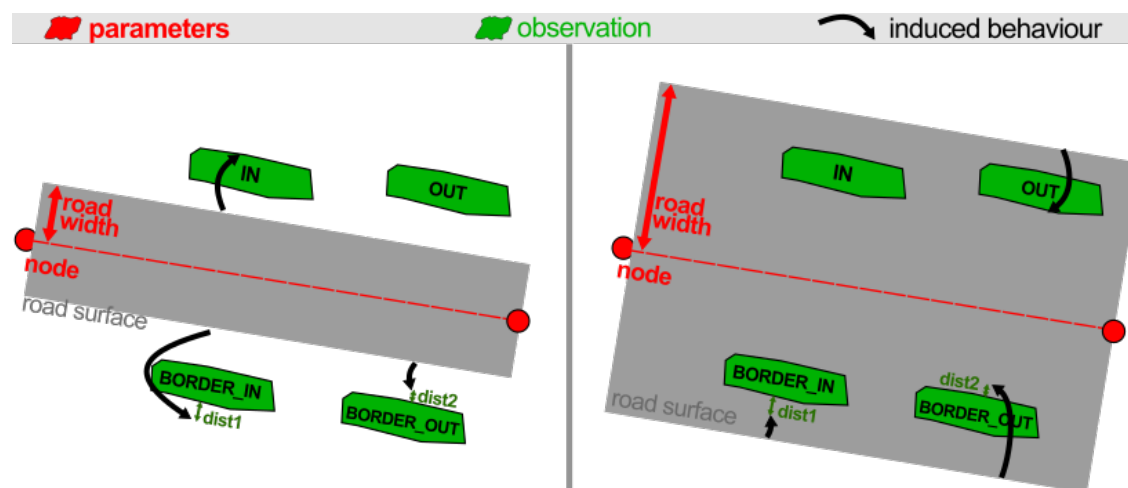
Figure 107: Each expected observation position is defined regarding the implicit road surface, with four options: In, Out, Border_in, Border_out. When Border is used, a distance to the road surface limit can be defined (dist1, dist2 here).
