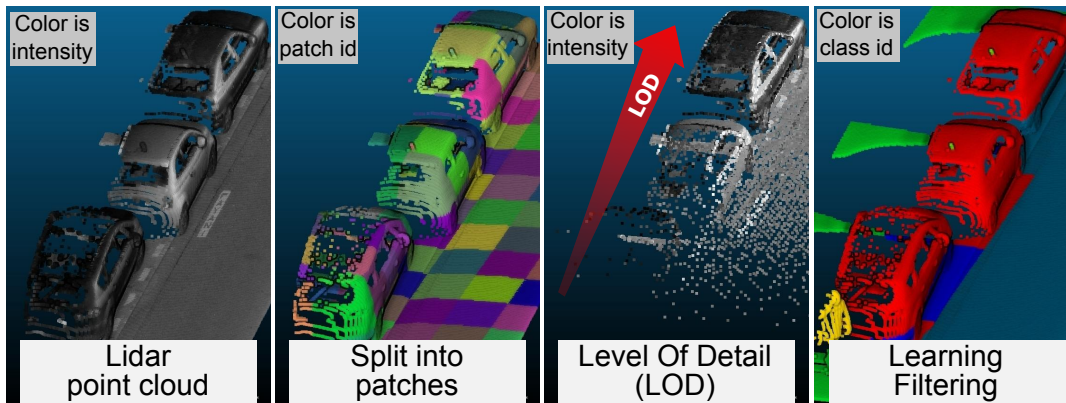
Figure 131: Graphical Abstract : a Lidar point cloud (1), is split it into patches (2) and stored in a Point Cloud Server, patches are re-ordered to obtain free LOD (3) (a gradient of LOD here), lastly the ordering by-product is a multiscale dimensionality descriptor used as a feature for learning and efficient filtering (4).
