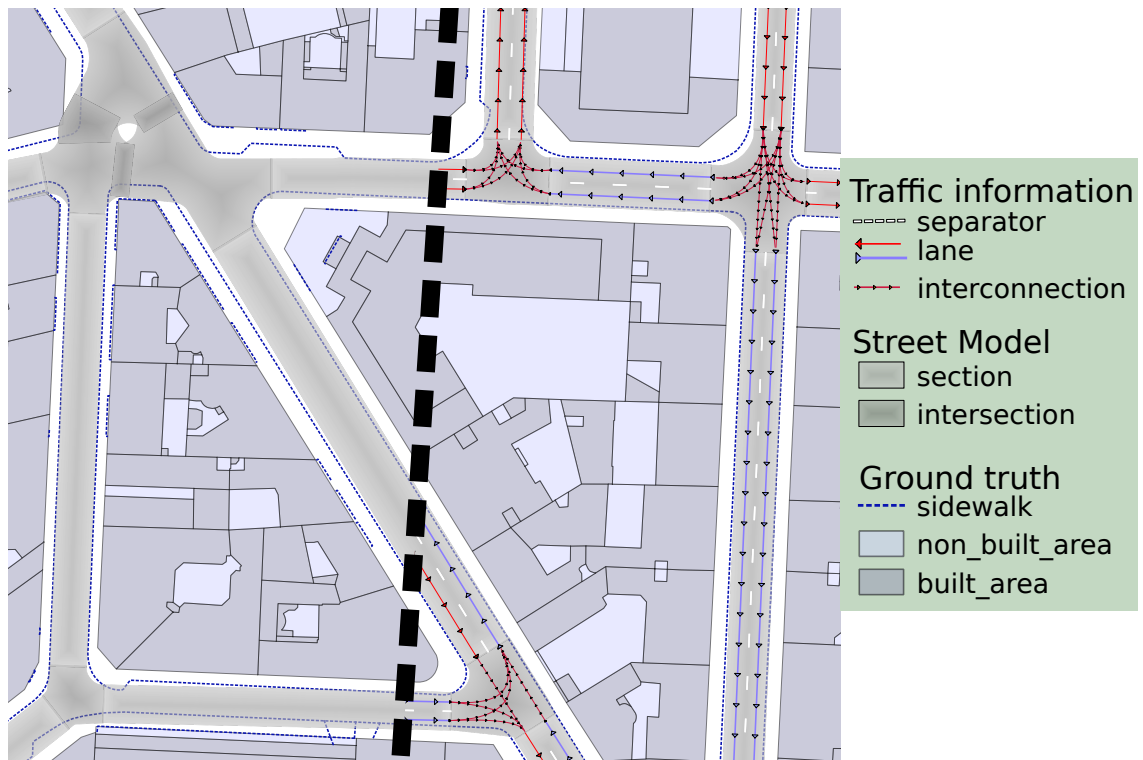
Figure 116: We use the optimised road model (kerb observation from sensing) as input to Street-Gen to generate a complete street model. Note that turning radius have not been optimised.
