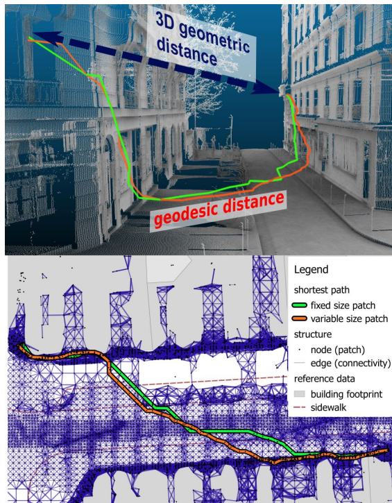
Figure 41: Two views of shortest path on regular (yellow) and varying (orange) size patches.~ 100ms
