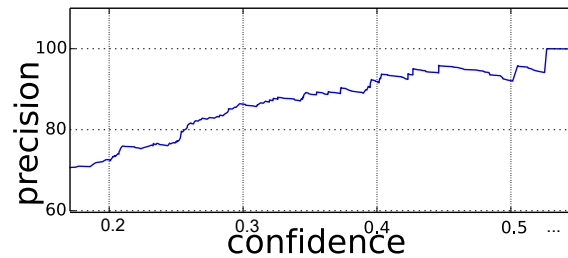
Figure 158: Precision of 4+wheelers class is a roughly rising function of random forest confidence scores.
