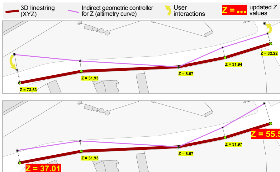
Figure 89: An indirect geometric controller is used to change the Z values of points of a 3D linestring within a traditional 2D GIS interface (here: QGIS). The altimetry curve is both a visualisation tool and an easy edit tool.
