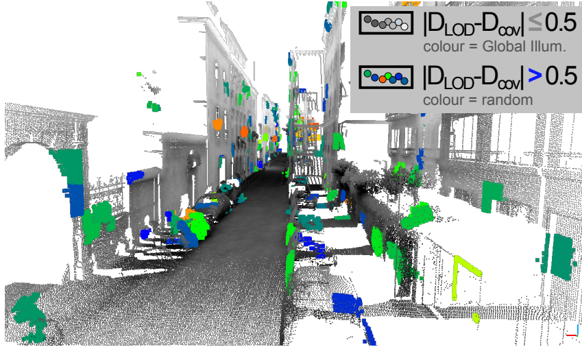
Figure 148: \text{Dim}_{\text{LOD}} and \text{Dim}_{\text{cov}} are mostly comparable, except for few patches (5%, coloured)
