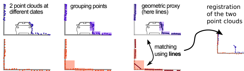
Figure 44: A schematic example of the benefits of using generalisation of points for fast registering. The critical part of matching could be done on geometric proxies instead of points, reducing the number of entities to be matched by a factor of at least 10^3 .
