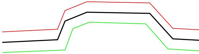
Figure 56: Starting from center line (black), a translation would not create correct a lane (red). We must use the buffer (green).
