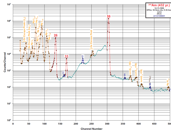
Figure 5.7 : Gamma-ray spectrum of {}^{241}\text{Am} taken from the website www.radiochemistry.org
