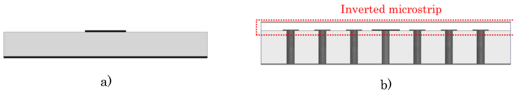
Figure 2.27. Front view of: a) Microstrip line, b) Gap waveguide.
