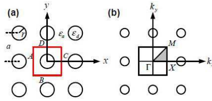
Figure 2.15. Brillouin zone of periodic pattern.
