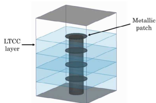
Figure 4.56. Insertion of a "metallic patch" in each LTCC layer to solve the via filling problems.
