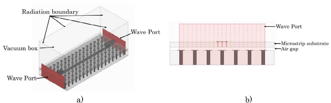
Figure 4.11. Microstrip-to-gap waveguide back-to-back transition: a) 3D view of the structure with HFSS, b) E-field distribution in the wave port excitation.
