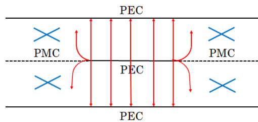
Figure 2.4. Stripline configuration.
