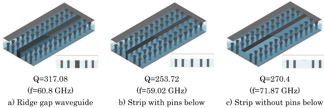
Figure 2.35. Three configurations based on gap waveguide concept.
