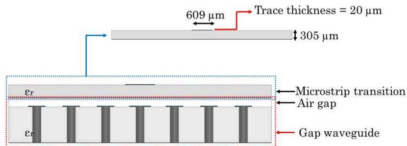
Figure 4.8. Front view and dimensions of the aperture coupled microstrip to gap waveguide transition.
