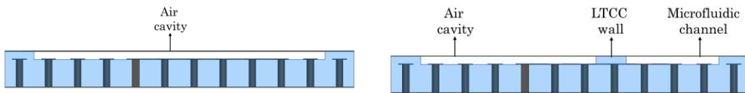
Figure 5.5. Front view of the gap waveguide resonator: Without and with the LTCC wall to separate the air cavity from the microfluidic channel.
