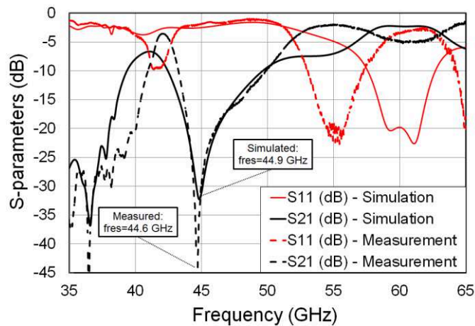
Figure 5.21. Computed and measured results for the gap waveguide resonator GW6.
