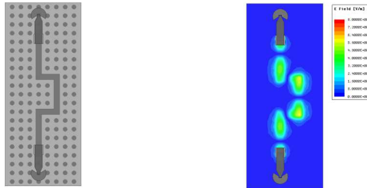
Figure 4.25. Top view of the gap waveguide with two 90^\circ bends. E-field view in the ground plane with the H-shape apertures at 52 GHz.
