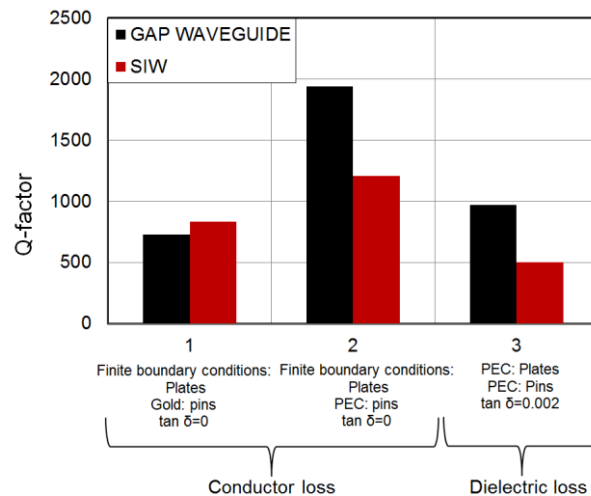
Figure 3.19. Q-factor obtained with the Eigenmode of HFSS considering dielectric, conductor, both or any losses.
