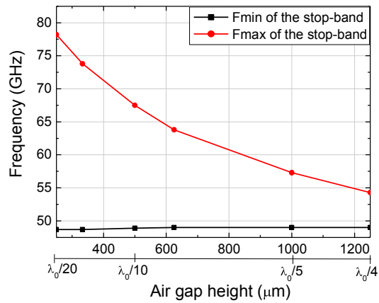
Figure 2.38. Computed minimum and maximum frequency of the stop-band.
