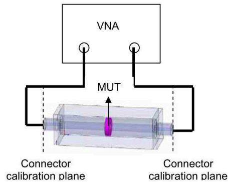
Figure 1.9. Transmission method for material characterization using waveguide transmission line.
