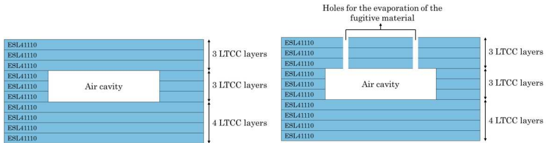
Figure 4.35. Geometry of the internal cavities.
