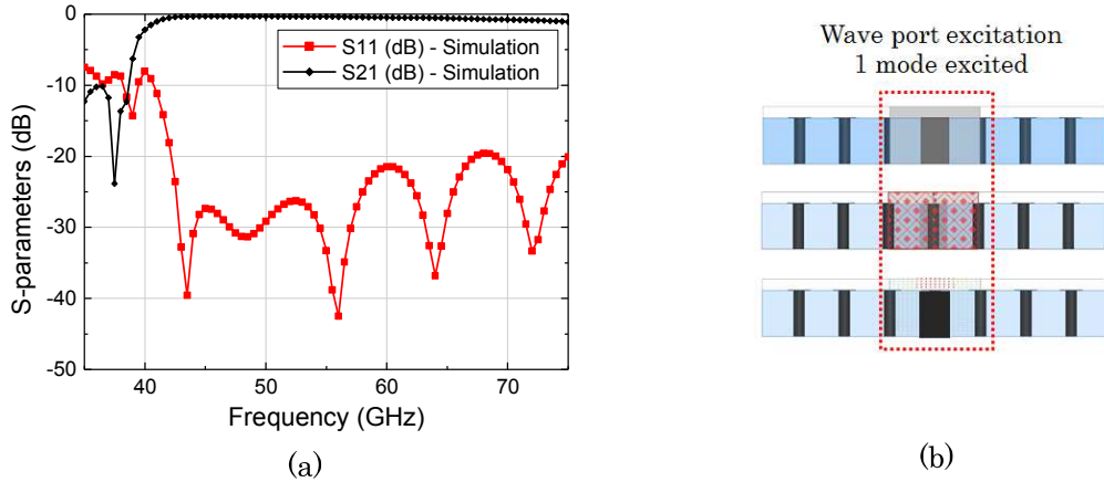
Figure 4.7. Gap waveguide with RO4003 substrate. a) Transmission and reflection coefficients b) Wave port excitation in HFSS.
