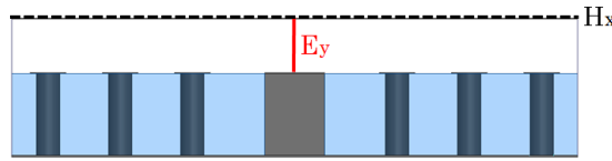
Figure 2.28. Integration lines used in the simulations
