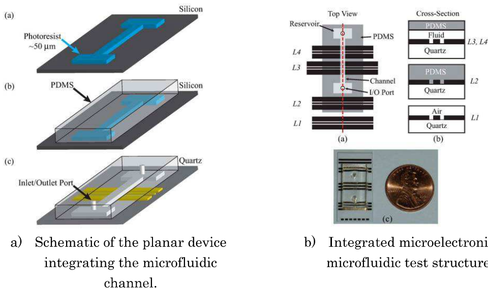
Figure 1.11. Measurement system based on microfluidic channels embedded in coplanar transmission lines proposed in [14].
