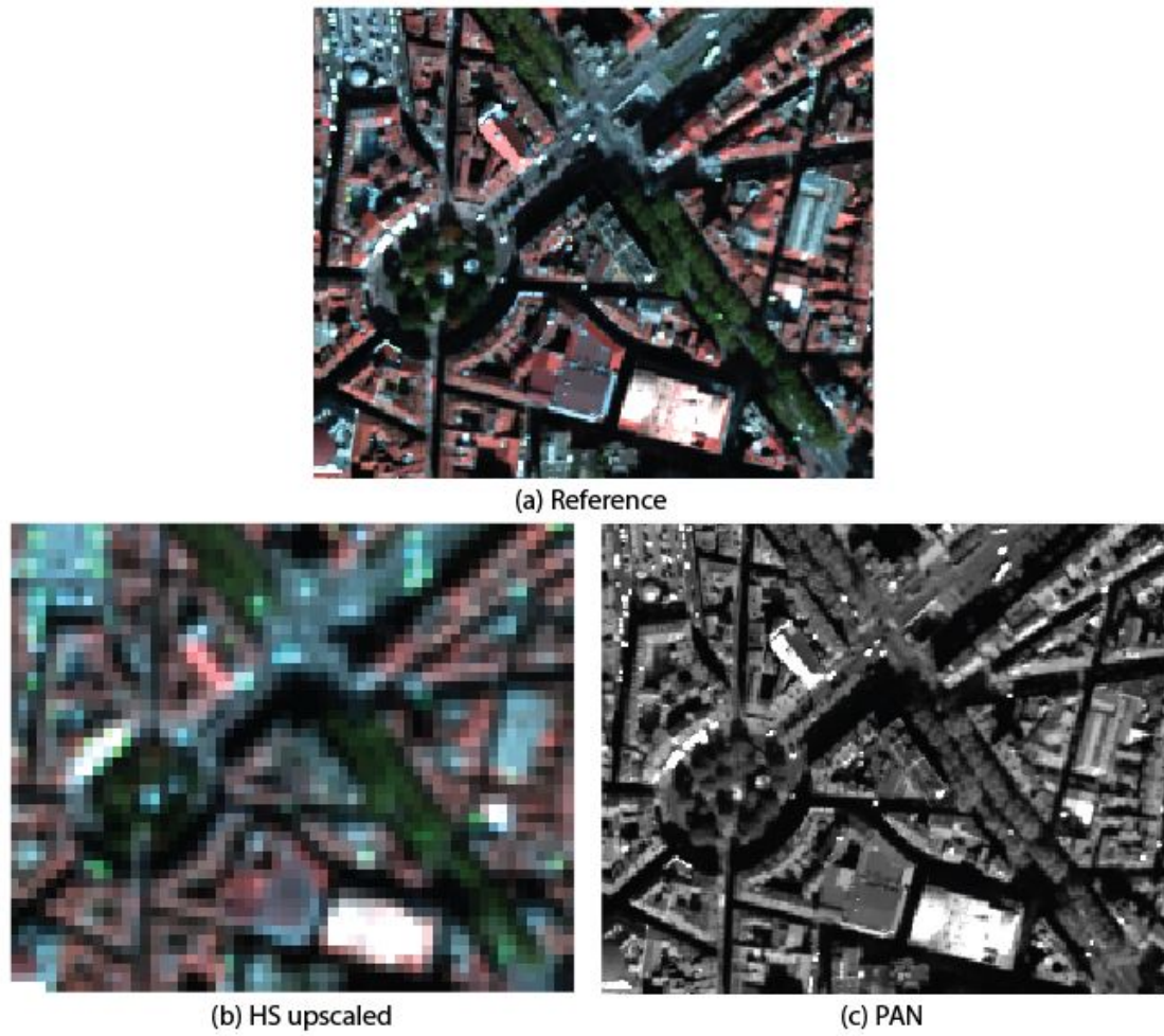
Figure 4.4: Toulouse dataset
