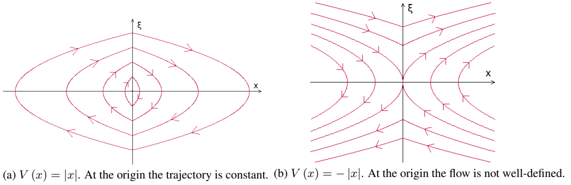
Figure 3.1.1: A glance on the classical flows for the potentials V(x) = \pm|x| near the origin. The arrows indicate their orientation.
