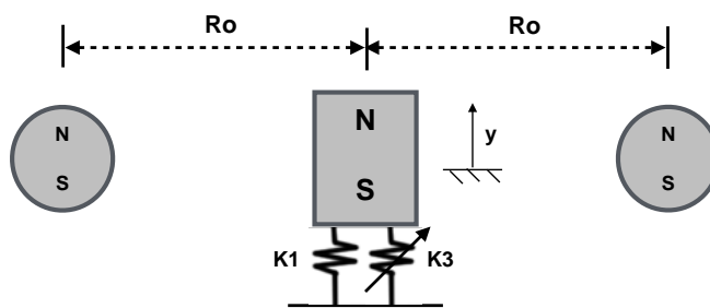
Figure 4.4: Schematic
