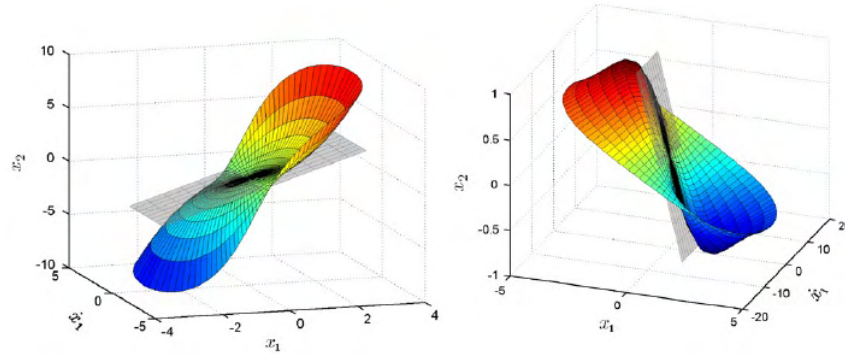
Figure 2.11: Invariant Manifolds of Nonlinear Normal Modes as defined by Shaw and Pierre [SP91,SP93].
