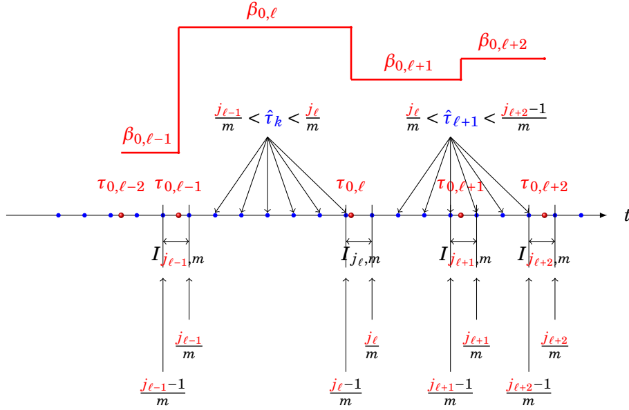
Fig. 2.9 – A zoom into the Case I.
