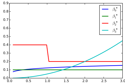
Fig. 4.1 – Baseline and true regression coefficients.
