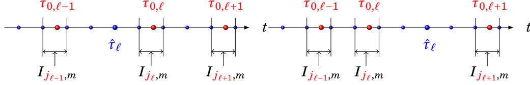
Fig. 2.7 – First case in the proof of Theorem 2.4.4: Case I. \hat{j}_\ell < j_\ell . Fig. 2.8 – Second case in the proof of Theorem 2.4.4: Case II. \hat{j}_\ell > j_\ell .
