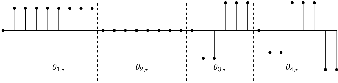
Fig. 3.1 – Illustration of \theta = (\theta_{1,\bullet}^\top \cdots \theta_{p,\bullet}^\top)^\top with: p = 4, d_1 = 9, d_2 = 8, d_3 = 6, d_4 = 8 .
