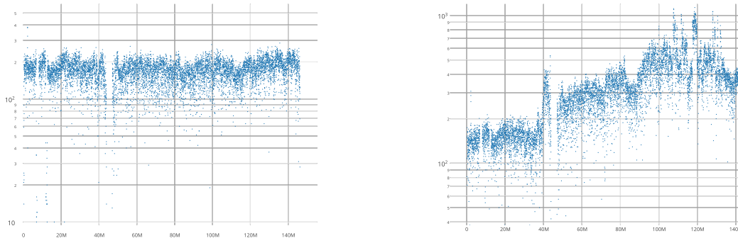
Fig. 2.5 – Binned counts of reads (log-scale) of the normal (left) and tumor (right) data.
