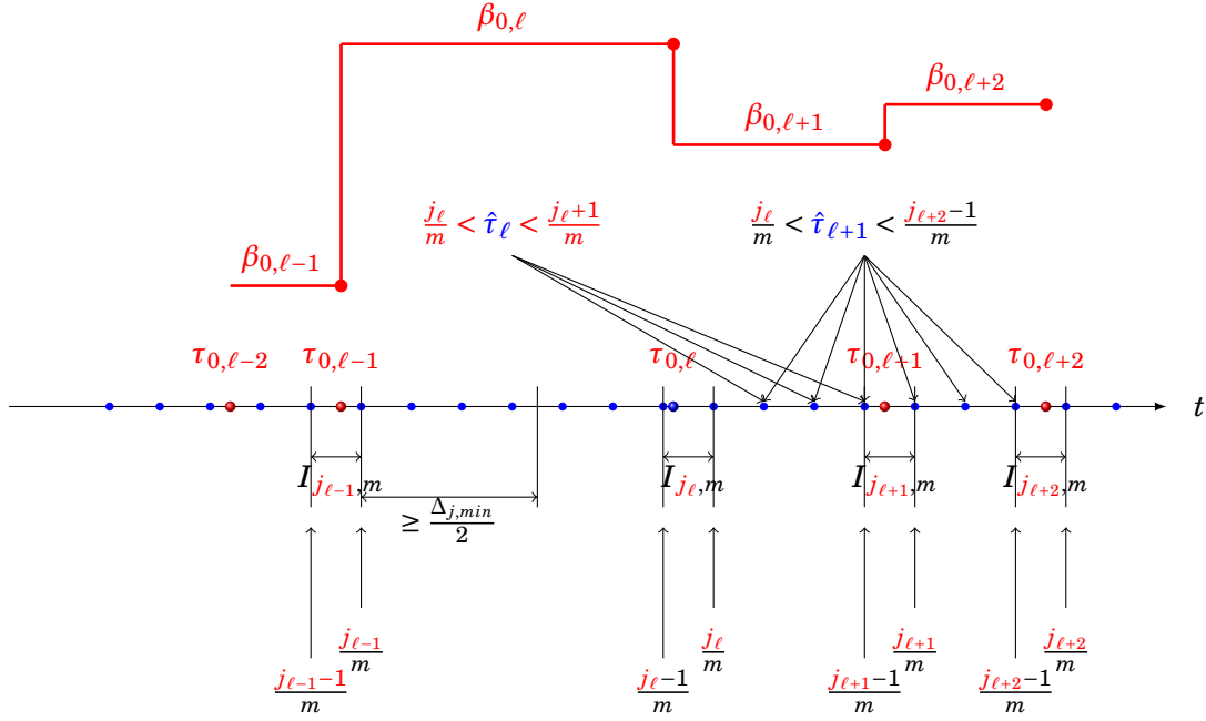
Fig. 2.B.1 – A zoom into the Case II.
