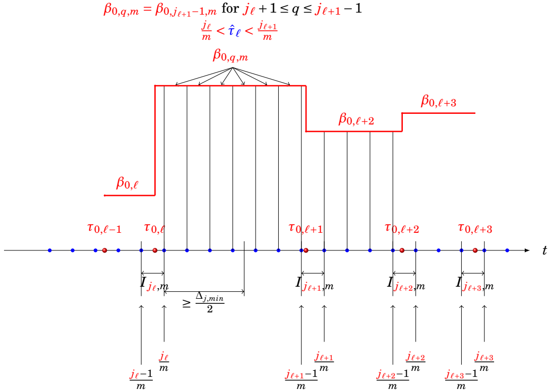
Fig. 2.B.2 – A zoom of \beta_{0,q,m} , the coefficients of the projection function \lambda_{0,m} in Case II.
