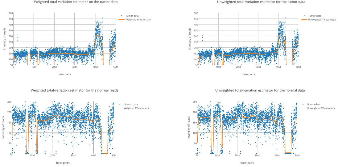
Fig. 2.6 – A zoom between reads number 0 and 50M of the weighted and unweighted total-variation estimators applied to the tumor and normal data.
