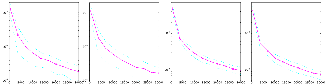
Fig. 2.3 – Average MISEs (bold lines) over 100 Monte-Carlo experiments and standard deviations of the MISEs (dashed lines). First: weighted TV for Example 1; Second: non-weighted TV for Example 1; Third: weighted TV for Example 2; Fourth: non-weighted TV for Example 2.
