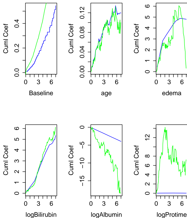
Fig. 4.3 – Estimated cumulative regression coefficients on PBC data: with CoxSGD (blue) and timereg R-package (green).
