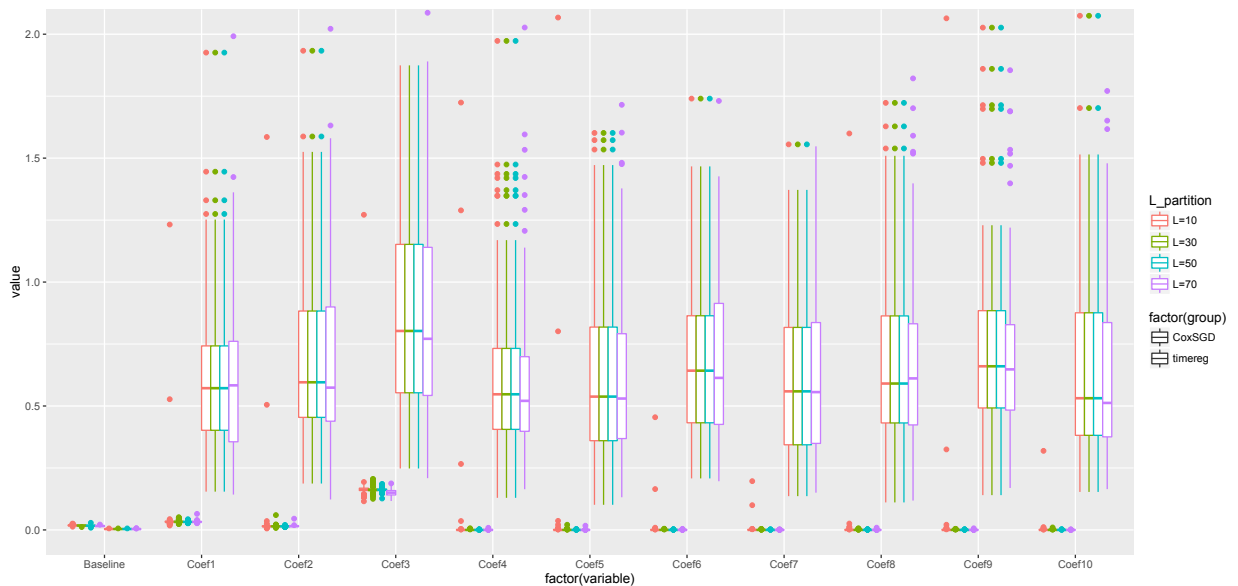
Fig. 4.2 – A boxplots of the MSE_j of estimated regression coefficients over L -partition ( L \in \{10, 30, 50, 70\} ) with CoxSGD and timereg R-package.
