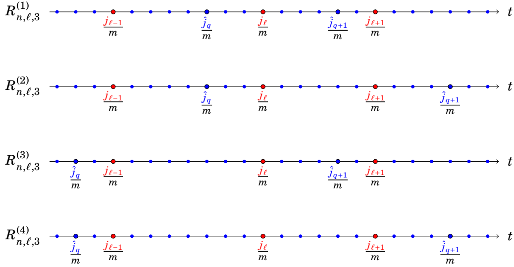
Fig. 2.11 – Illustration of the events R_{n,\ell,3}^{(s)} for s = 1, \dots, 4 .
