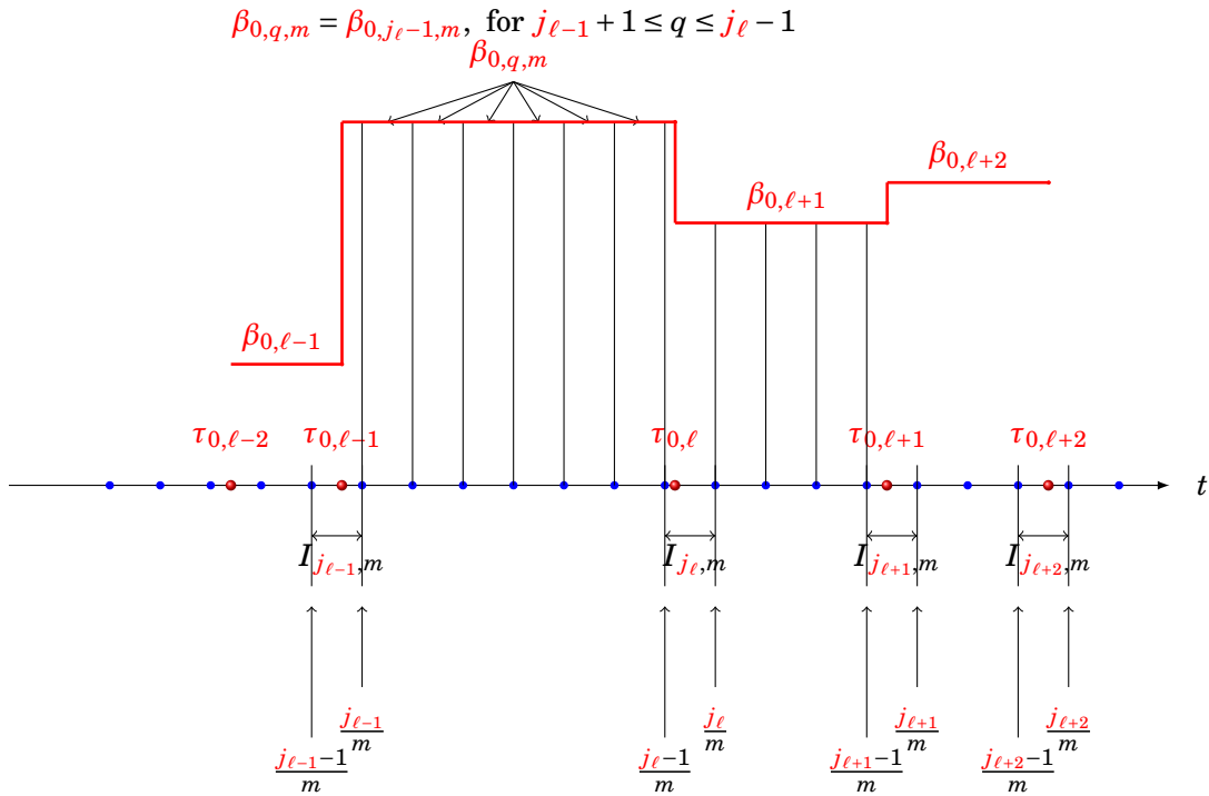
Fig. 2.10 – A zoom of \beta_{0,q,m} , the coefficients of the projection function \lambda_{0,m} in Case I.
