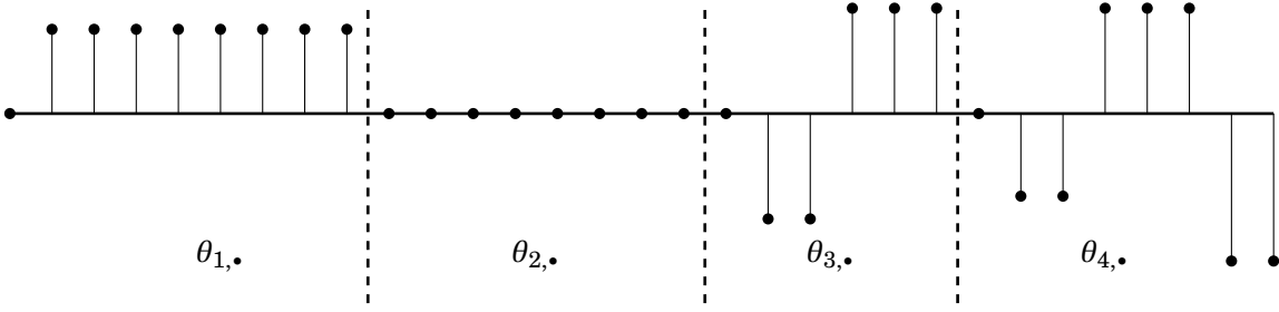
Fig. 1.2 – Illustration de \theta = [\theta_{1,\bullet}^\top, \dots, \theta_{p,\bullet}^\top]^\top avec : p = 4, d_1 = 9, d_2 = 8, d_3 = 6, d_4 = 8 .
