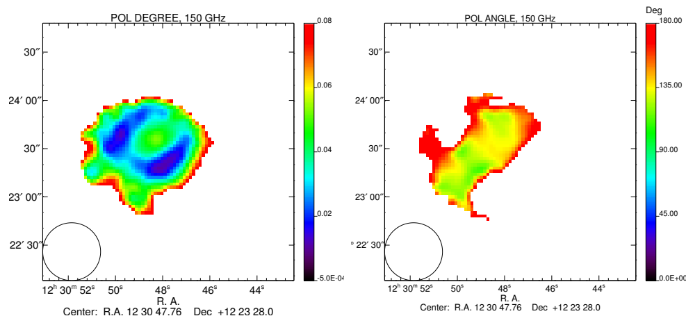
Figure 7.15: Polarisation degree (left) and angle (right) map of M87 in the region where P > 2 \sigma_P . The most polarised regions of the source reaches a value of the polarisation degree of \sim 2\% .
