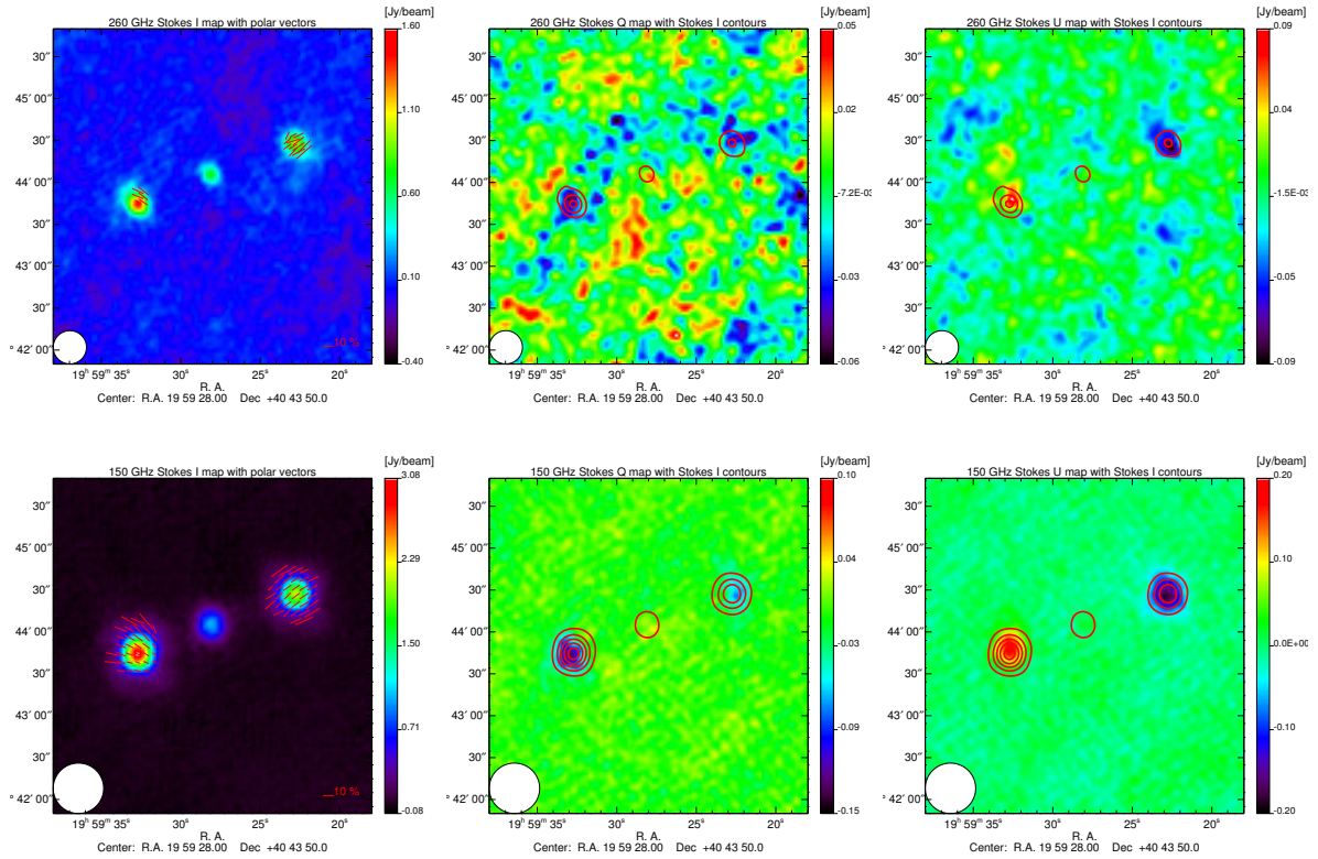
Figure 7.17: Cygnus A leakage corrected Stokes I, Q and U maps at 260 GHz (top) and 150 GHz (bottom). The contours in Q, U represent the intensity map. They start from 0.2 Jy/beam with steps of 0.2 Jy/beam. Polarisation vectors are over-plotted in red on the intensity image when I > 0 and P > 2 \sigma_P .
