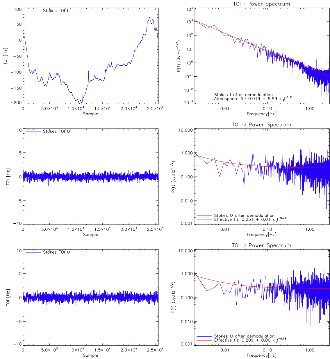
Figure 6.12: From top to bottom “pure” Stokes TOI I, Q, U obtained after the demodulation procedure (left) and corresponding spectrum (right) for a KID of one observation. A bandpass filter [0.01, 2.9] Hz is applied to reject any high frequency noise.
