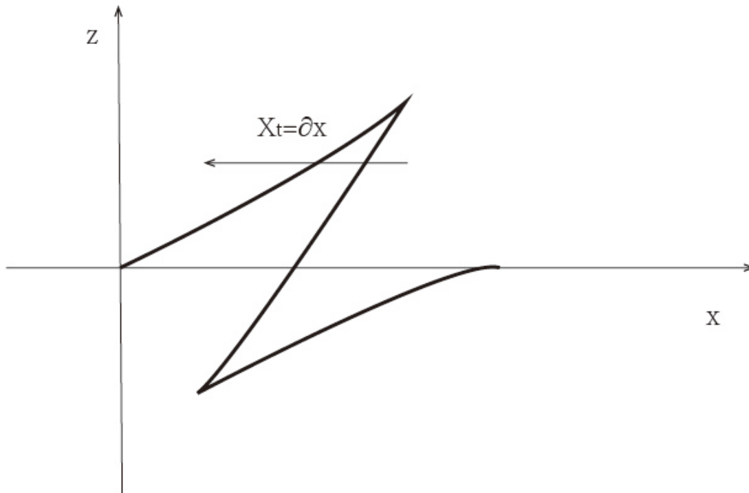
FIGURE 2.1 – Rotation
