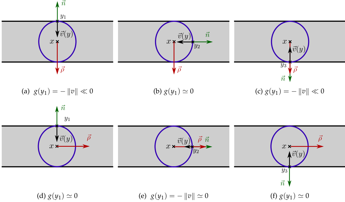
Figure 52: The direction \rho maximizing the total outward flux is the curvilinear structure direction. Each image represents a curvilinear structure and a sphere centered at x , on which the flux can be computed. (a-c) represent the case of a flux computed along a direction \vec{\rho} , which is not the direction of the curvilinear structure; (d-e) represent the case of a flux computed along the curvilinear structure direction. \vec{v}(y) is the image gradient at point y and \|v\| its norm. For y on the edge of the curvilinear structure, \|v\| \gg 0 while everywhere else, \|v\| \simeq 0 . If the flux is computed from these 3 cases, f(x, r, \rho) = \sum_{i=1}^3 (g(y_i)) = \sum_{i=1}^3 (\vec{v}(y_i) \cdot \vec{\rho}) \vec{\rho} \cdot \vec{n} . The direction \rho maximizing the outward flux is the curvilinear structure direction.
