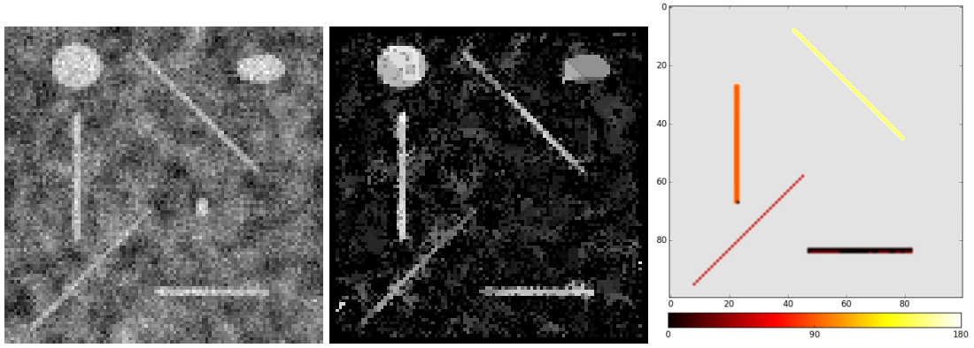
Figure 66: The synthetic initial image (a) and its RORPO intensity feature (b) and RORPO directional feature (c). The directions are encoded with colors, from 0^\circ (black) to 180^\circ (white).
