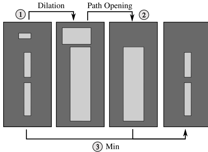
Figure 44: Illustration of the simplified robust path opening. A curvilinear structure is disconnected by a noisy pixel. After dilation this pixel is no longer consider as noise, but belongs to the curvilinear structure , which allows the path opening to preserve the whole curvilinear structure. A minimum operator is finally applied to ensure anti-extensivity.
