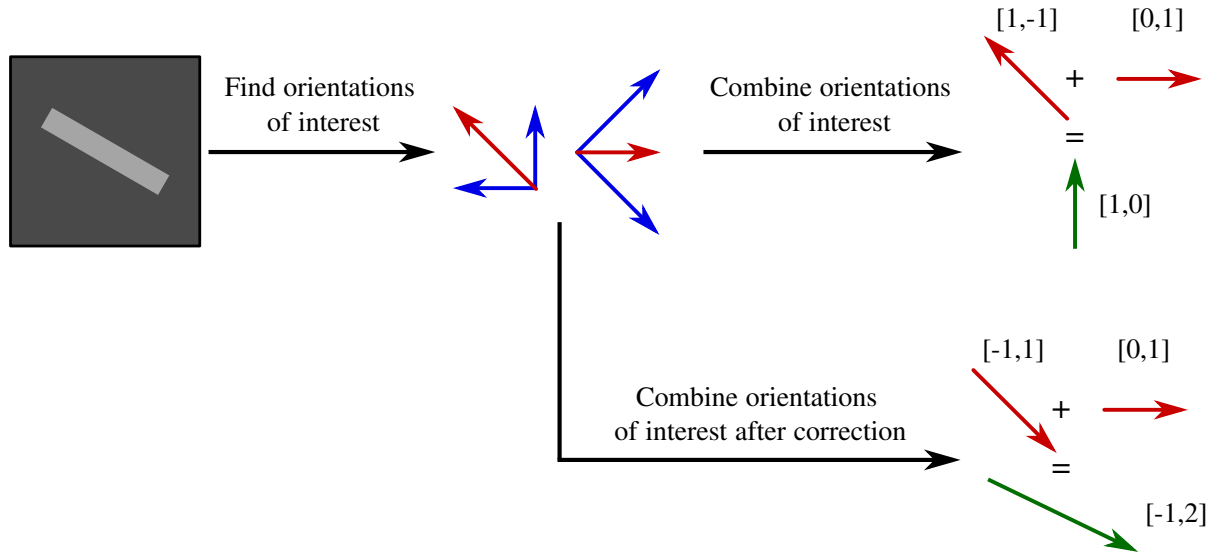
Figure 41: Without correction of the principal vectors, the final curvilinear structure direction is incorrect ( [1, 0] ). We first need to switch one of the principal vectors from [1, -1] to [-1, 1] (both have the same orientation), and sum them to obtain the correct curvilinear structure direction ( [-1, 2] ).
