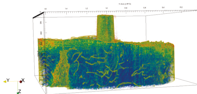
Figure 7: Volume rendering of the micro-pillar (' istb_mp5_25nm_tomo3 '). The box is 51\mu\text{m} (X) by 51\mu\text{m} (Y) by 19.9\mu\text{m} (Z). A lacuna is visible on the bottom left of the base.
