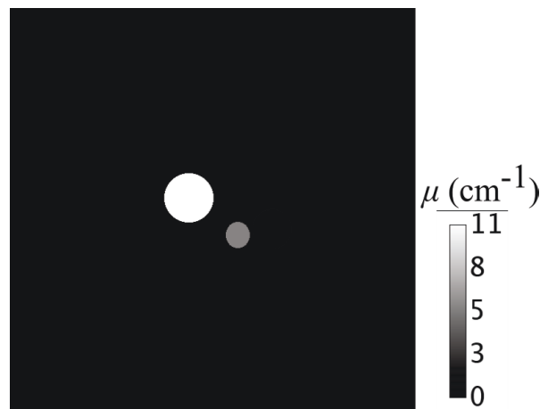
Figure 3: Example of an attenuation slice of the three-wire phantom. Wires, from left to right: Al, Mg and PET, of diameters 250\mu\text{m} , 125\mu\text{m} and 200\mu\text{m} respectively.
