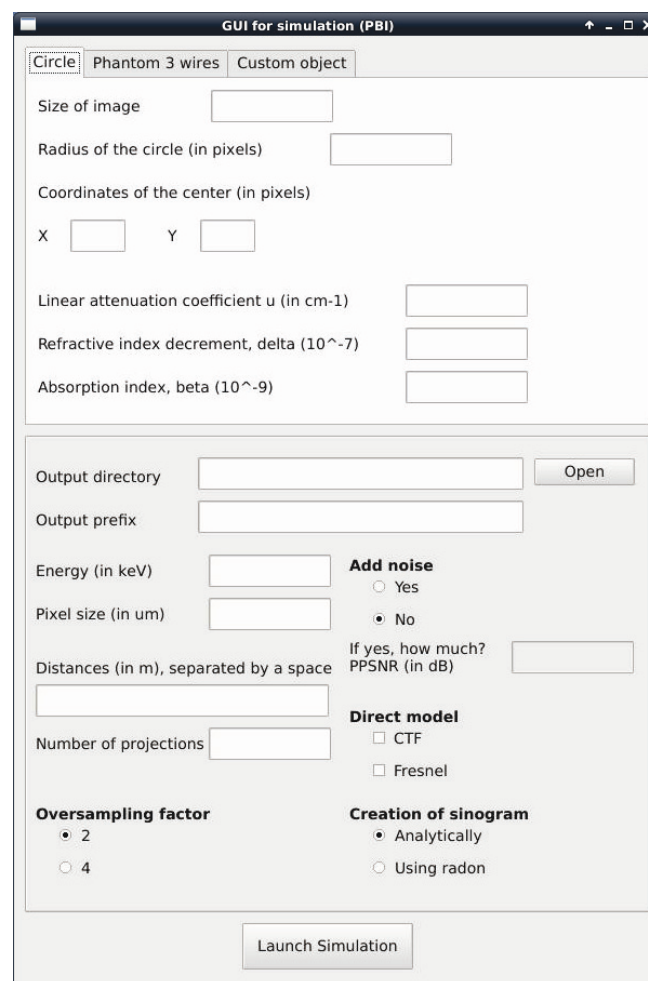
Figure 4: Python interface for data simulation, when the object is a 2D-circle. The upper part (white background) corresponds to the parameter related to the chosen object. The lower part (gray background) refers to the general settings.
