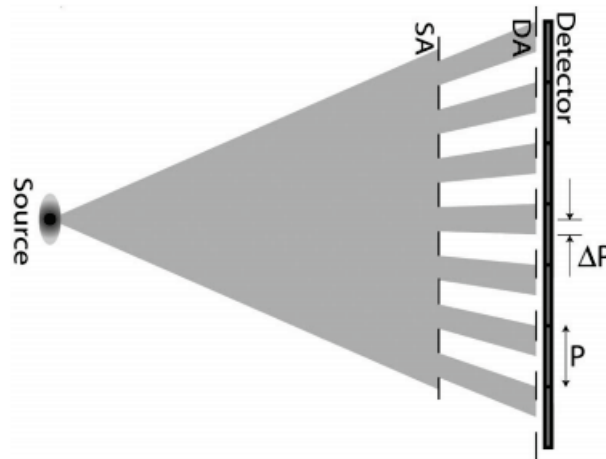
Figure 19: Coded-aperture set-up (from [Olivo, 2011]). The Sample Aperture (SA) mask is placed just upstream to the sample. The Detector Aperture (DA) mask is placed just before the detector. P denotes the detector pixel size, and \Delta P the illuminated fraction of a pixel.
