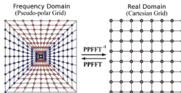
Figure 1: Pseudo-Polar Fast Fourier Transform bridges the gap between real domain and frequency domain. Image from (Miao et al. , 2005).
