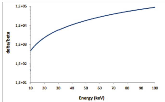
Figure 14: \delta_n/\beta ratio of soft tissues, as a function of the energy (in the range of hard X-rays).
