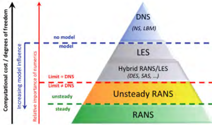
Figure 3.2: Classification of unsteady approaches according to levels of modeling and readiness, from Larauie [137], adapted from Sagaut et al. [182]
