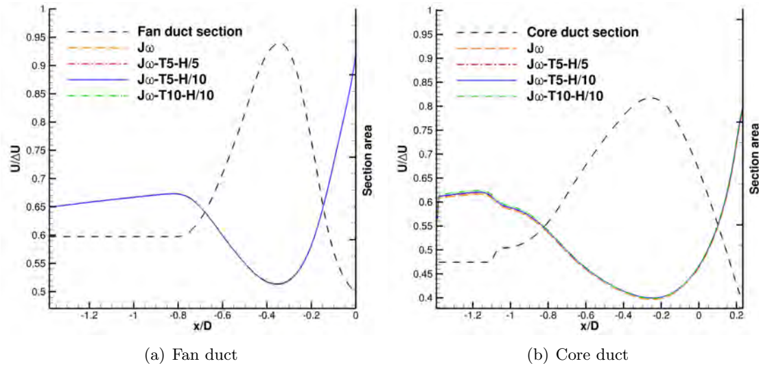
Figure 5.3: Evolution of the axial velocity U/\Delta U along the fan and core ducts
