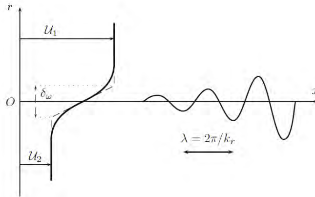
Figure 2.2: Illustration of vorticity thickness in the case of an hyperbolic tangent profile and of the instability wave growth, from Bailly & Comte-Bellot (2015)[16]
