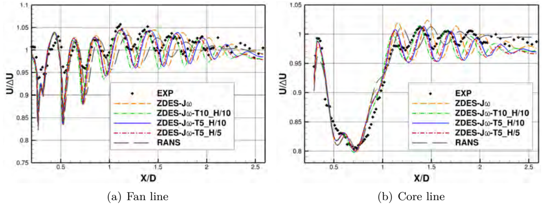
Figure 5.11: Mean field of axial velocity : Fan and Core lines
