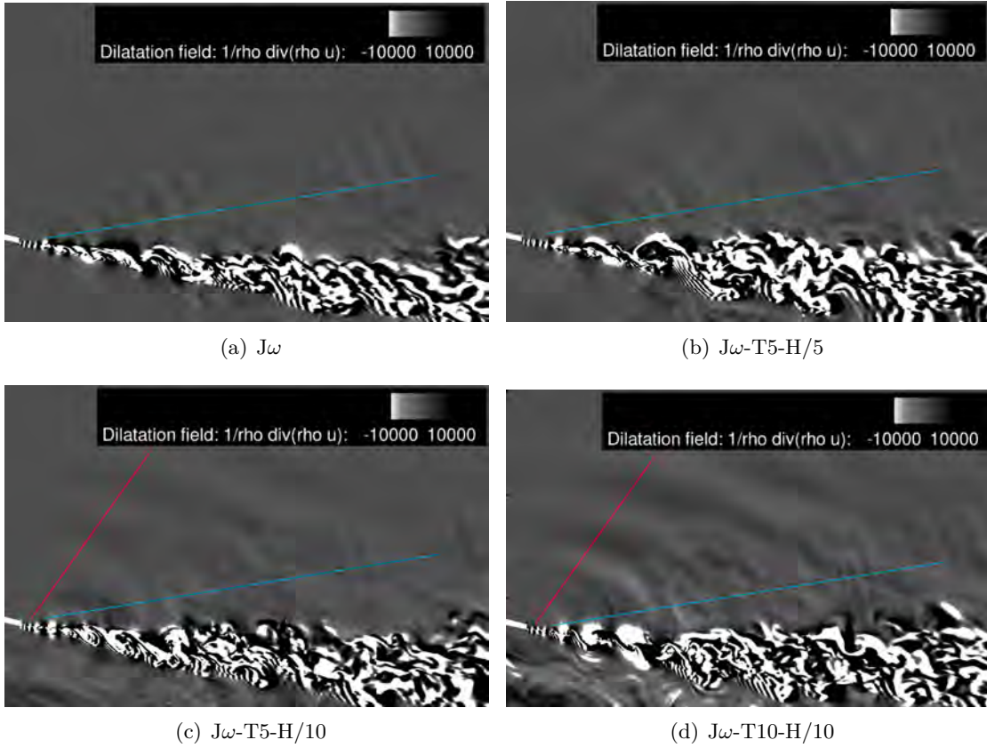
Figure 5.21: Instantaneous fields : dilatation field. The red and blue lines are used to identify the different acoustic waves emanating from the nozzle trailing edge area.
