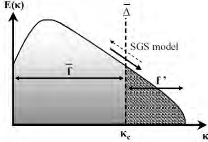
Figure 3.3: LES turbulent field decomposition (sharp cutoff filter), adapted from Sagaut et al. [182]
