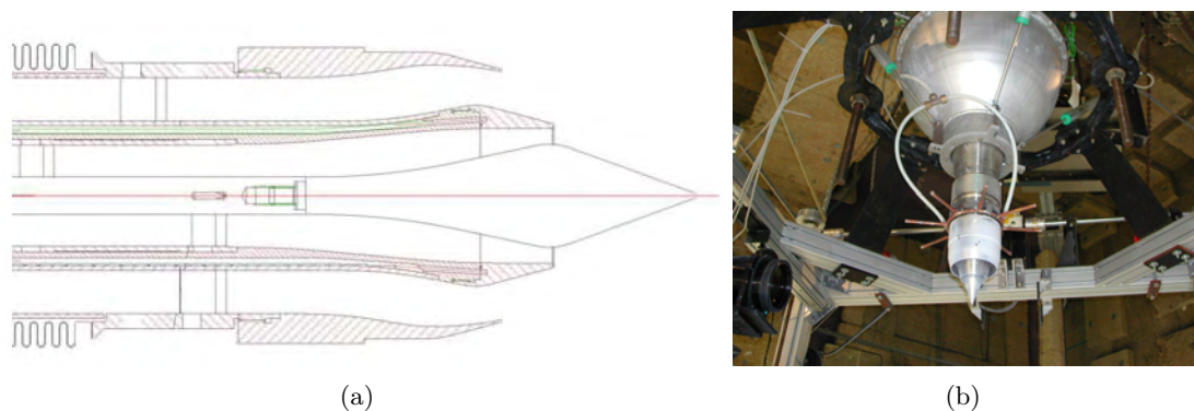
Figure 3.7: Martel test rig: (a) geometry of the coaxial nozzle, (b) JEDI nozzle installed on the MARTEL Test Rig
