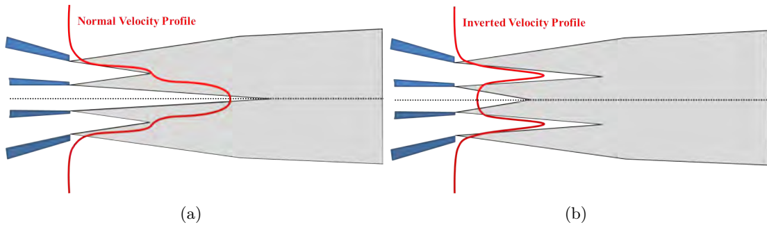
Figure 2.16: Two kinds of velocity profiles in coaxial configurations: (a) Normal velocity profile (NVP), (b) Inverted Velocity Profile (IVP)
