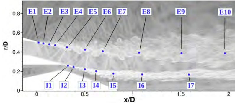
Figure 4.12: Probes location
