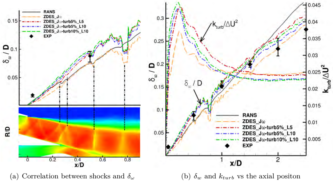
Figure 5.18: External mixing layer development: (a) Effect of the shock cell pattern on the vorticity thickness, (b) vorticity thickness \delta_\omega and turbulent kinetic energy k_{turb} evolution along the mixing layer.
