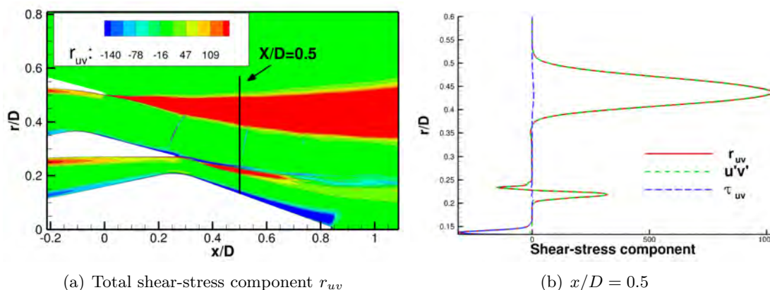
Figure B.1: Shear-stress component estimation: (a) contour of the total estimation, (b) breakdown of the shear-stress component at x/D = 0.5
