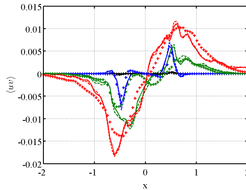
Figure 6.3.9: Reynolds tensor investigation.
