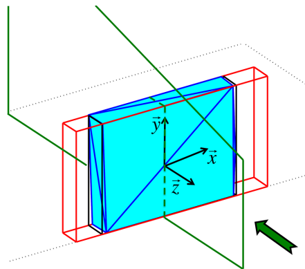
Figure 5.2.4: 2D-PIV measurement plane ( yz plane) and tomographic volume.
