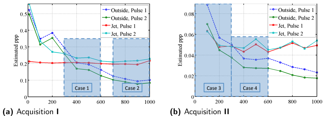
Figure 6.3.1: 3D-PIV ppp estimation for Acquisition I and II . The 2 pulses in the figure's legend refer to the 2 pulses of the 2D-PIV laser. The pulse 1 was more powerful than pulse 2, hence detecting more particles
