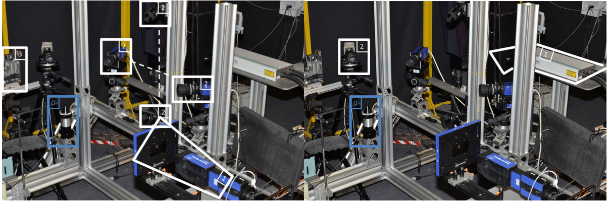
3D-PIV Setup
