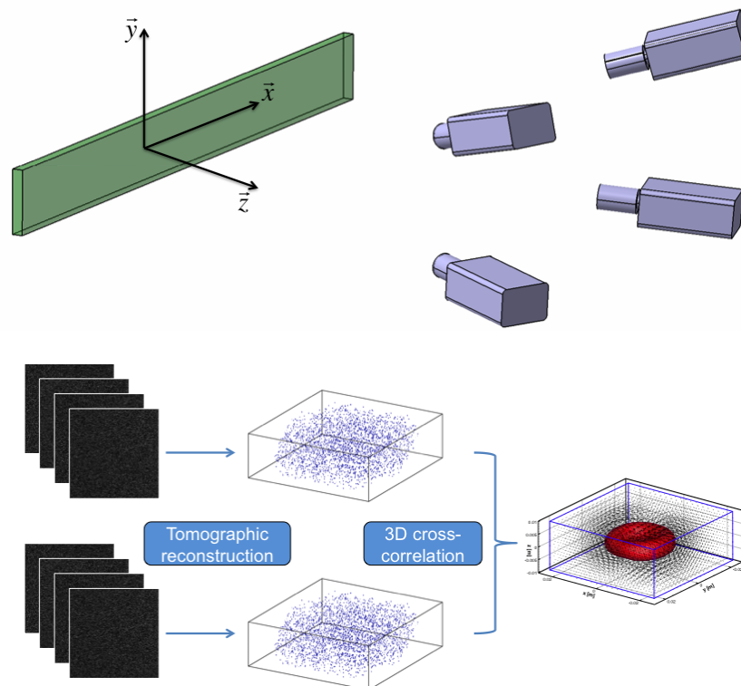
Figure 1.3.1: Simplified experimental setup (top) and main working principles of tomographic PIV (down).
