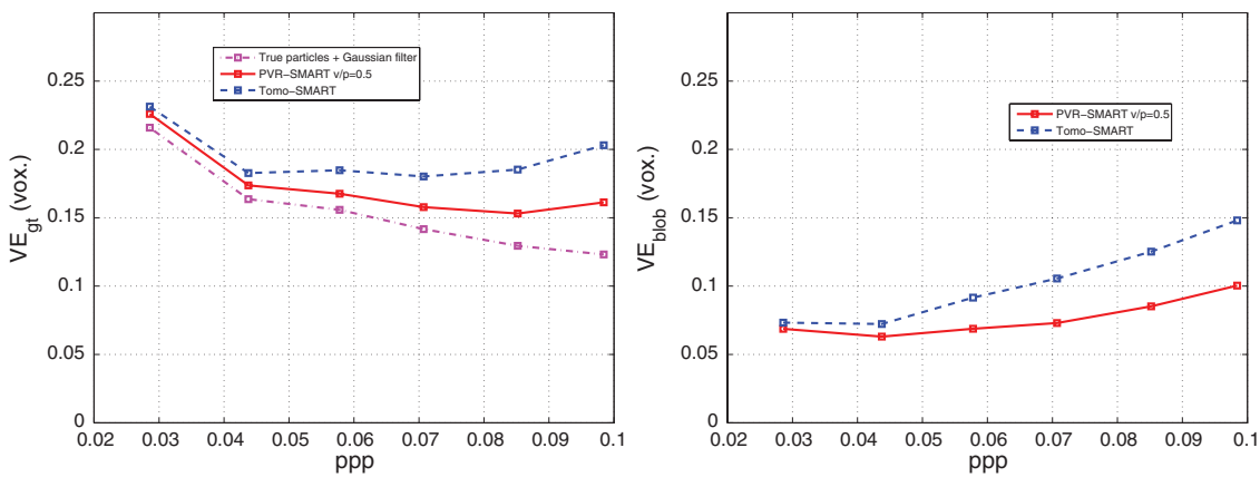
Figure 15. Comparison between conventional tomographic reconstruction and the proposed PVR approach, using the SMART algorithm, \sigma_{psf}=0.6 , for varying N_{ppp} . I/U=0.47 . Left: displacement error w.r.t. ground truth \nu^* . Right: displacement error w.r.t. \nu^o .
