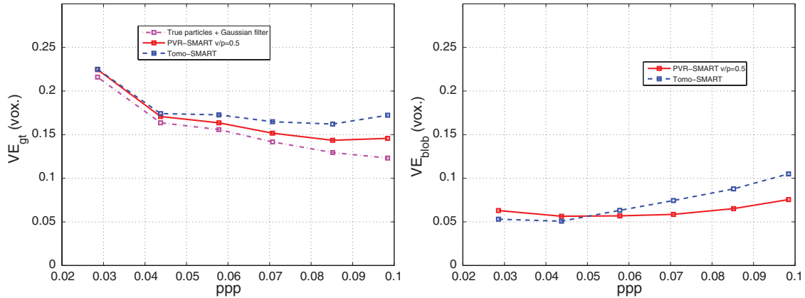
Figure 14. Comparison conventional tomographic reconstruction and the proposed PVR approach, using the SMART algorithm, \sigma_{psf}=0.6 , for varying N_{ppp} . I/U=1 . Left: displacement error w.r.t. ground truth \nu^* . Right: displacement error w.r.t. \nu^o .
