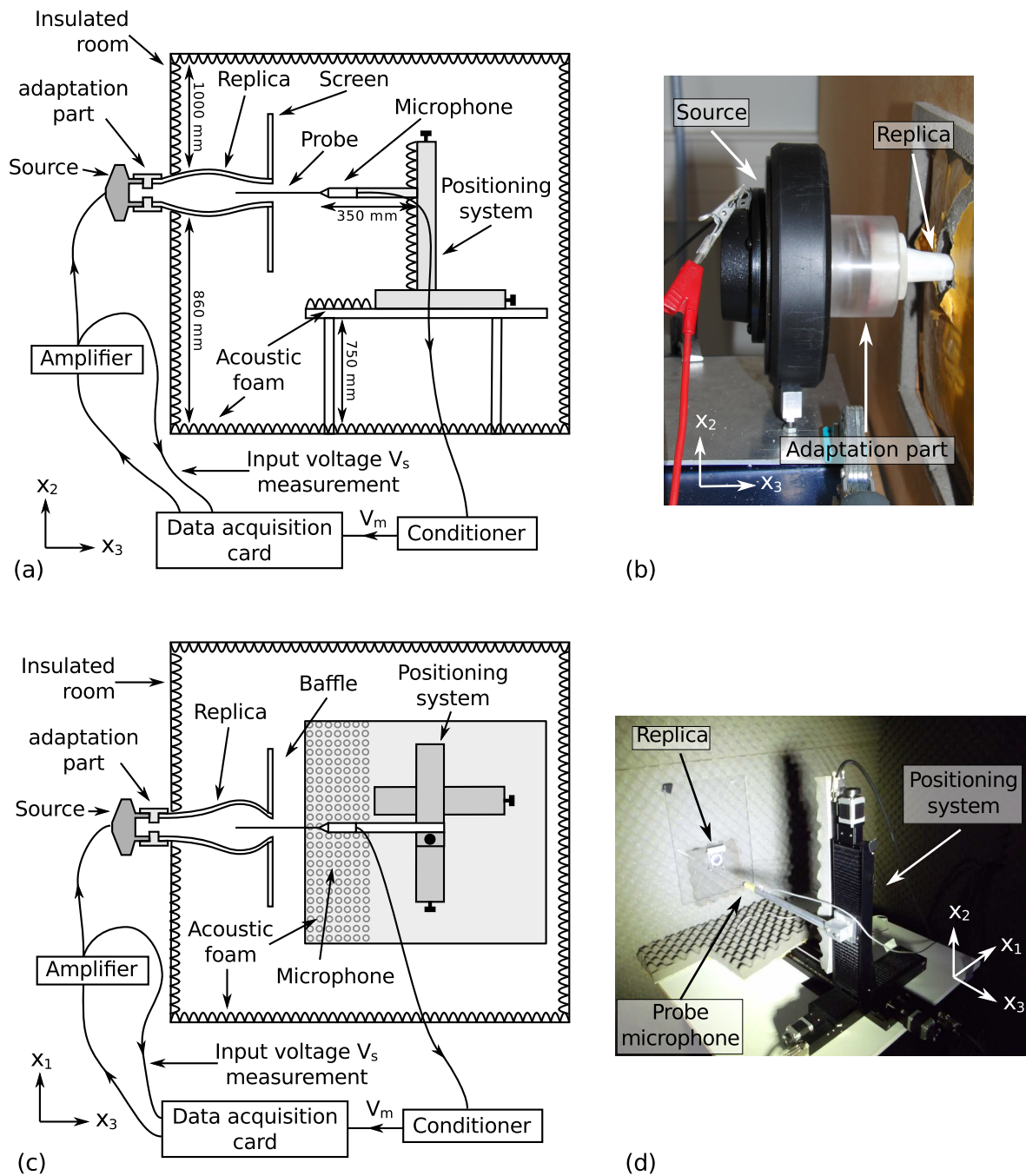
Figure 3.4: Experimental setup (a) schematic diagram in the plane (x_2, x_3) (b) sound source (Eminence PSD:2002S-8 in this case) (c) schematic diagram in the plane (x_1, x_3) (d) positioning system inside the insulated room
