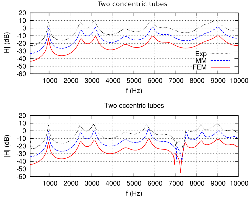
Figure 4.3: Examples of pressure-pressure transfer functions between two points inside two vowel [a] vocal tract replicas made of two cylindrical tubes with (top) concentric (2CC[a]) and (bottom) eccentric junctions (2CE[a]). The Exp and FEM data has respectively been increased and decreased by 10 dB and -10 dB with respect to the MM for visualization purposes. (Exp: experimental data, MM: multimodal method, FEM: finite element method).
