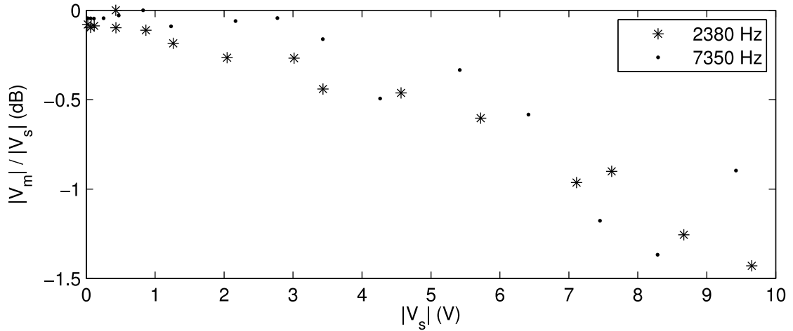
Figure 3.6: Ratio of the amplitude |V_m| of the microphone output voltage over the amplitude |V_s| of the sound source input voltage as a function of |V_s| obtained with two sinusoidal input signals of frequency 2380 Hz and 7350 Hz. The data have been normalized by the maximum.
