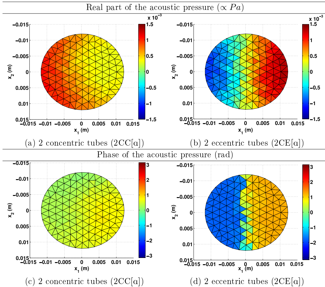
Figure 4.6: Real part and phase of the acoustic pressure measured in the plane (x_1, x_2) perpendicularly to the propagation axis x_3 , 4.5 cm after the junction inside larger part of the two tube replicas of the vowel [a] having either a concentric (2CC[a]) or an eccentric (2CE[a]) junction. The real part is proportional to Pa to the sensitivity of the microphone and the phase is computed as the difference between the phase of the microphone and the phase of the sound source input signal.
