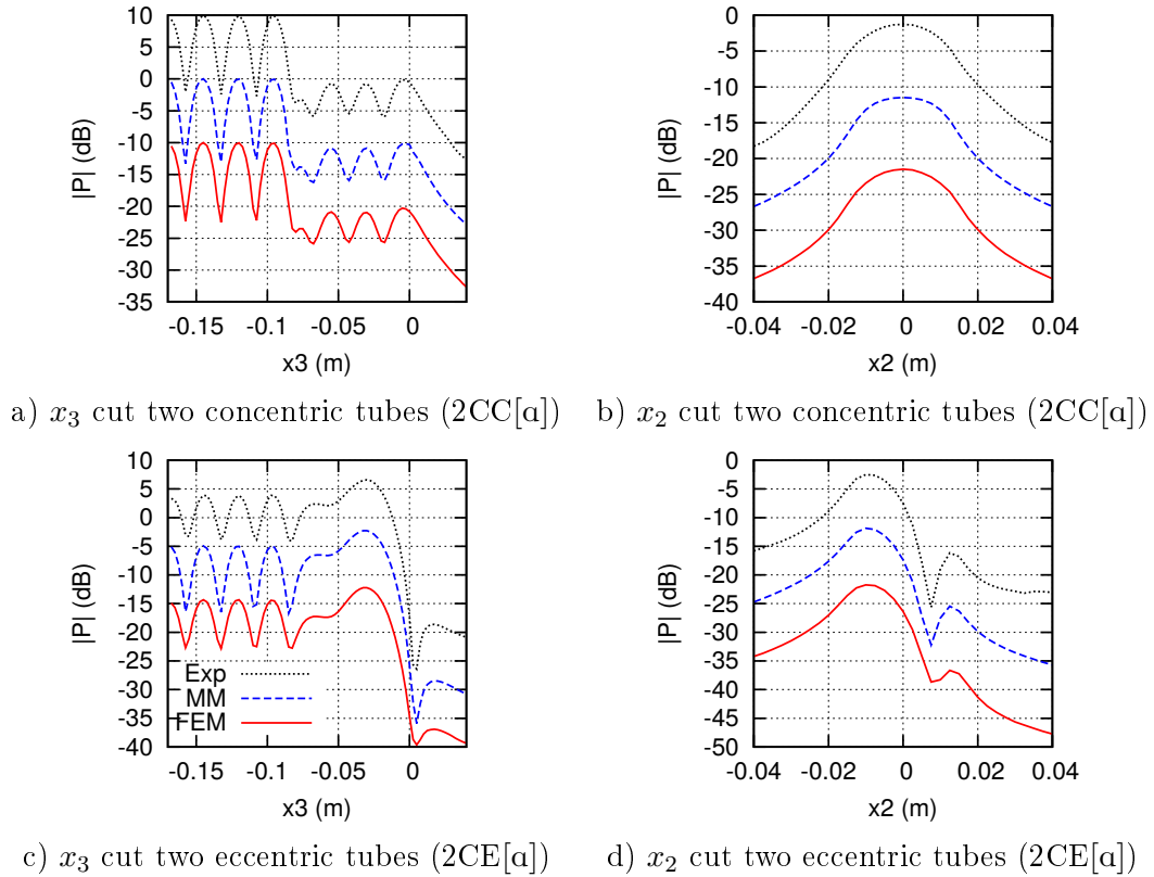
Figure 4.5: Cuts of the pressure maps in Fig. 4.4 along the central axis x_3 (left column) and a perpendicular x_2 axis located just in front of the open end (right column) measured and simulated on two vowel [a] vocal tract replicas made of two cylindrical tubes with either concentric or eccentric junctions (2CC[a] and 2CE[a]). A 10 dB shift has been applied between the maxima of the three curves for visualization purposes. (Exp: experimental data, MM: multimodal method, FEM: finite element method).
