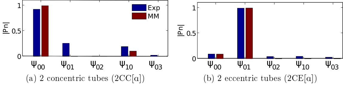
Figure 4.7: Modale amplitudes |P_n| of the pressure measured and simulated on a plane perpendicular to the propagation axis of two tube approximations of the vowel [a] with either concentric (2CC[a]) or eccentric (2CE[a]) junctions.
