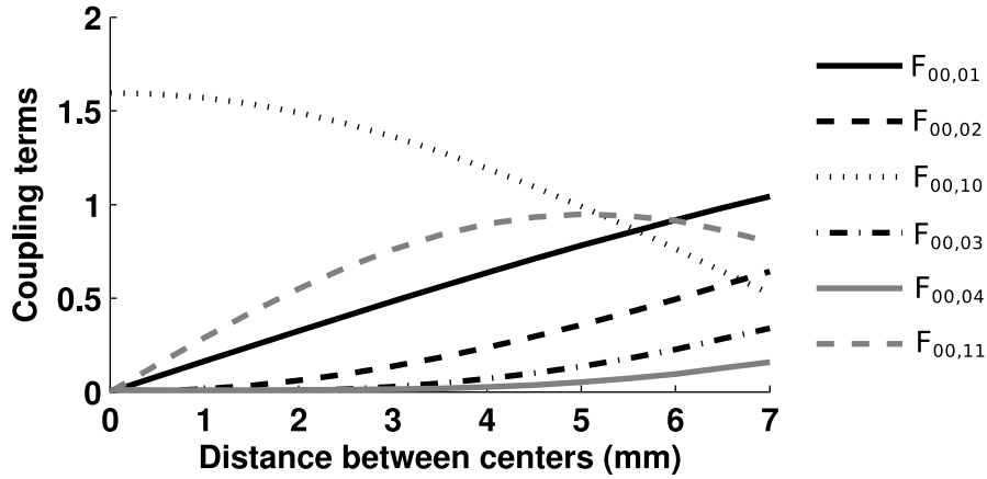
Figure 2.13: Coupling terms of the projection matrix \mathbf{F} of Eq. (2.36) between the plane mode \psi_{00} and the HOM whose cut-on frequency is below 20 kHz ( \psi_{01} , \psi_{02} , \psi_{10} , \psi_{03} , \psi_{04} and \psi_{11} ) for a junction between two cylindrical sections of diameter 14.5 mm and 29.5 mm with a distance between their centers varying from 0 to 7 mm. The amplitude of the terms F_{00,01} , F_{00,02} , F_{00,03} , F_{00,04} and F_{00,11} , correspond to the combination of the amplitude of both degenerated HOM \psi_{mn1} and \psi_{mn2} : F_{00,mn} = \sqrt{F_{00,mn1}^2 + F_{00,mn2}^2} .
