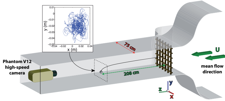
Figure 6.1: The measurement plane is located 2.08m downstream the grid, in a region where the turbulence is fully developed, homogeneous and isotropic.
