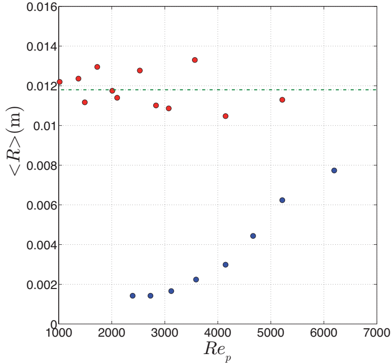
Figure 6.16: Mean value for the radial component of the position for the laminar case (blue) and the turbulent case (red), where the green line represents the average of these points ( R = 1.18 cm).
