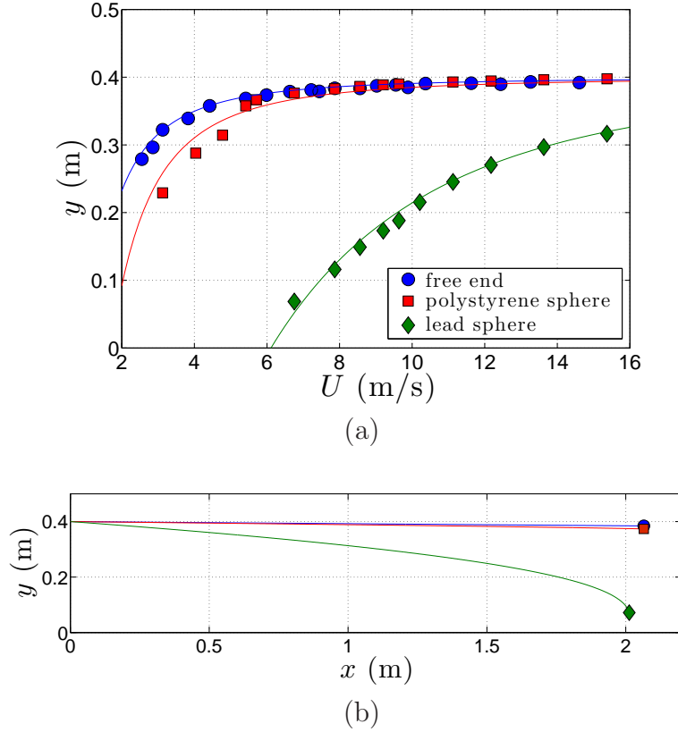
Figure 5.4: (a) Mean height for the wire cable tip measured for the three configurations of towed object. The solid lines correspond to the best simultaneous adjustment of the drag coefficients C_D , C_N and C_T acting on the cable in equations (5.1). (b) Global shape of the cable calculated from the resolution of equations 5.1 for a towing velocity of U = 7 m/s.
