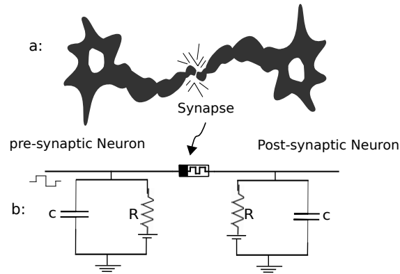
Figure 6.1: a) Schematic of two simple biological neurons connected with synapse, b) Leaky Integrated & Fire model of neuron connected with artificial synapse (memristor)
