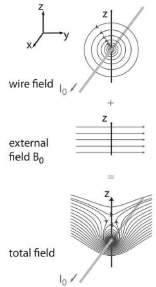
Figure 49 Magnetic trap produced by a single carrying wire and a transverse bias field. Adapted from [243]
