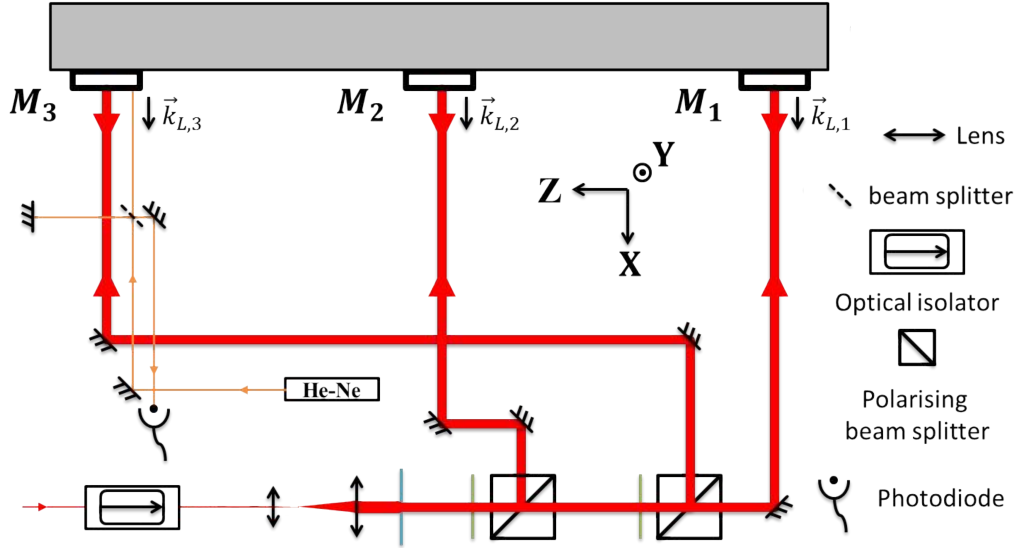
Figure 7: Schematic representation of the optical and mechanical setup used to produce three Bragg lattices. The optical bench is represented from above and the atom beam travels from the right to the left.
