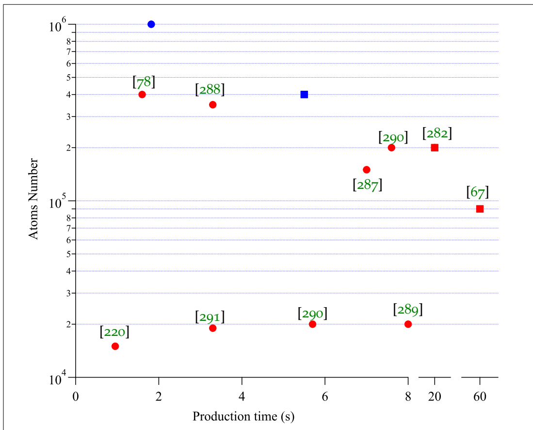
Figure 60: Demonstrated high production rates ( \leq 8 s, circles) of ^{87}\text{Rb} BEC sources, adapted from [78]. All dual isotopes sources ^{85}\text{Rb}/^{87}\text{Rb} are also represented (squares). The red points correspond to published experiments (notice the temporal axis break for dual experiments) and the blue points correspond to the characteristics inferred from our simulations. Our dual evaporation is calculated to perform much faster than the two published experiments [67], [282] thanks to the fast loading rate and the tight initial magnetic trap.
