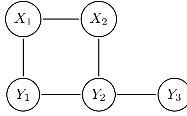
Fig. 4.6. A DN of the joint distribution p(\mathbf{x}, \mathbf{y}) , whose local distributions are p(x_1|x_2, y_1) , p(x_2|x_1, y_2) , p(y_1|x_1, y_2) , p(y_2|x_2, y_1, y_3) , and p(y_3|y_2) .
