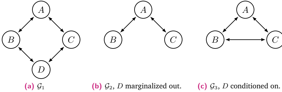
Fig. 2.15. Three BGs \mathcal{G}_1, \mathcal{G}_2, \mathcal{G}_3 such that I(\mathcal{G}_2) = I(\mathcal{G}_1)^\emptyset_D and I(\mathcal{G}_3) = I(\mathcal{G}_1)^D_\emptyset .
