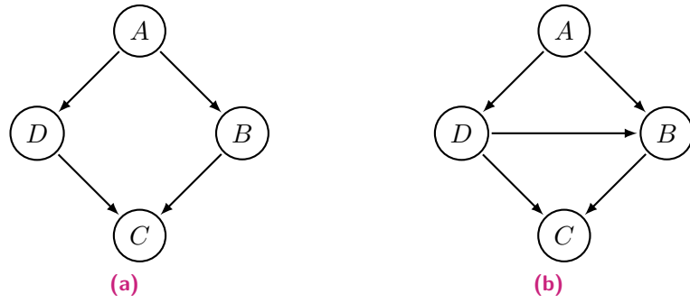
Fig. 2.4. Two directed acyclic graphs (DAGs).
