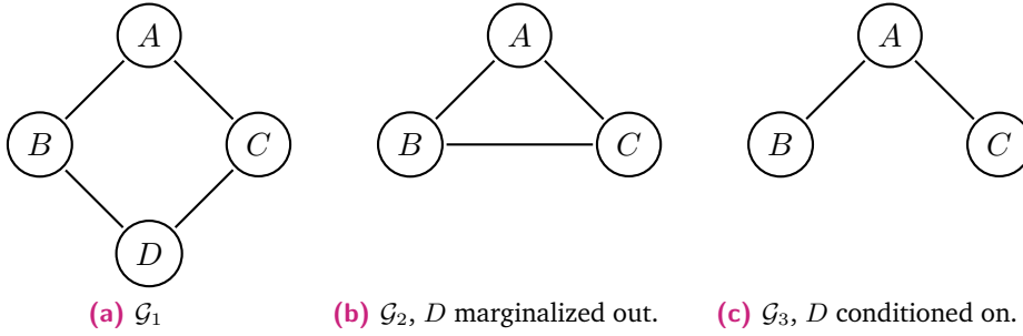
Fig. 2.14. Three UGs \mathcal{G}_1, \mathcal{G}_2, \mathcal{G}_3 such that I(\mathcal{G}_2) = I(\mathcal{G}_1)^\emptyset_D and I(\mathcal{G}_3) = I(\mathcal{G}_1)^D_\emptyset .
