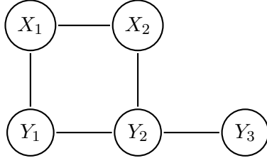
Fig. 4.10. A CRF over \mathbf{Y} , which encode the independence relation \{Y_1\} \perp\!\!\!\perp \{Y_3\} \mid \{Y_2\} \cup \mathbf{X} .
