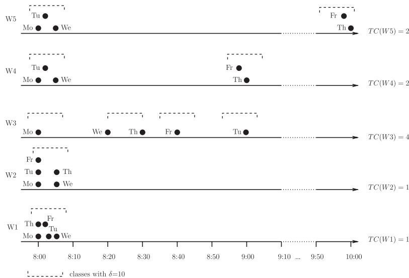
FIG. 2. Time-class consistency.
