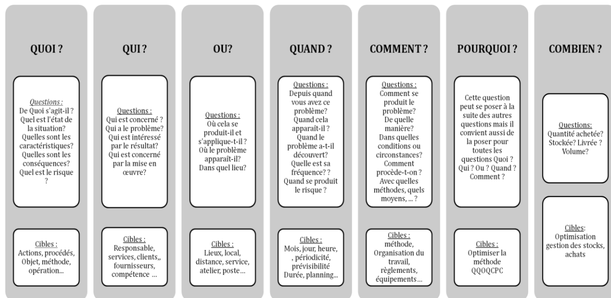
Figure 80: Méthode QQQQPC
