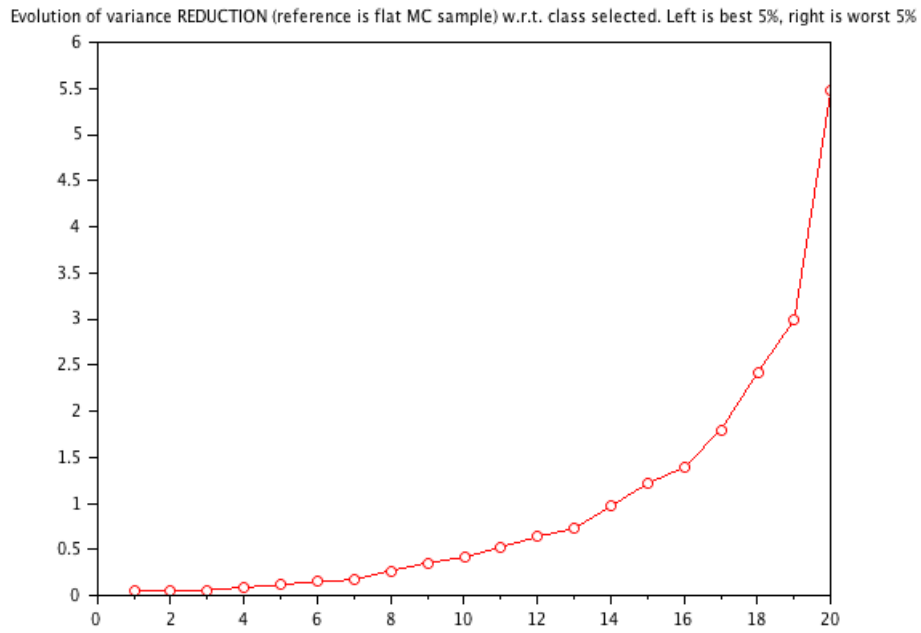
Figure 4.2 – Variance ratio V_{SQS\ 1}/V_{MC} for the 20 groups of realizations (sorted according to their SQS 1 error)
