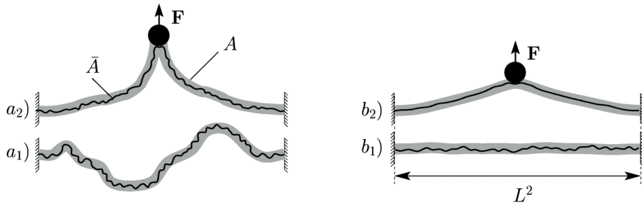
Figure 3.3: Membranes with a microscopic area \bar{A} and optically visible area A , attached to solid frame of surface S = L^2 . A floppy membrane has large fluctuations that are optically visible (a1). By pulling sufficiently on the membrane (a2), one can hinder optically visible fluctuations, without suppressing fluctuations of lower length scales. Similarly an initially "flat" membrane (b1) has a small microscopic excess area and can be further extended (b2) by a small perturbation. (Adapted from [Fournier 2001])
