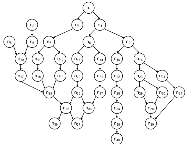
Fig. 2. Precedence graph of random 2 algorithm.
