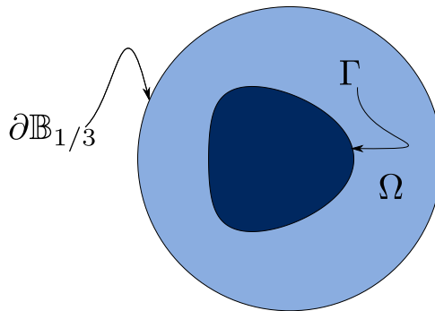
Figure 5.1: Illustration of the geometry
