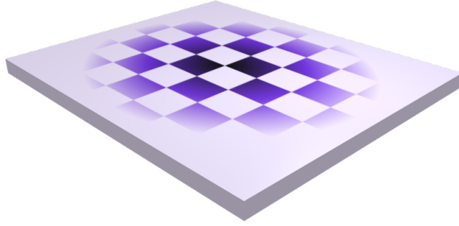
Figure 1.19: The plate for patching solution
