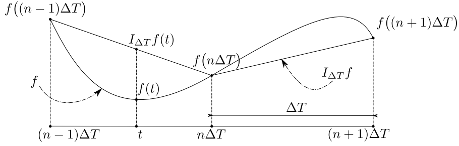
Figure 5.5: Illustration of I_{\Delta T}
