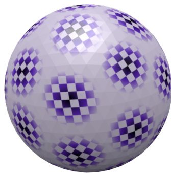
Figure 1.22: The \psi_{\Gamma} - \delta - periodicity for soccer ball
