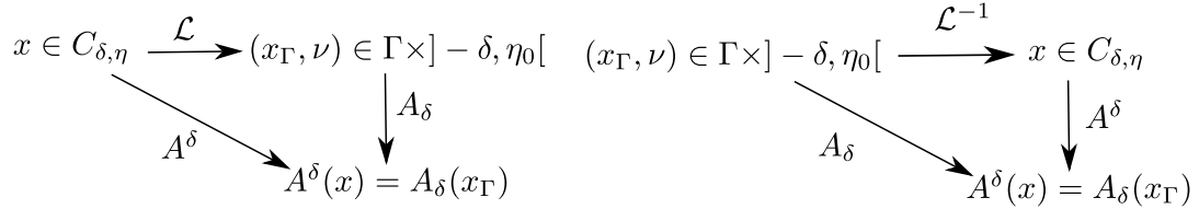
Figure 1.27: The maps A^\delta and A_\delta
