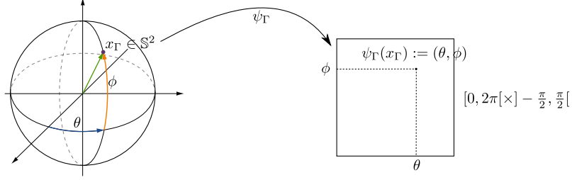
Figure 1.6: the sphere
