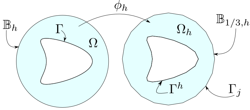
Figure 5.3: Illustration of the domain \Omega_h and the map \phi_h
