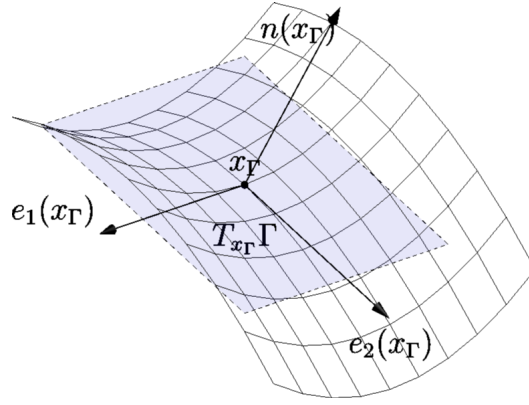
Figure 1.16: Illustration of the space T_{x_\Gamma} \Gamma
