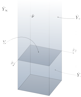
Figure 4.2: Illustration the of infinite strip
