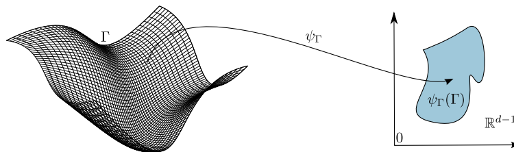
Figure 1.4: The application \psi_\Gamma
