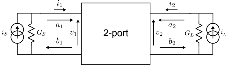
Figure 2.2 The two-port representation of the filter excited by a current source.
