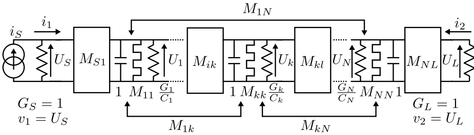
Figure 2.13 Equivalent lumped-element lowpass network of the microwave filter that is represented by the matrix \mathbf{A}
