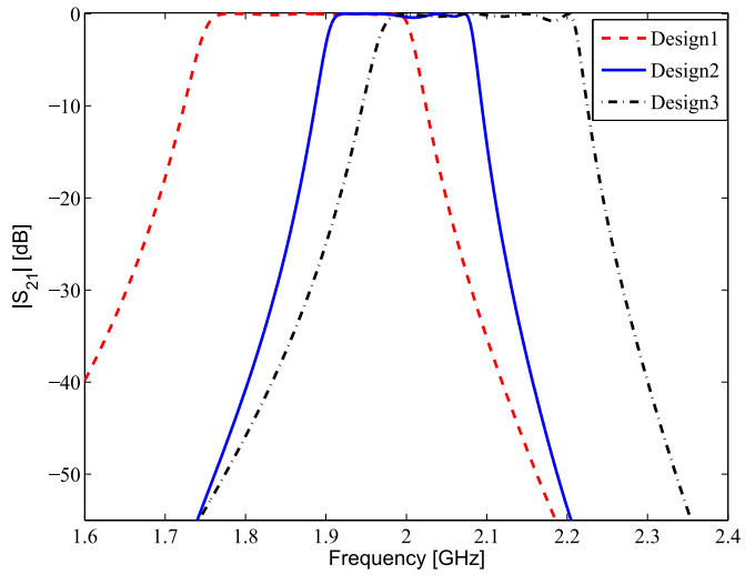
(b) |S_{21}| for the different initial designs.
