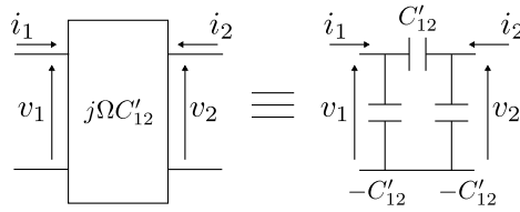
Figure 2.9 Equivalent circuit of mutual capacitive coupling C'_{12} .
