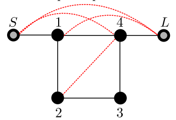
(b) Coupling graph of the extracted arrow form M_{arr}^0 .
