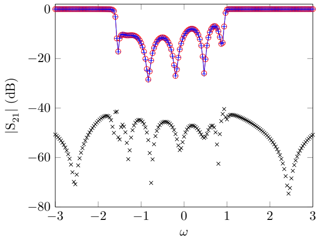
(a) Bode plot for |S_{C11}| ( -o ), |S_{Rat11}| ( -+ ) and the approximation error ( x ).
