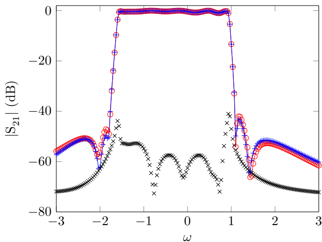
(b) Magnitude of |S_{C21}| ( -o ), |S_{Rat21}| ( -+ ) and the approximation error ( x ).
