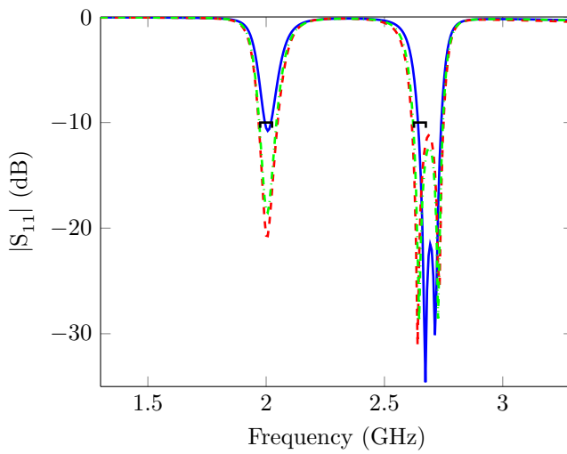
(a) |S_{11}| for the initial design (—), optimized design evaluated using the macromodel (---), EM-simulation (-.-) and specifications (—).
