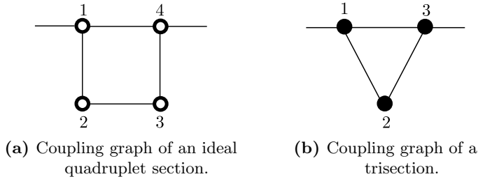
Figure 5.1 Coupling graph of an (ideal) quadruplet and of a trisection.
