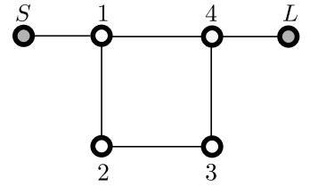
(a) Coupling graph of the ideal quadruplet filter.
