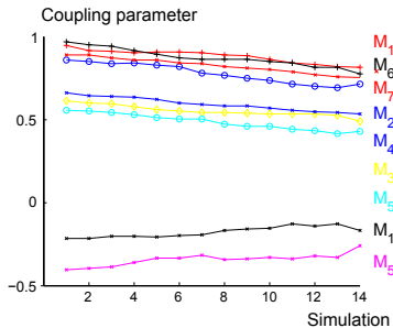
Fig. 6: The extracted inter-resonator couplings for each simulation.
