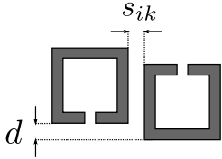
Fig. 3: Top-view of 2 coupled resonators, where s_{ik} is the spacing between them and d is a possible offset.
