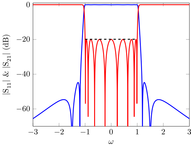
Figure 2.6 Magnitude of S_{11} (—) and S_{21} (—) of (8-4) symmetric pseudo-elliptic filter in the lowpass domain, with RL = 20 (---) dB and finite transmission zeros at \omega = \pm 1.2 and \omega = \pm 1.5 .
