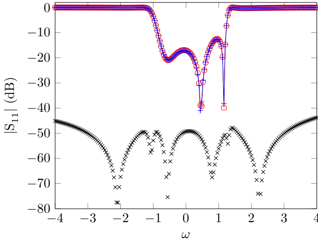
(a) Magnitude of |S_{C11}| ( -o ), |S_{Rat11}| ( -+ ) and the approximation error ( x ).
