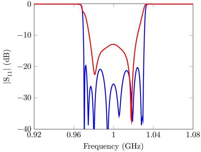
(a) |S_{11}| for the ideal coupling matrix with extra couplings added (—), the final loss-less design (—) and the ideal response (- - -)
