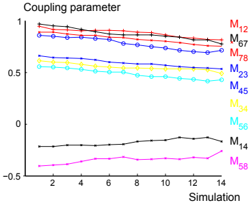
Fig. 6: The extracted inter-resonator couplings for each simulation.
