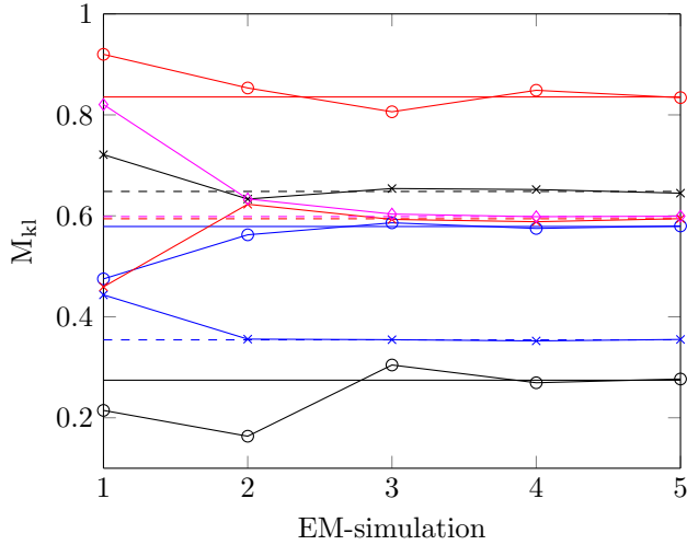
(a) Evolution of the inter-resonator couplings during the tuning process.
