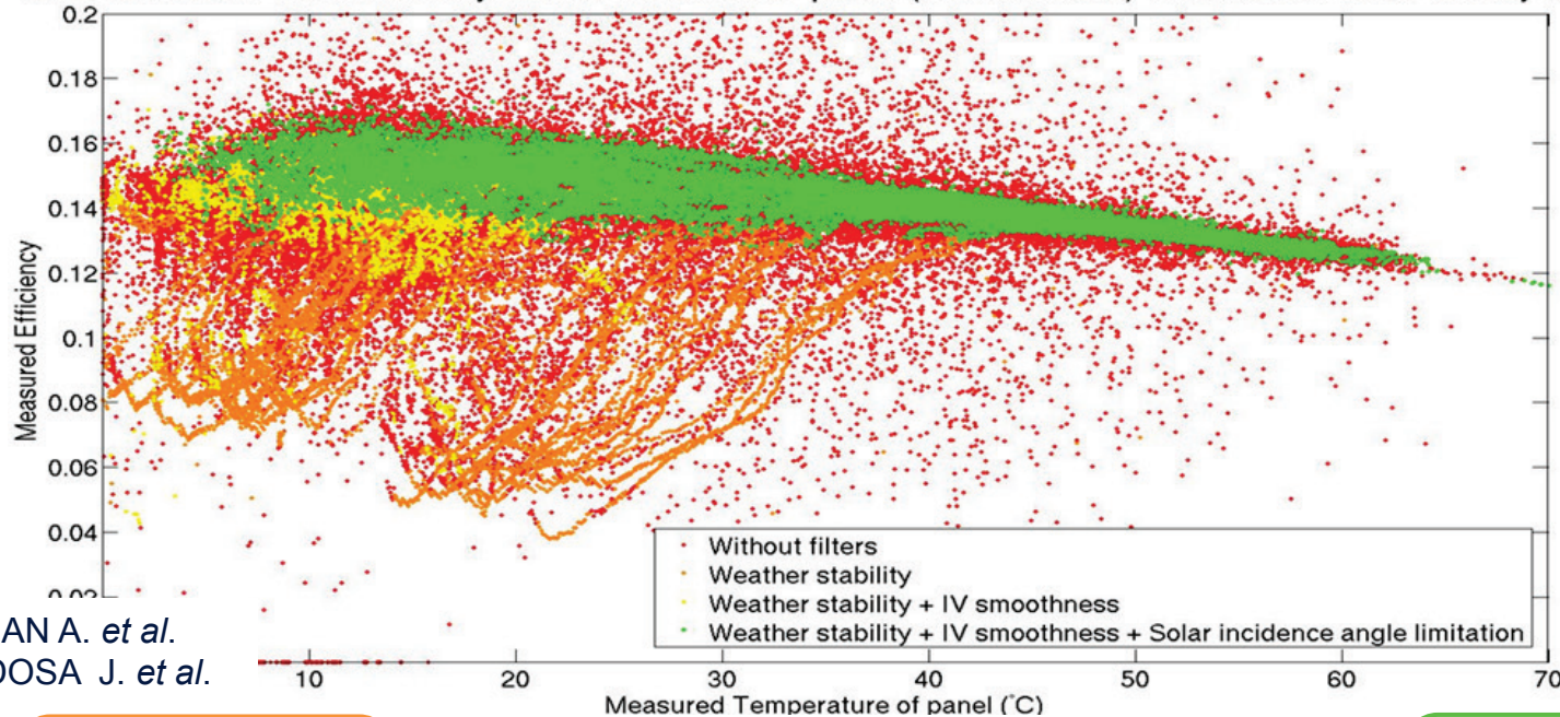
Data extraction from monocrystalline silicon solar panel (FranceWatts) from March 2015 to May 2015
