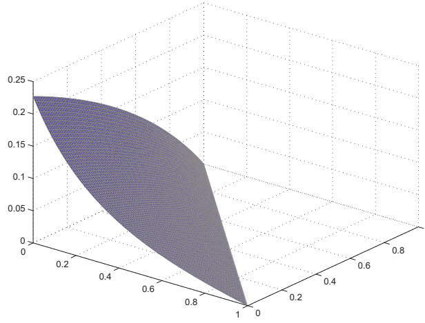
Figure 3.2. Graph of the function \mu_3(\cdot) for k_2 = 1 and the parameter values in table 3.5.
